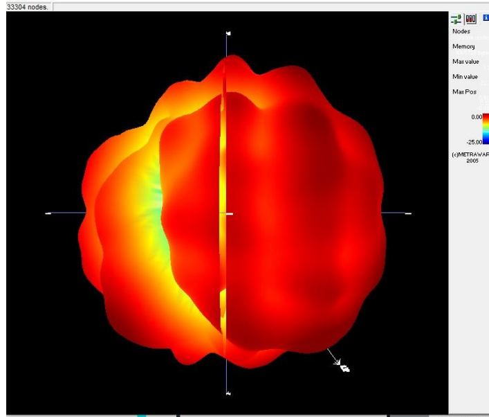
Max Antenna 3D Radiation Pattern 5150-5250 MHz
