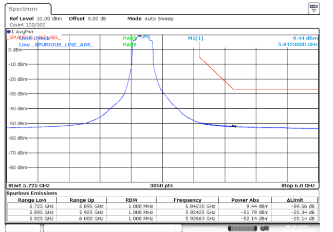
BE-NR-HIGH, MIMO-B, 802.11n20-HT8, Ch169
