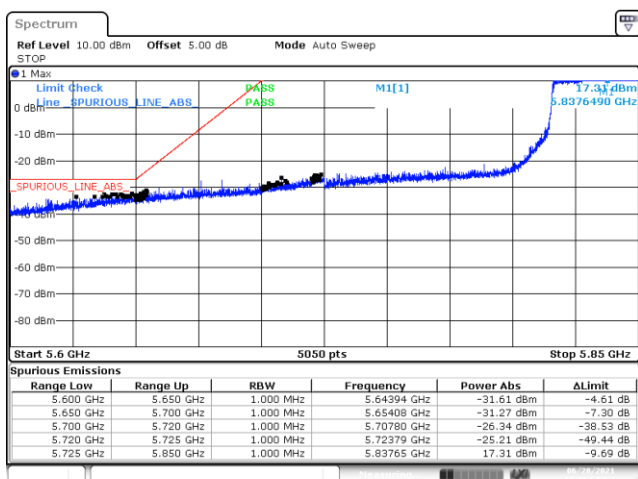
BE-NR-LOW, MIMO-B, 802.11ax80-HE0, Ch171
