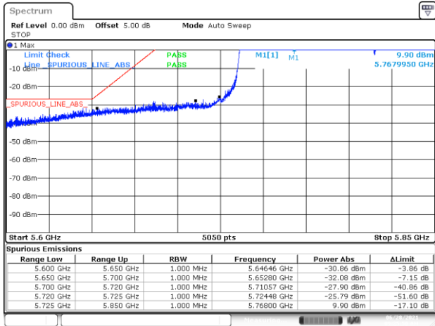
Date: 28.JUN.2021 09:25:50 BE-NR-LOW, MIMO-B, 802.11ax160-HE0, Ch163
