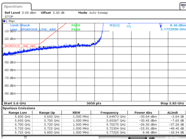
Date: 28.JUN.2021 08:03:39 BE-NR-LOW, MIMO-B, 802.11ac160-VHT0, Ch163
