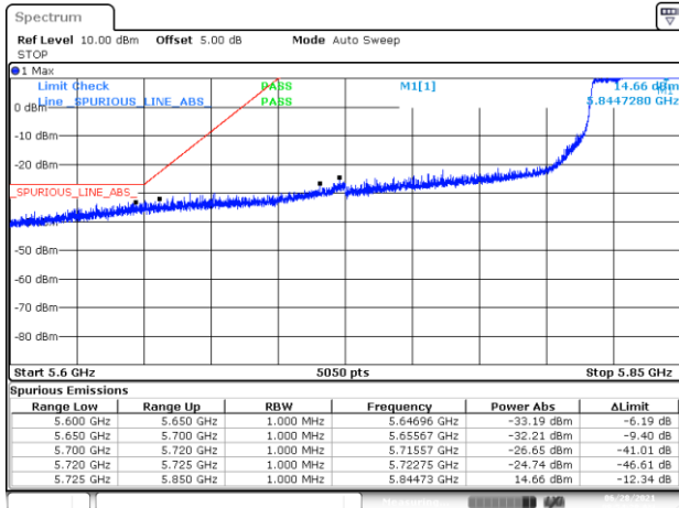
Date: 28.JUN.2021 08:54:28 BE-NR-LOW, MIMO-B, 802.11ac80-VHT0, Ch171
