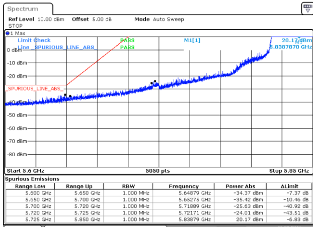
BE-NR-LOW, MIMO-A, 802.11n40-HT8, Ch167
