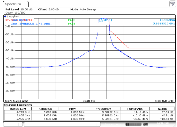
BE-NR-HIGH, SISO-B, 802.11n20-HT0, Ch177
