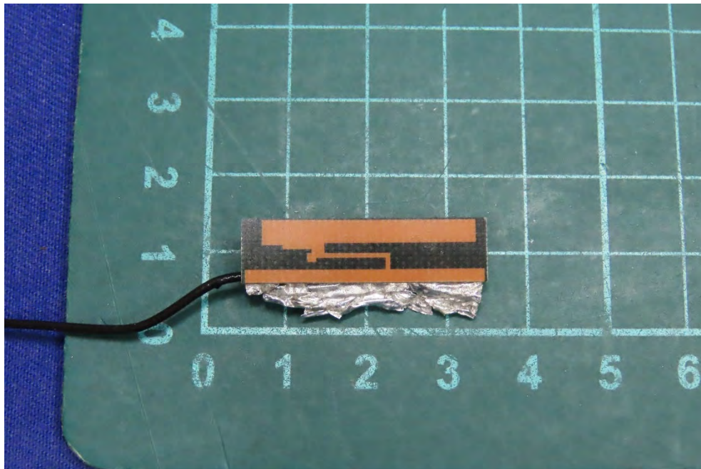
(36) EUT Photo_Plus Main Antenna
