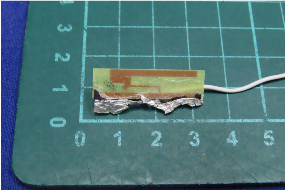
(38) EUT Photo_Plus Aux Antenna
