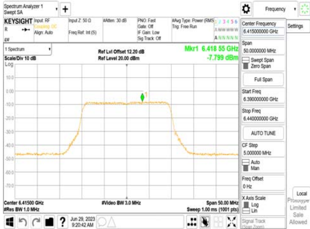
802.11be_20MHz_Chain1_6415MHz_106+26_MRU2
