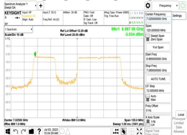
802.11be_80MHz_Chain0_7025MHz_RU484+242_Punc20
