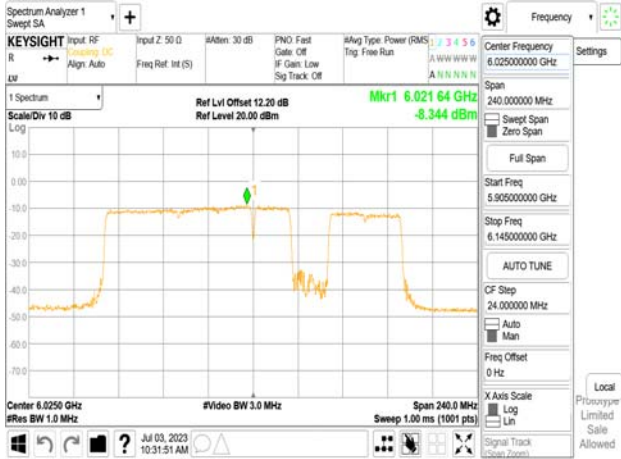
802.11be_160MHz_Chain1_6025MHz_SU_Punct40_Mid2
