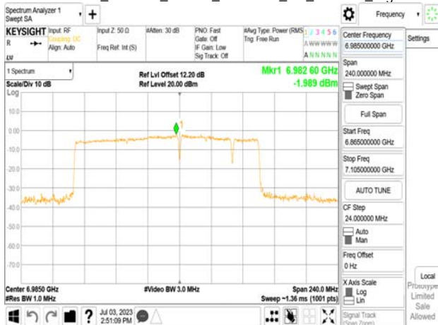
802.11be_160MHz_Chain1_6985MHz_SU_Punct20_Mid3
