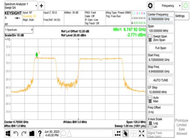
802.11be_80MHz_Chain0_6785MHz_SU_Punct20_Mid2
