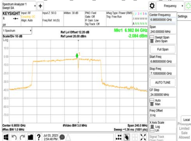
802.11be_160MHz_Chain1_6985MHz_SU_Punct40_High
