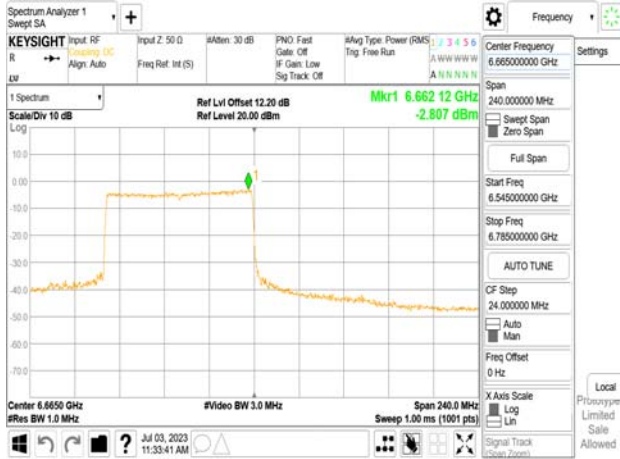
802.11be_160MHz_Chain0_6665MHz_SU_Punct20_High
