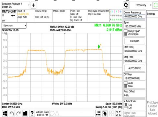
802.11be_80MHz_Chain0_6625MHz_SU_Punct20_Mid2
