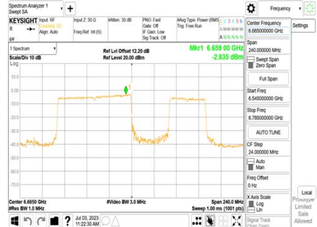
802.11be_160MHz_Chain0_6665MHz_SU_Punct40_Mid2
