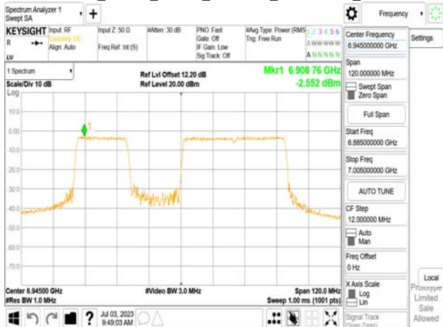
802.11be_80MHz_Chain0_6945MHz_RU484+242_Punc20
