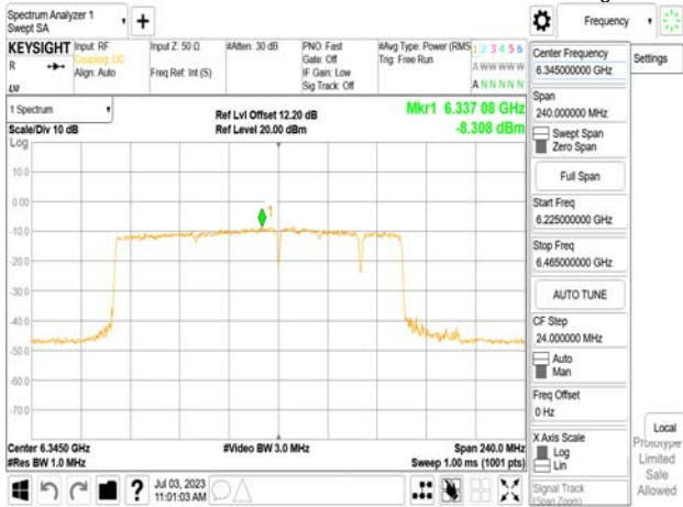
802.11be_160MHz_Chain0_6345MHz_SU_Punct40_High
