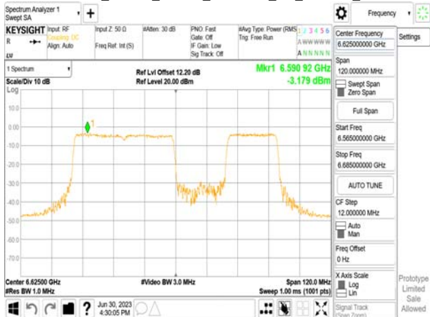
802.11be_80MHz_Chain1_6625MHz_SU_Punc20_Mid2
