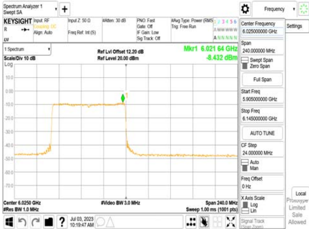
802.11be_160MHz_Chain1_6025MHz_SU_Punct20_Mid3
