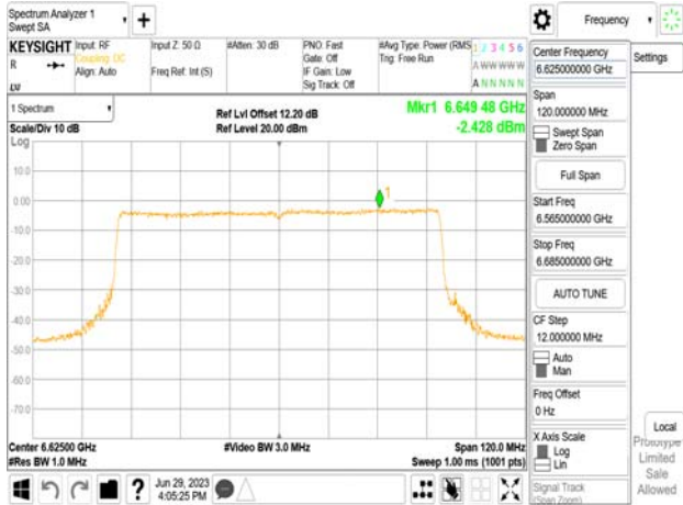
802.11be_80MHz_Chain1_6625MHz_RU484+242_Punc20
