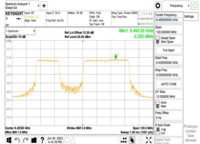
802.11be_80MHz_Chain1_6465MHz_SU_Punc20_Mid2
