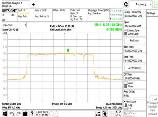
802.11be_160MHz_Chain1_6345MHz_SU_Punct20_High
