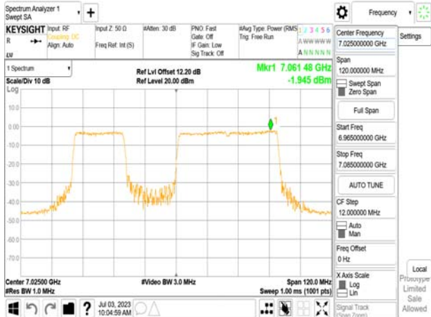
802.11be_80MHz_Chain1_7025MHz_SU_Punc20_Mid2
