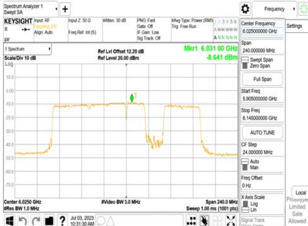
802.11be_160MHz_Chain0_6025MHz_SU_Punct40_Mid2
