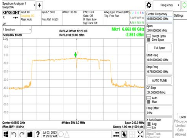
802.11be_160MHz_Chain0_6665MHz_SU_Punct20_High
