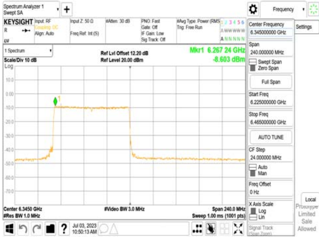
802.11be_160MHz_Chain0_6345MHz_SU_Punct20_High
