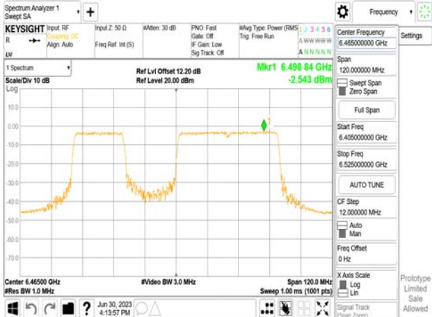
802.11be_80MHz_Chain0_6465MHz_RU484+242_Punc20
