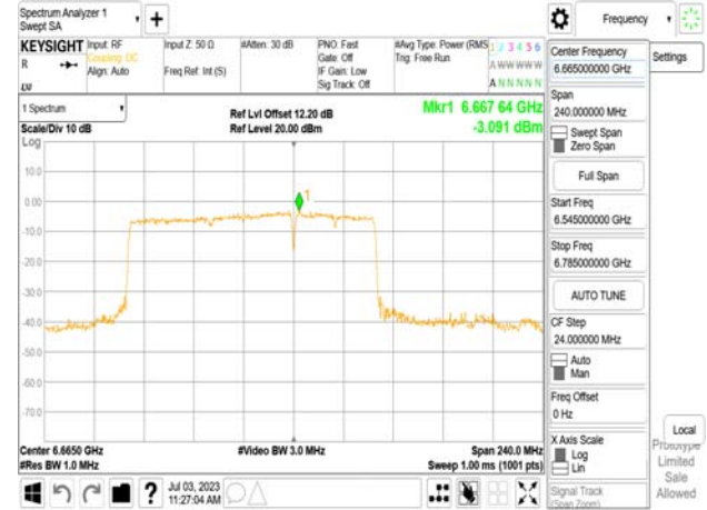
802.11be_160MHz_Chain0_6665MHz_SU_Punct40_Mid2
