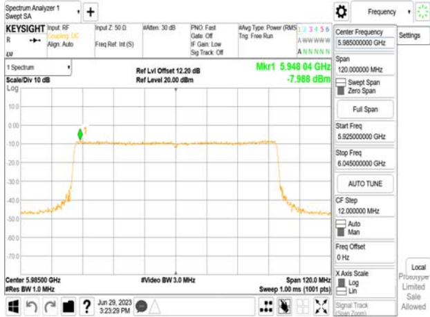
802.11be_80MHz_Chain1_5985MHz_RU484+242_Punc20
