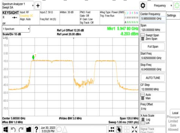
802.11be_80MHz_Chain0_5985MHz_SU_Punc20_Mid2
