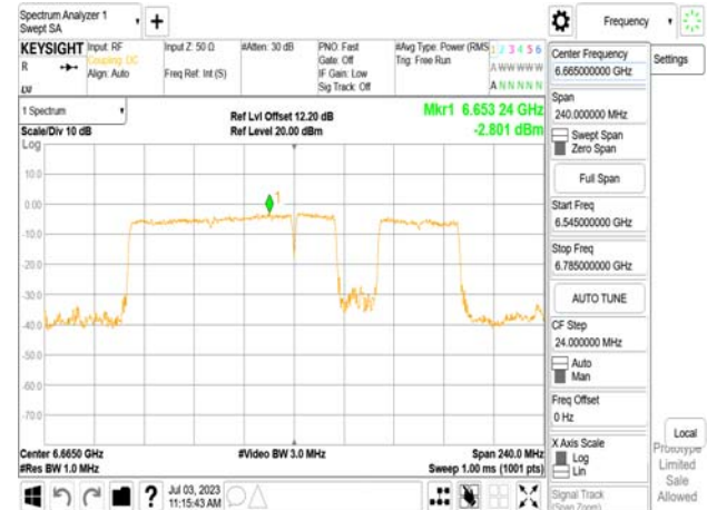
802.11be_160MHz_Chain1_6665MHz_SU_Punct40_High
