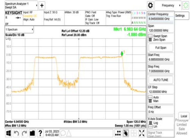
802.11be_80MHz_Chain1_6945MHz_SU_Punc20_Mid2
