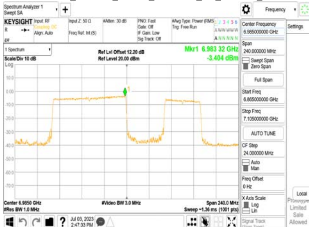
802.11be_160MHz_Chain0_6985MHz_SU_Punct40_Mid2
