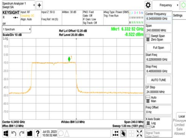
802.11be_160MHz_Chain1_6345MHz_SU_Punct20_High
