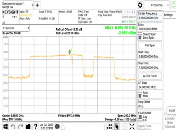
802.11be_160MHz_Chain0_6985MHz_SU_Punct40_High
