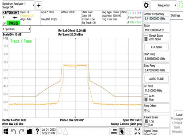
802.11be_20MHz_Chain1_6415MHz_106+26_MRU2
