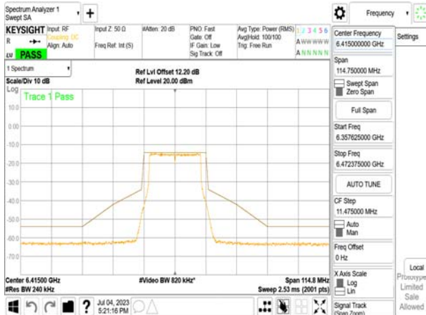
802.11be_20MHz_Chain0_6415MHz_106+26_MRU2
