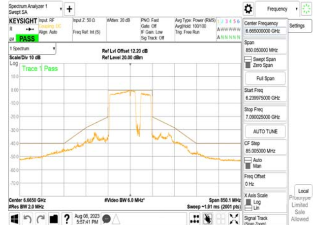
802.11be_160MHz_Chain0_6665MHz_SU_Punct40_High
