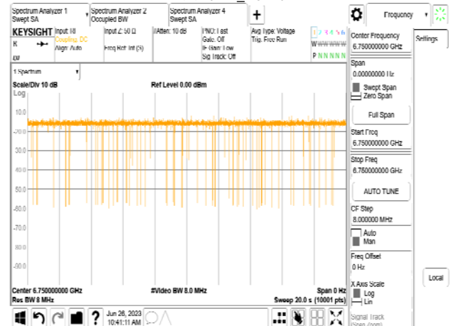
802.11be_320MHz_CF 6905MHz_Interference_6750MHz_-79.92dBm_Normal
