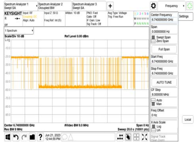
802.11be_320MHz_CF 6585MHz_Interference_6740MHz_-79.37dBm_Normal
