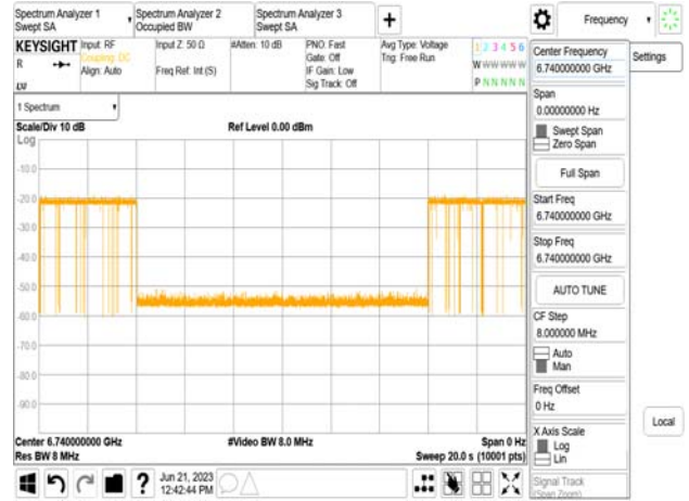
802.11be_320MHz_CF 6585MHz_Interference_6740MHz_-77.37dBm_Minimal
