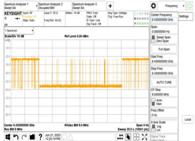
802.11be_320MHz_CF 6585MHz_Interference_6430MHz_-79.43dBm_Normal
