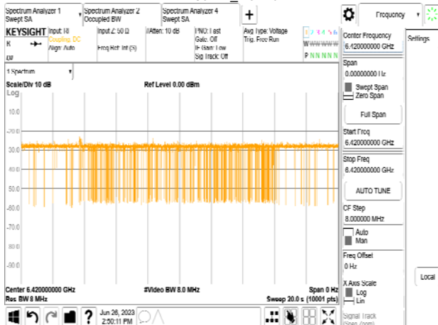
802.11be_320MHz_CF 6265MHz_Interference_6420MHz_-77.28dBm_Normal
