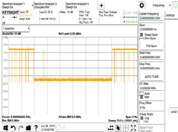
802.11be_320MHz_CF 6745MHz_Interference_6900MHz_-79.32dBm_Normal
