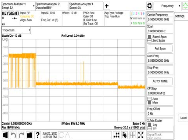
802.11be_320MHz_CF 6585MHz_Interference_6585MHz_-78.32dBm_NormaldBm_Normal
