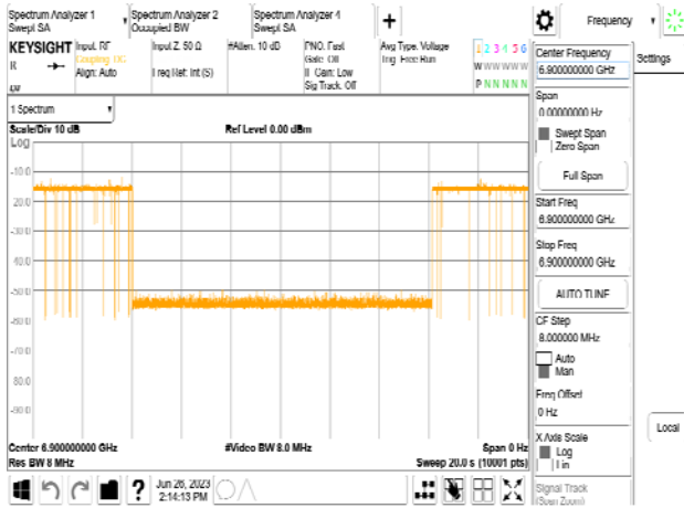
802.11be_320MHz_CF 6745MHz_Interference_6900MHz_-75.32dBm_Minimal
