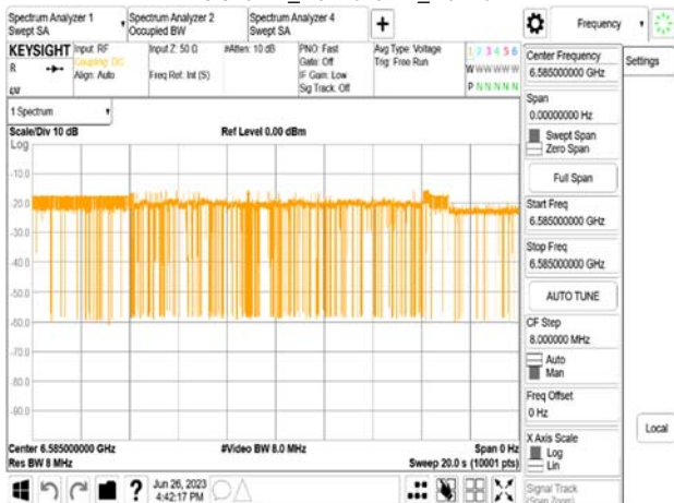
802.11be_320MHz_CF 6585MHz_Interference_6585MHz_-78.32dBm_NormaldBm_Normal
