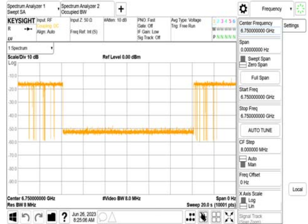
802.11be_320MHz_CF 6905MHz_Interference_6750MHz_-76.92dBm_Minimal
