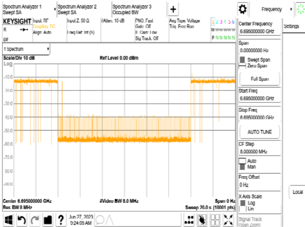
802.11be_20MHz_CF 6695MHz_Interference_6695MHz_-83.47dBm_Normal
