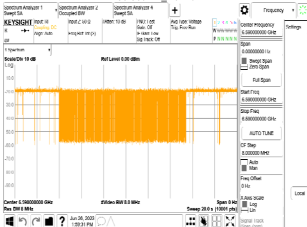
802.11be_320MHz_CF 6745MHz_Interference_6590MHz_-80.36dBm_Normal
