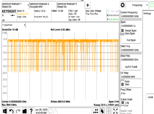
802.11be_320MHz_CF 6905MHz_Interference_6905MHz_-77.76dBm_Normal
