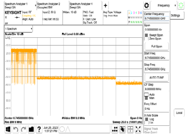
802.11be_320MHz_CF 6745MHz_Interference_6745MHz_-73.42dBm_Minimal
