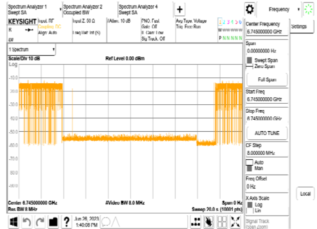
802.11be_320MHz_CF 6745MHz_Interference_6745MHz_-78.42dBm_Normal
