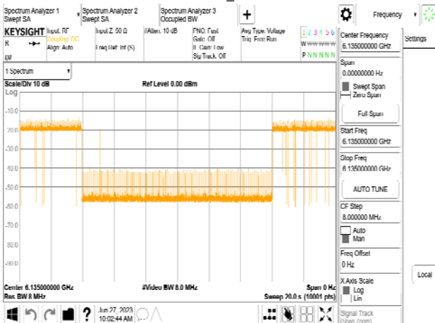
802.11be_20MHz_CF 6135MHz_Interference_6135MHz_-82.25dBm_Normal
