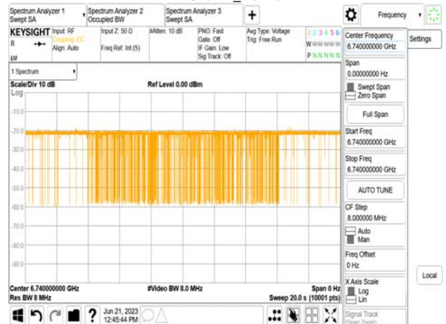
802.11be_320MHz_CF 6585MHz_Interference_6740MHz_-79.37dBm_Normal
