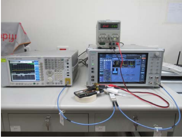
FCC_22_24_27_LTE_ULCA_Radiated_Setup
