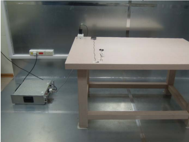
FCC_15_247_BT_Conduction_Setup
