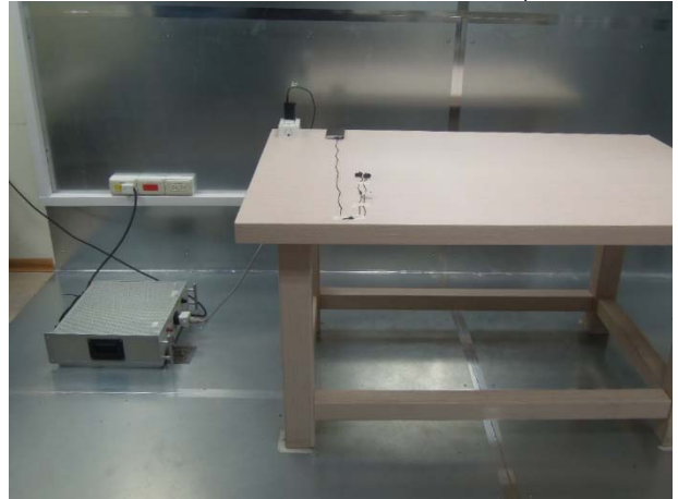
FCC_15_407_WLAN_Conduction_Setup
