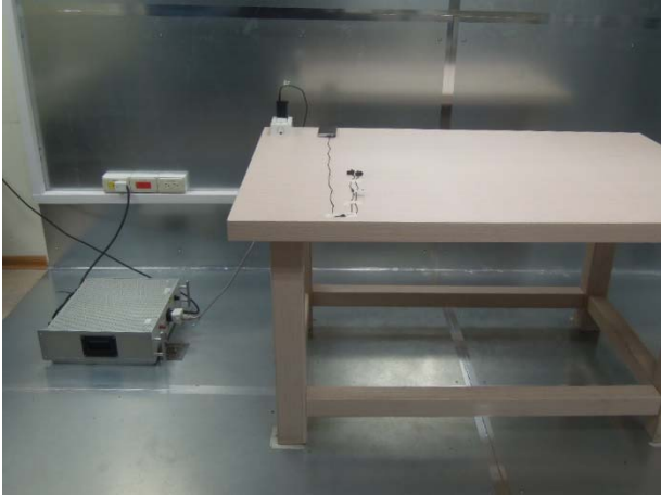
FCC_15_247_WLAN_Conduction_Setup
