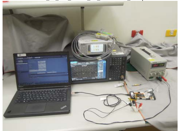
FCC_15_407_WLAN_6E_Conducted_Setup
