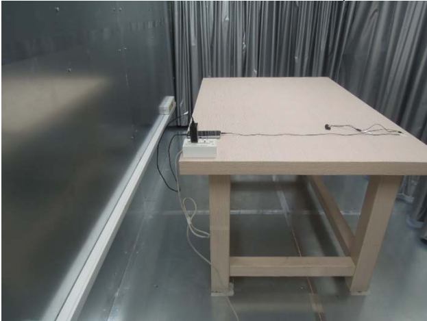
FCC_22_24_27_2_3G_Conducted_SETUP
