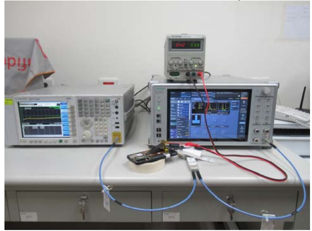
FCC_22_24_27_LTE_Radiated_Setup
