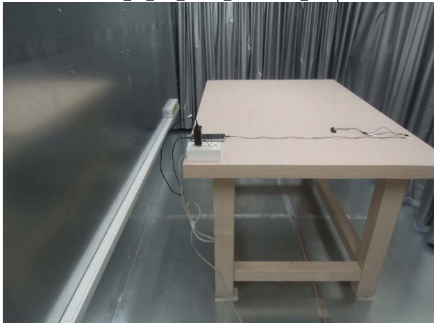
FCC_15_247_WLAN_Conduction_Setup
