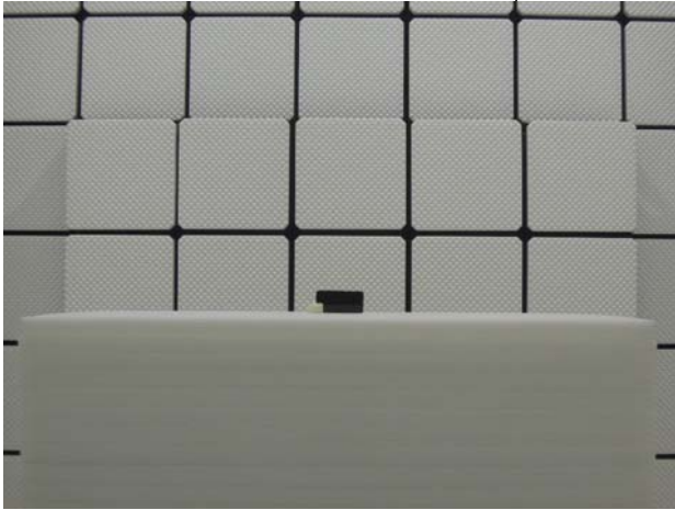
FCC_22_24_27_FR1_Radiated_Setup
