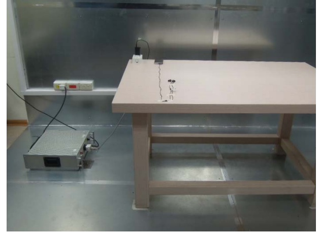
FCC_15_407_WLAN_6E_Conduction_Setup
