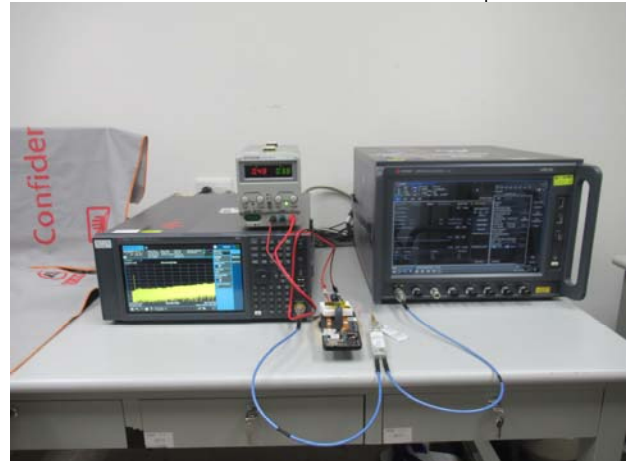
FCC_22_24_27_FR1_Conducted_Setup
