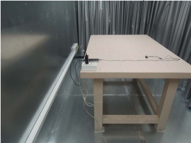
FCC_15_247_WLAN_Conducted_Setup
