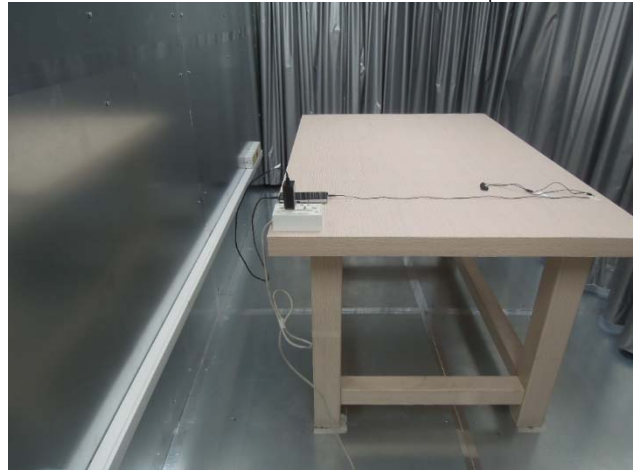
FCC_15_407_WLAN_6E_Conducted_Setup
