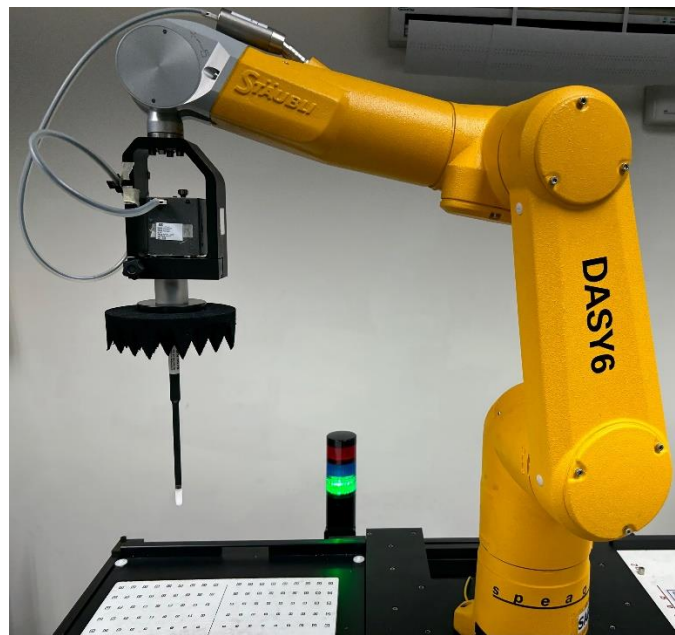
Fig.1 Photograph of the SAR measurement system
