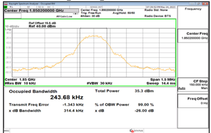
GSM_1900MHz_LowCH512-1850.2
