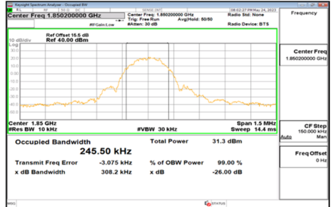
EDGE_1900MHz_LowCH512-1850.2
