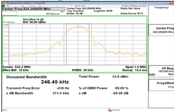
EDGE_850MHz_LowCH128-824.2
