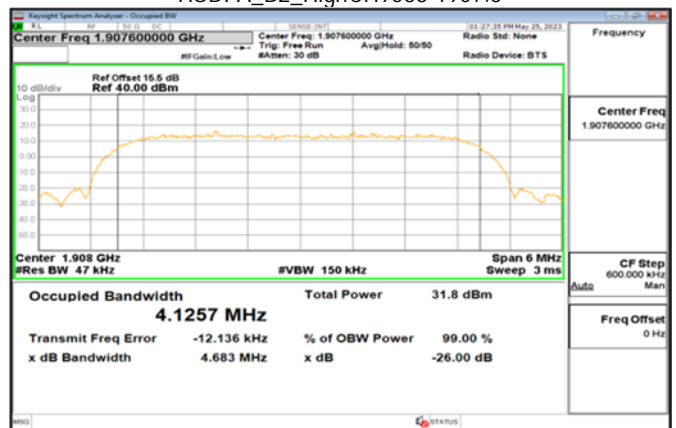
HSDPA_B2_HighCH9538-1907.6
