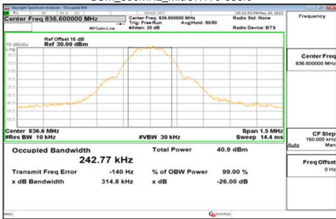
GSM_850MHz_MidCH190-836.6
