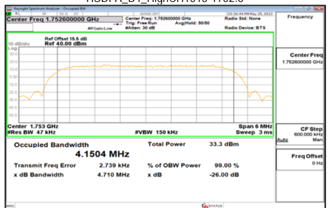
HSDPA_B4_HighCH1513-1752.6
