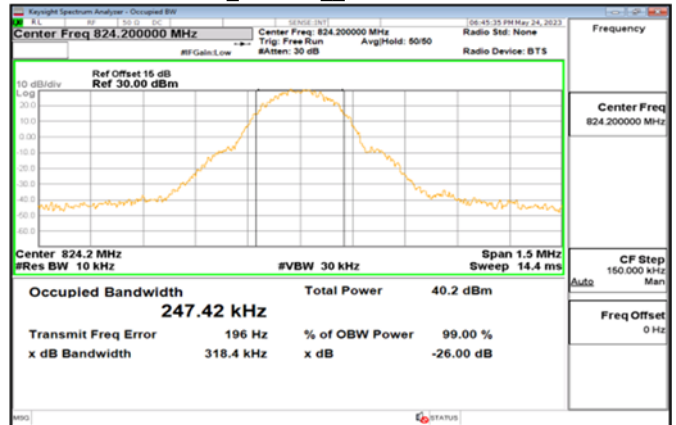
GPRS_850MHz_LowCH128-824.2
