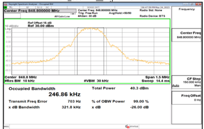
EDGE_850MHz_HighCH251-848.8
