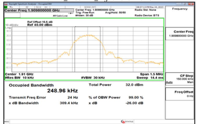
GPRS_1900MHz_HighCH810-1909.8
