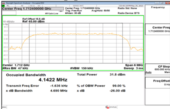
HSDPA_B4_LowCH1312-1712.4
