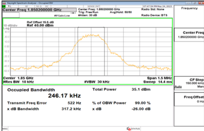
GPRS_1900MHz_LowCH512-1850.2
