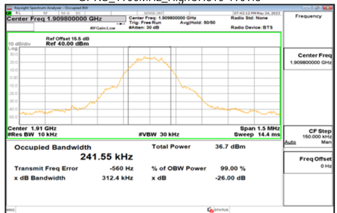
GPRS_1900MHz_HighCH810-1909.8
