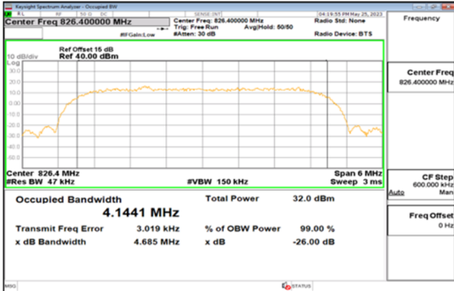
HSUPA_B5_LowCH4132-826.4
