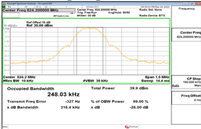
GSM_850MHz_LowCH128-824.2
