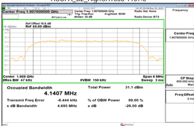
HSUPA_B2_HighCH9538-1907.6
