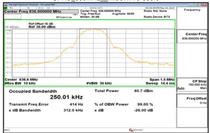
GPRS_850MHz_MidCH190-836.6
