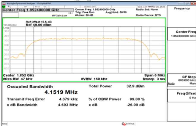
WCDMA_B2_LowCH9262-1852.4
