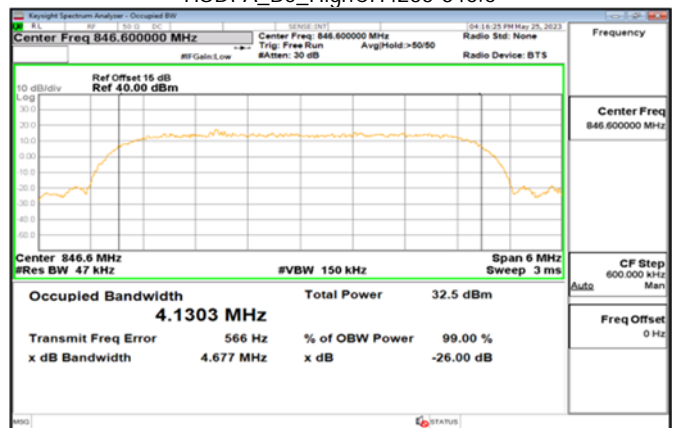
HSDPA_B5_HighCH4233-846.6
