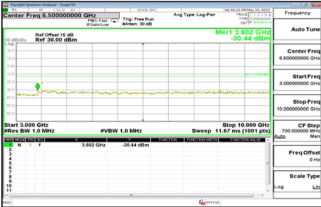
GP RS_850MHz_MidCH190-836.6
