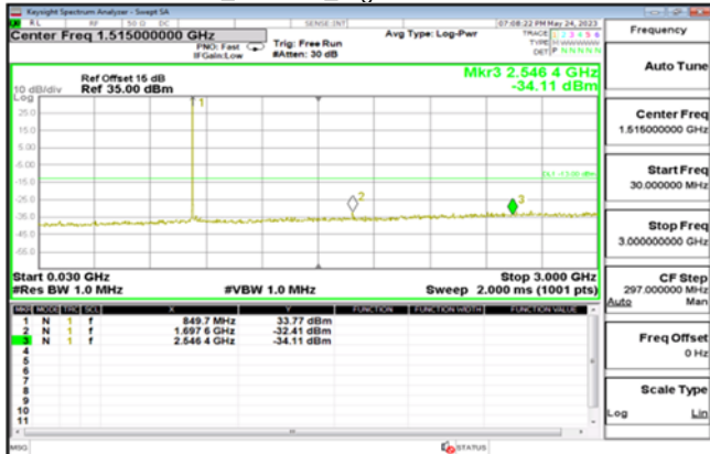
GSM_850MHz_HighCH251-848.8
