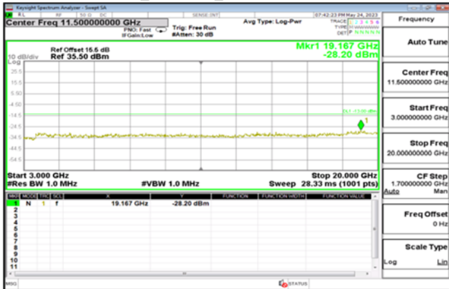
GSM_1900MHz_HighCH810-1909.8
