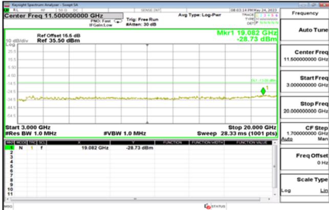
EDGE_1900MHz_MidCH661-1880
