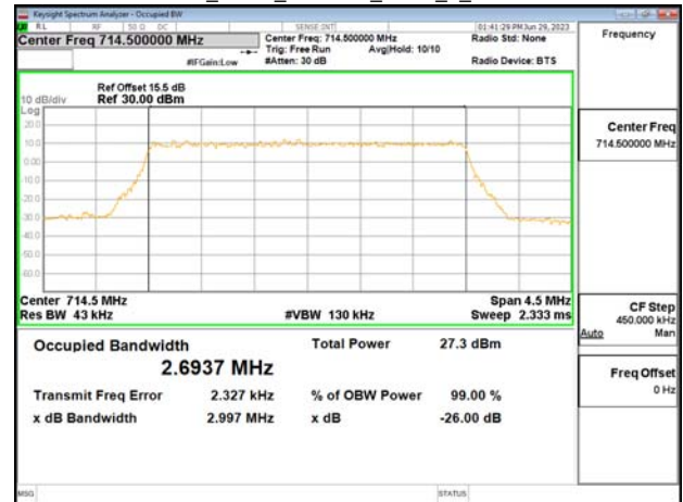
Band12_3MHz_256QAM_RB15_0_CH23165
