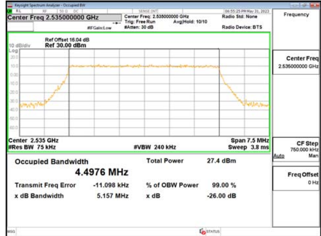
Band7_5MHz_256QAM_RB25_0_CH21425
