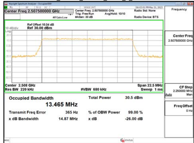
Band7_15MHz_16QAM_RB75_0_CH21100
