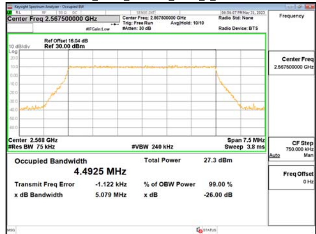
Band7_5MHz_256QAM_RB25_0_CH21425
