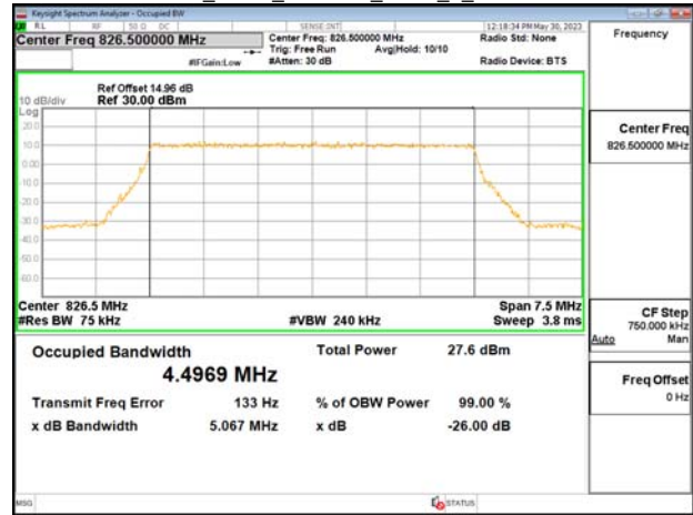
Band5_5MHz_256QAM_RB25_0_CH20525
