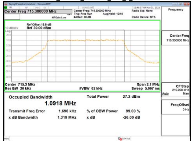
Band12_1.4MHz_256QAM_RB6_0_CH23173
