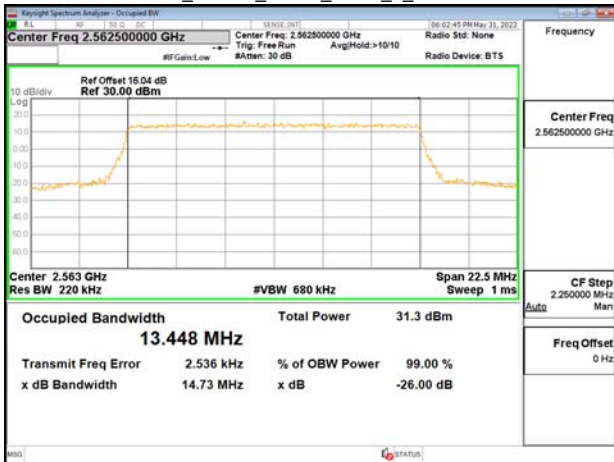
Band7_15MHz_QPSK_RB75_0_CH21375
