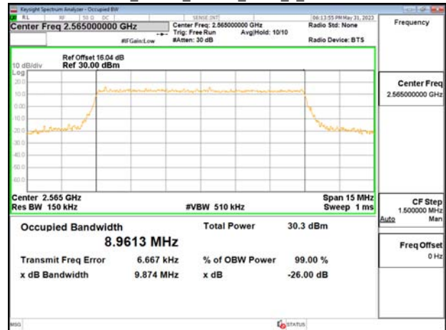
Band7_10MHz_16QAM_RB50_0_CH21400
