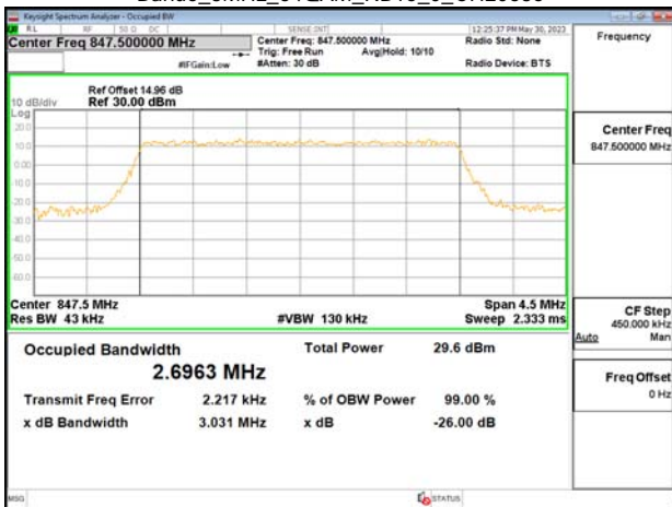
Band5_3MHz_64QAM_RB15_0_CH20635
