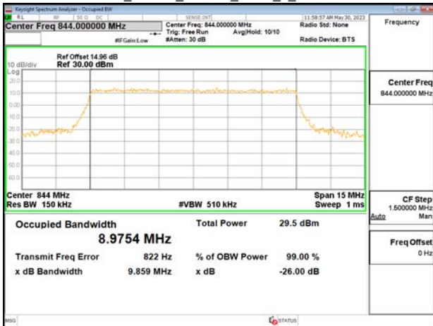
Band5_10MHz_64QAM_RB50_0_CH20600
