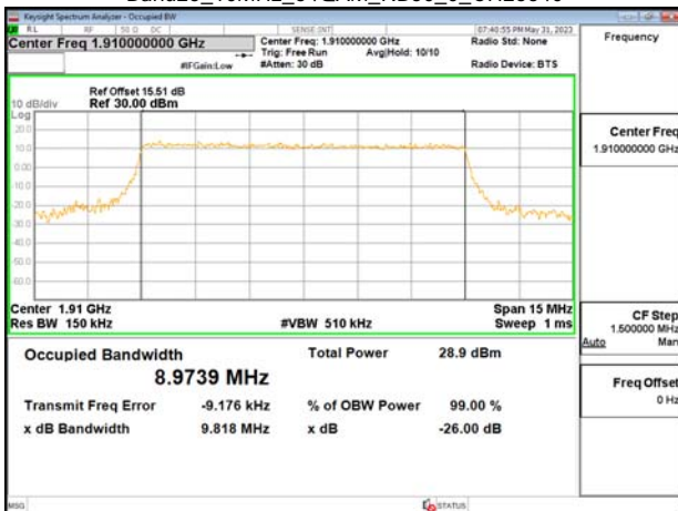
Band25_10MHz_64QAM_RB50_0_CH26640
