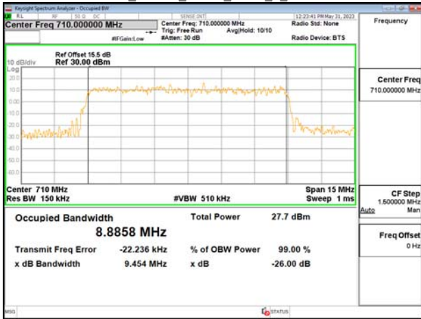
Band17_10MHz_QPSK_RB50_0_CH23800
