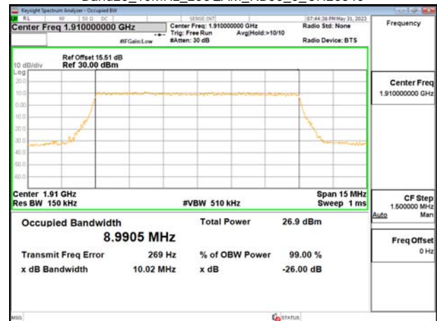
Band25_10MHz_256QAM_RB50_0_CH26640
