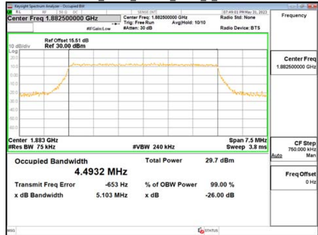
Band25_5MHz_16QAM_RB25_0_CH26665
