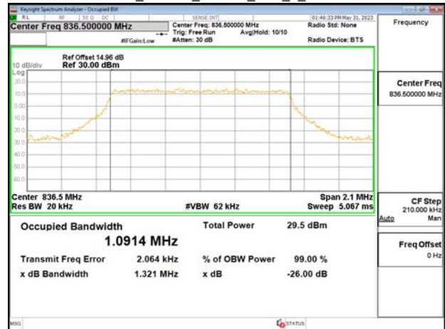
Band26_1.4MHz_64QAM_RB6_0_CH26915
