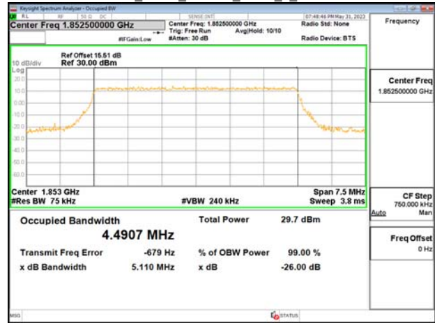
Band25_5MHz_16QAM_RB25_0_CH26365
