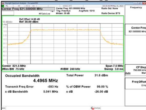
Band26-Part90s_5MHz_QPSK_RB25_0_CH26765
