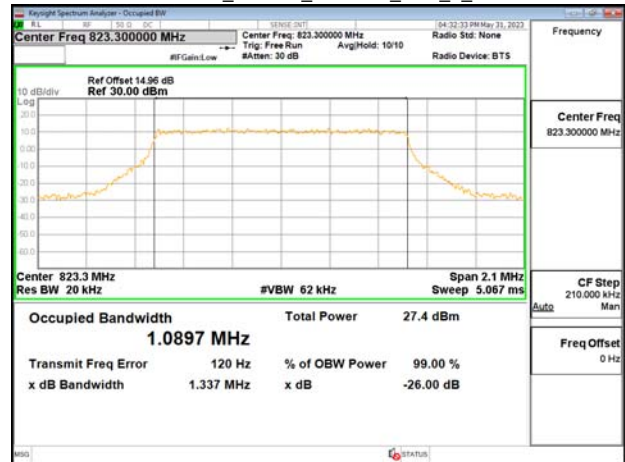
Band26-Part90s_1.4MHz_256QAM_RB6_0_CH26783
