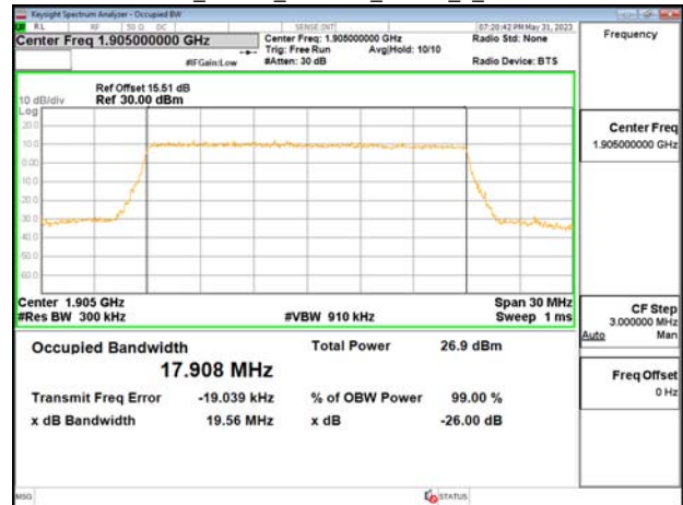
Band25_20MHz_256QAM_RB100_0_CH26590
