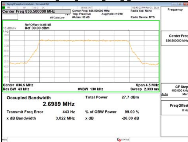
Band26_3MHz_256QAM_RB15_0_CH26915
