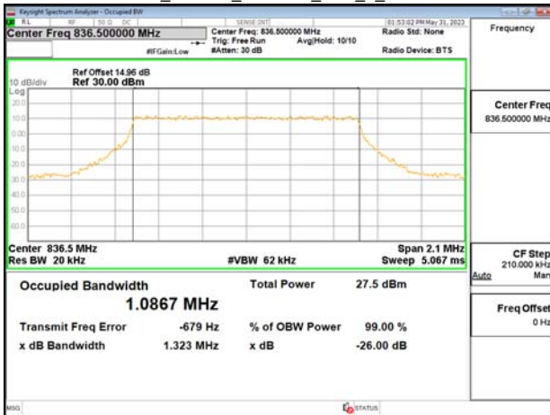
Band26_1.4MHz_256QAM_RB6_0_CH26915
