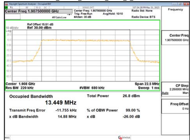
Band25_15MHz_256QAM_RB75_0_CH26615
