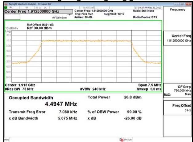
Band25_5MHz_256QAM_RB25_0_CH26665
