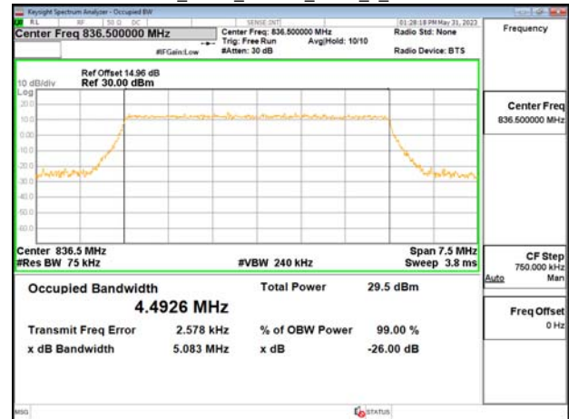
Band26_5MHz_64QAM_RB25_0_CH26915
