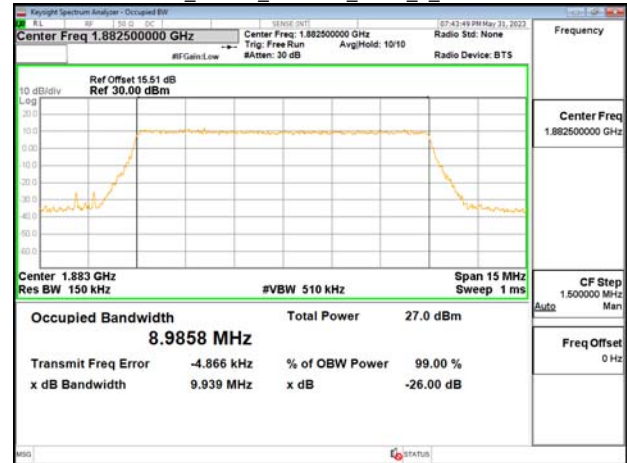
Band25_10MHz_256QAM_RB50_0_CH26640
