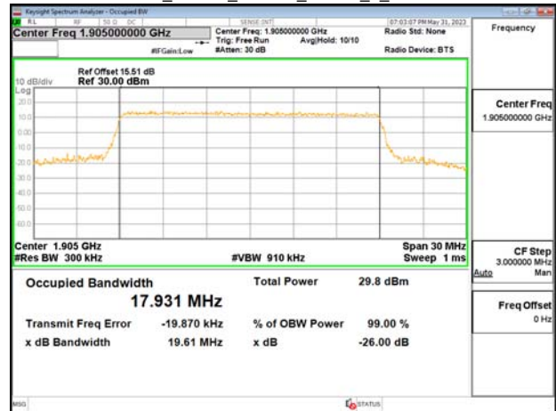
Band25_20MHz_16QAM_RB100_0_CH26590
