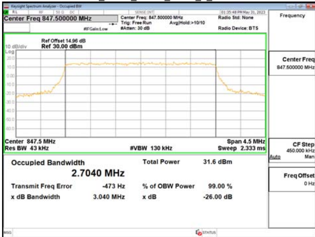
Band26_3MHz_16QAM_RB15_0_CH26805
