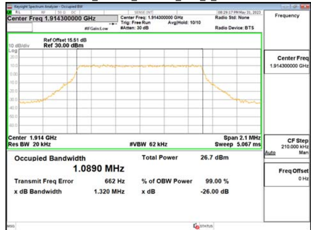
Band25_1.4MHz_256QAM_RB6_0_CH26683
