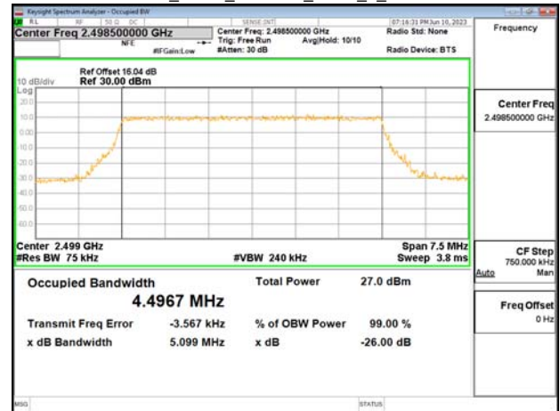
Band41_5MHz_256QAM_RB25_0_CH39675
