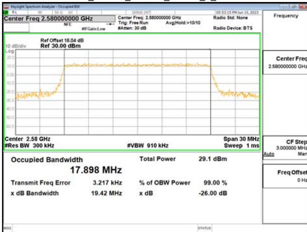
Band38_20MHz_64QAM_RB100_0_CH37850
