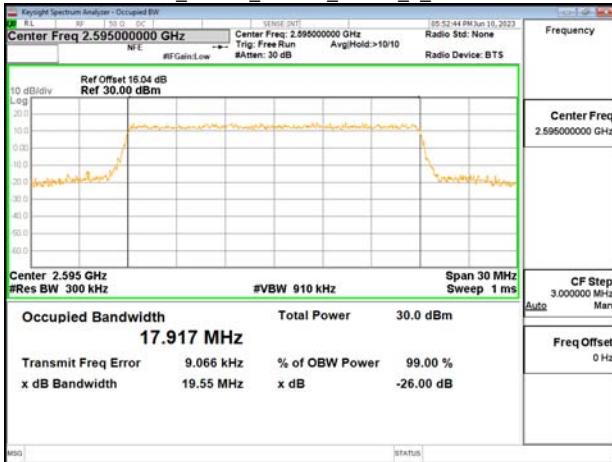
Band38_20MHz_16QAM_RB100_0_CH38150
