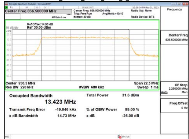
Band26_15MHz_QPSK_RB75_0_CH26915
