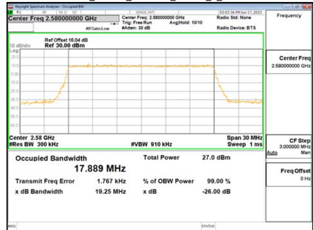
Band38_20MHz_256QAM_RB100_0_CH37850
