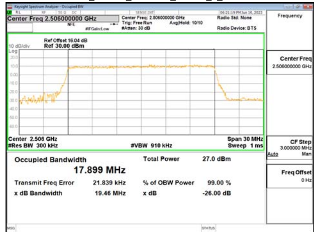
Band41_20MHz_256QAM_RB100_0_CH39750
