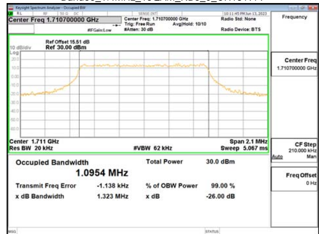
Band66_1.4MHz_16QAM_RB6_0_CH131979
