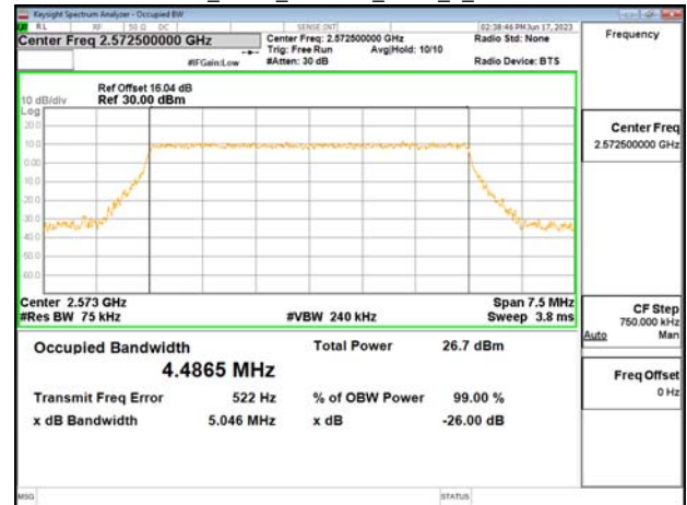
Band38_5MHz_256QAM_RB25_0_CH37775
