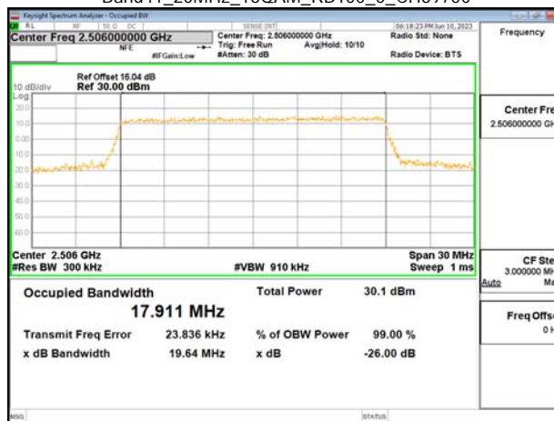
Band41_20MHz_16QAM_RB100_0_CH39750
