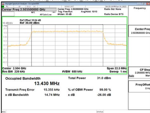
Band41_15MHz_QPSK_RB75_0_CH39725
