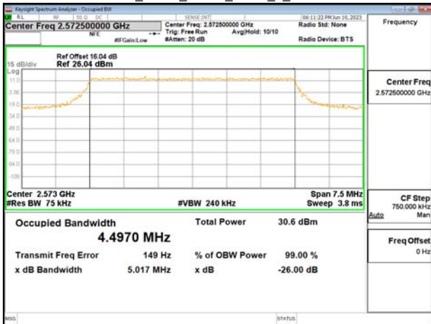
Band38_5MHz_QPSK_RB25_0_CH37775
