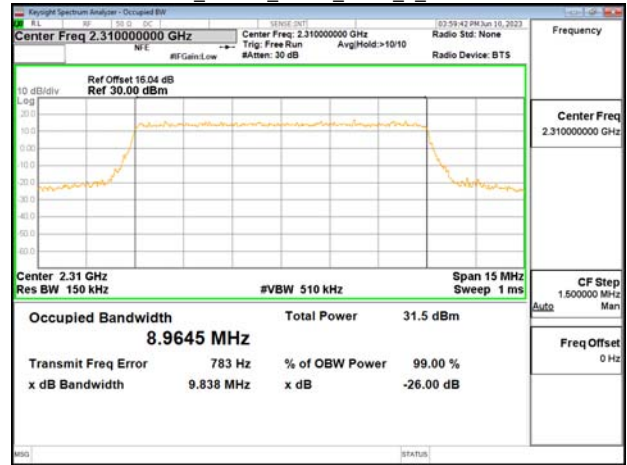
Band30_10MHz_16QAM_RB50_0_CH27710
