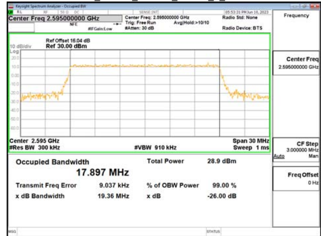
Band38_20MHz_64QAM_RB100_0_CH38150
