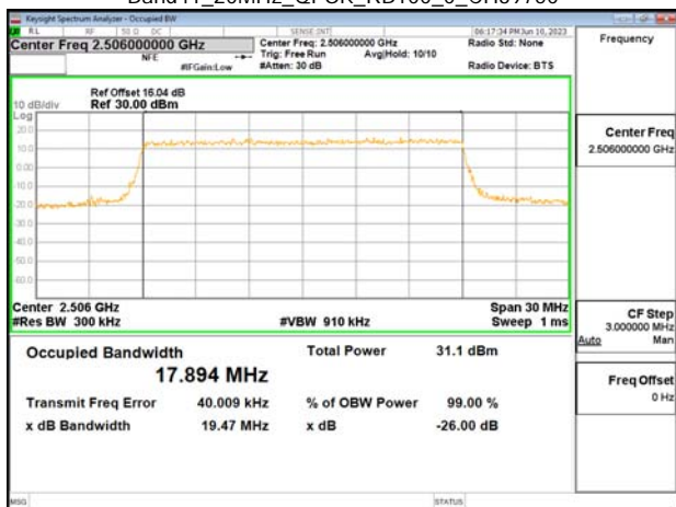
Band41_20MHz_QPSK_RB100_0_CH39750
