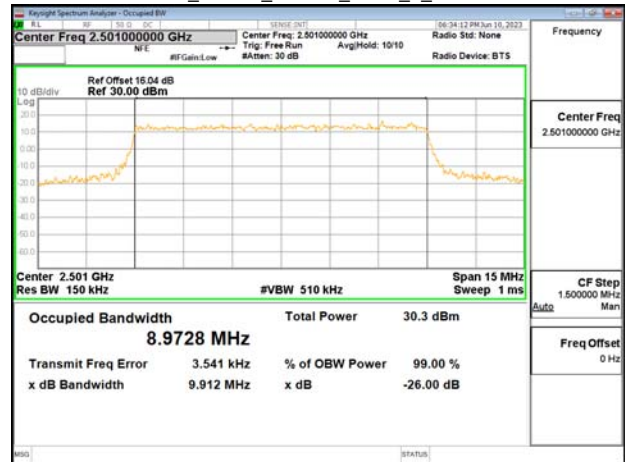
Band41_10MHz_16QAM_RB50_0_CH39700
