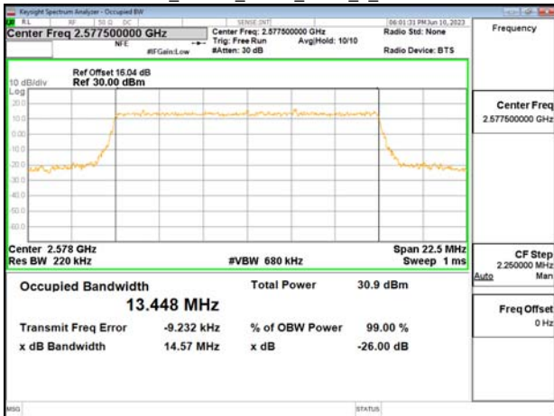
Band38_15MHz_QPSK_RB75_0_CH37825
