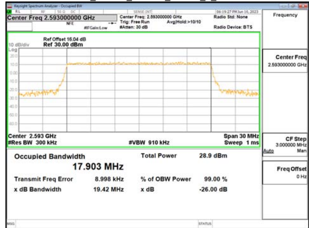
Band41_20MHz_64QAM_RB100_0_CH41490
