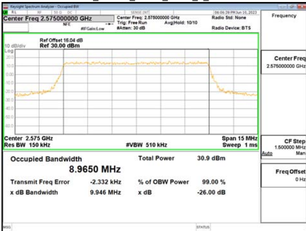
Band38_10MHz_QPSK_RB50_0_CH37800
