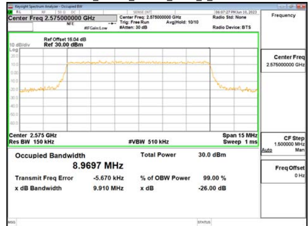
Band38_10MHz_16QAM_RB50_0_CH37800
