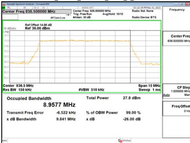
Band26_10MHz_256QAM_RB50_0_CH26915
