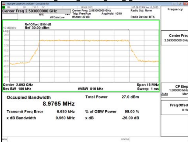
Band41_10MHz_256QAM_RB50_0_CH41540
