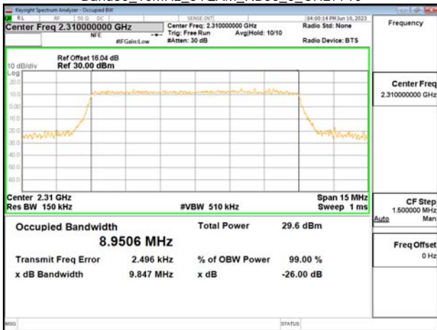
Band30_10MHz_256QAM_RB50_0_CH27710
