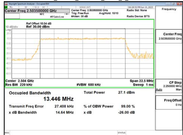
Band41_15MHz_256QAM_RB75_0_CH39725
