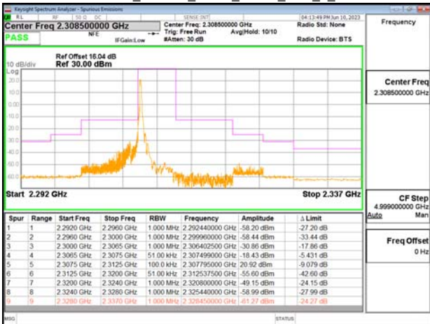
Emission Mask_Band30_5MHz_OPSK_RB1_0_CH27710
