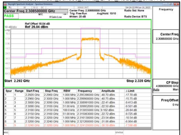
Emission Mask_Band30_10MHz_QPSK_RB1_0_CH27710
