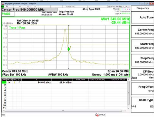
Band Edge_Band26_10MHz_OPSK_RB50_0_CH26840
