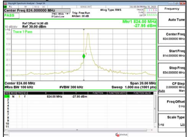
Band Edge_Band26_10MHz_QPSK_RB1_0_CH26840
