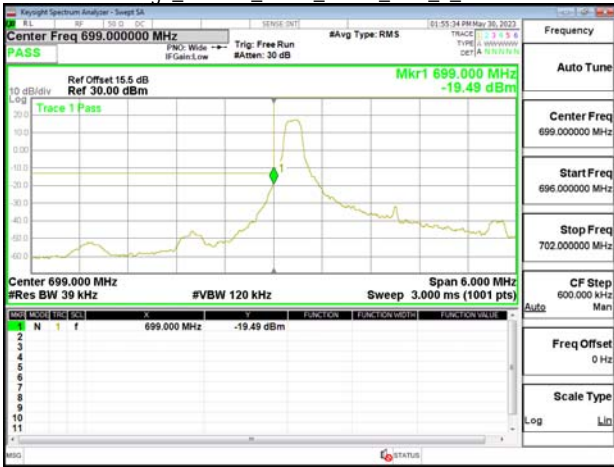
Band Edge_Band12_3MHz_OPSK_RB1_14_CH23165
