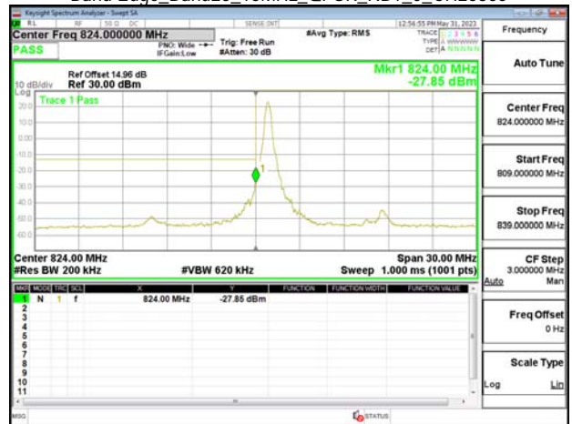
Band Edge_Band26_15MHz_OPSK_RB1_74_CH26965
