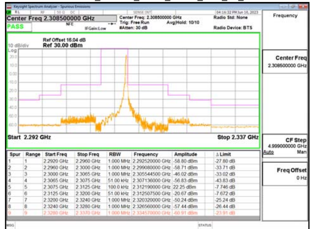
Emission Mask_Band30_5MHz_OPSK_RB1_24_CH27710
