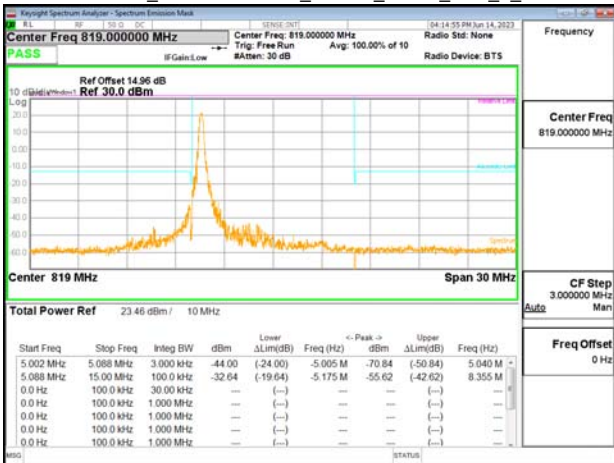
Emission Mask_Band26-Part90s_10MHz_OPK RB1_0_CH26740
