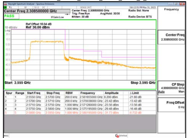
Emission Mask_Band7_10MHz_QPSK_RB50_0_CH21400
