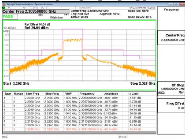
Emission Mask_Band30_5MHz_QPSK_RB25_0_CH27710
