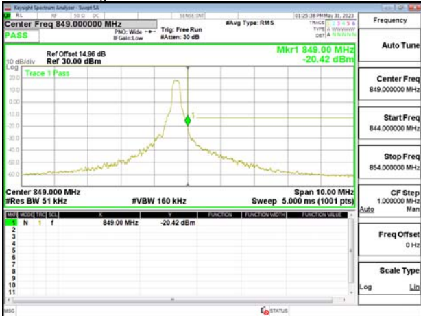
Band Edge_Band26_5MHz_QPSK_RB1_24_CH27015
