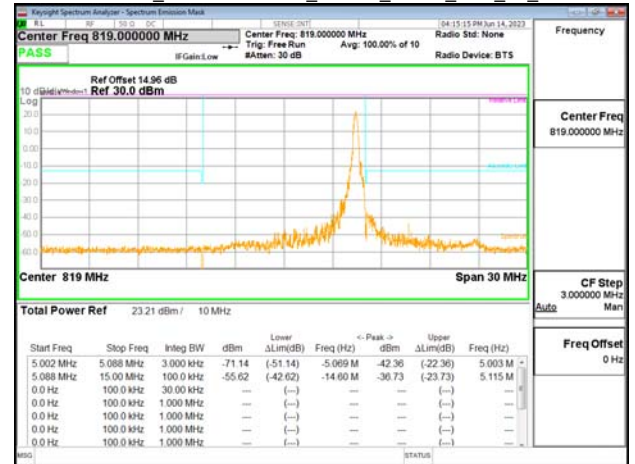
Emission Mask_Band26-Part90s_10MHz_OPK RB50_0_CH26740
