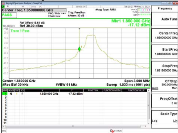
Band Edge_Band25_1.4MHz_QPSK_RB1_0_CH26047
