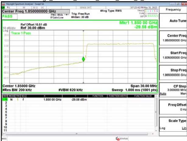
Band Edge_Band25_15MHz_QPSK_RB75_0_CH26115
