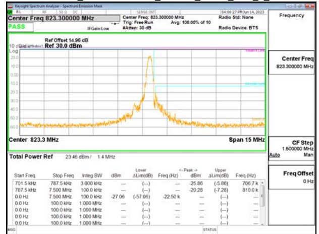
Emission Mask_Band26-Part90s_1.4MHz_QPSK_RB6_0_CH26697
