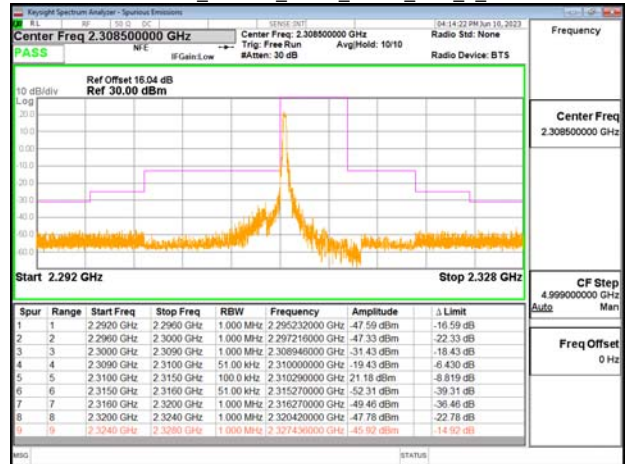
Emission Mask_Band30_5MHz_OPSK_RB1_24_CH27685
