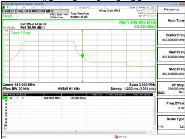
Band Edge_Band26_1.4MHz_QPSK_RB6_0_CH27033
