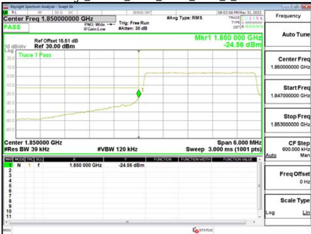
Band Edge_Band25_3MHz_OPSK_RB15_0_CH26055
