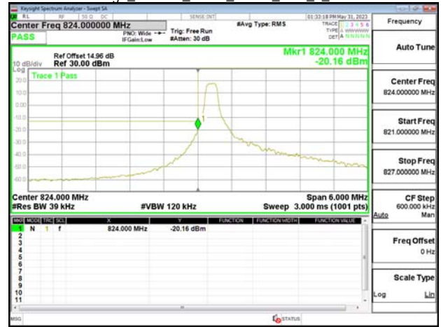
Band Edge_Band26_3MHz_QPSK_RB1_14_CH27025
