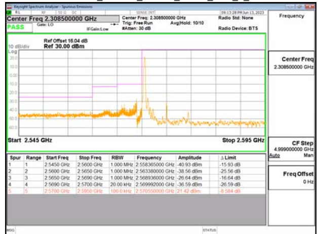
Emission Mask_Band38_10MHz_OPSK_RB1_0_CH37800
