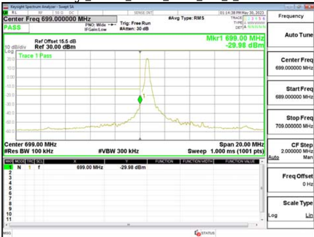
Band Edge_Band12_10MHz_QPSK_RB1_0_CH23060
