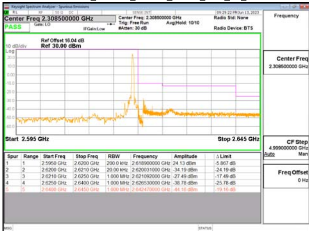
Emission Mask_Band38_20MHz_QPSK_RB1_99_CH38150
