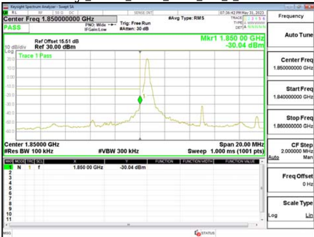
Band Edge_Band25_10MHz_QPSK_RB1_0_CH26090
