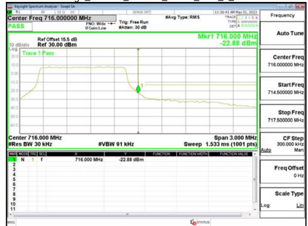
Band Edge_Band12_1.4MHz_QPSK_RB6_0_CH23173
