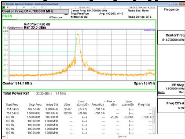
Emission Mask_Band26-Part90s_1.4MHz_QPSK_RB1_0_CH26697
