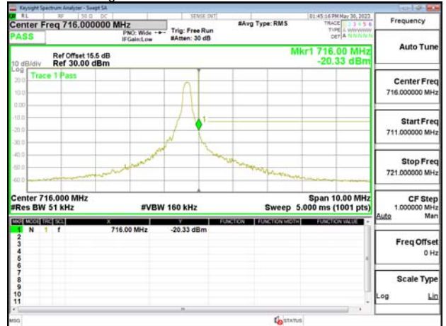
Band Edge_Band12_5MHz_OPSK_RB1_24_CH23155
