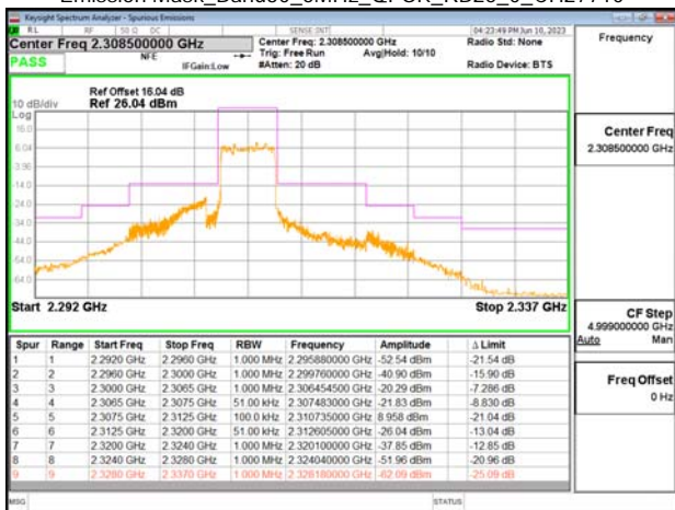
Emission Mask_Band30_5MHz_QPSK_RB25_0_CH27710
