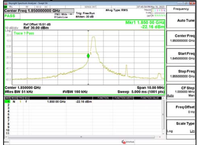
Band Edge_Band25_5MHz_OPSK_RB1_24_CH26665
