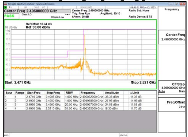
Emission Mask_Band41_5MHz_QPSK_RB1_0_CH39675
