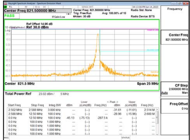
Emission Mask_Band26-Part90s_5MHz_QPSK_RB1_24_CH26765
