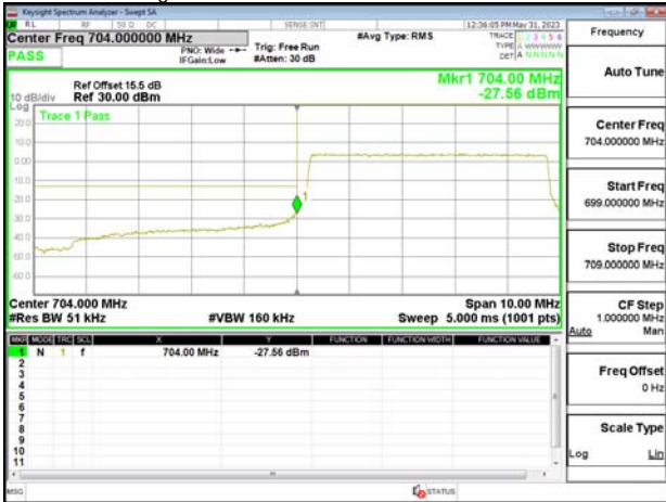
Band Edge_Band17_5MHz_QPSK_RB25_0_CH23755
