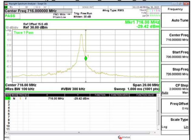
Band Edge_Band12_10MHz_QPSK_RB50_0_CH23060
