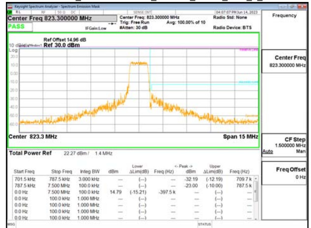
Emission Mask_Band26-Part90s_1.4MHz_QPSK_RB6_0_CH26783
