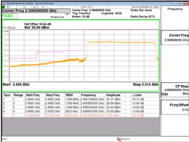
Emission Mask_Band7_15MHz_QPSK_RB75_0_CH20825
