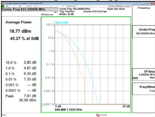
Band26-Part90s_1.4MHz_256QAM_RB6_0_CH26783
