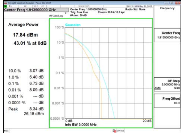
Band25_3MHz_256QAM_RB15_0_CH26675
