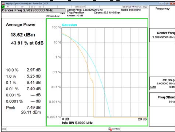
Band7_5MHz_256QAM_RB25_0_CH21100
