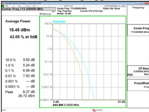
Band17_5MHz_256QAM_RB25_0_CH23825
