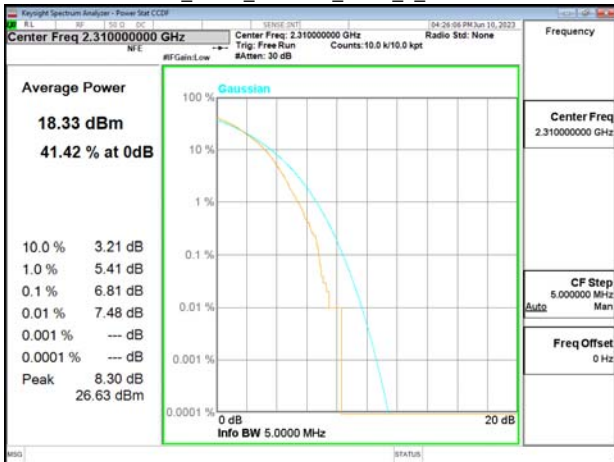
Band30_5MHz_256QAM_RB25_0_CH27710
