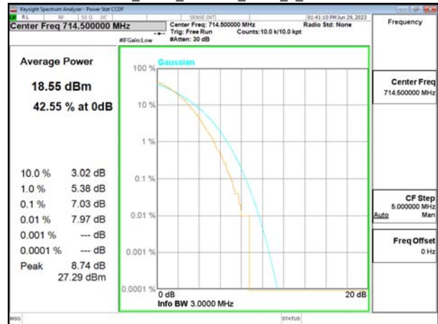
Band12_3MHz_256QAM_RB15_0_CH23165
