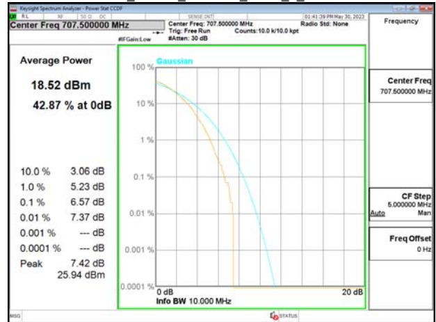
Band12_10MHz_256QAM_RB50_0_CH23130
