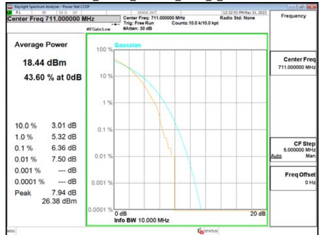
Band17_10MHz_256QAM_RB50_0_CH23800
