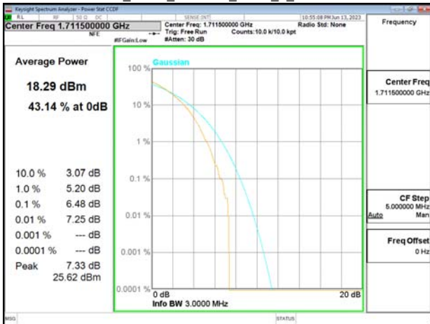
Band66_3MHz_256QAM_RB15_0_CH131987
