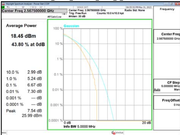
Band7_5MHz_256QAM_RB25_0_CH21425
