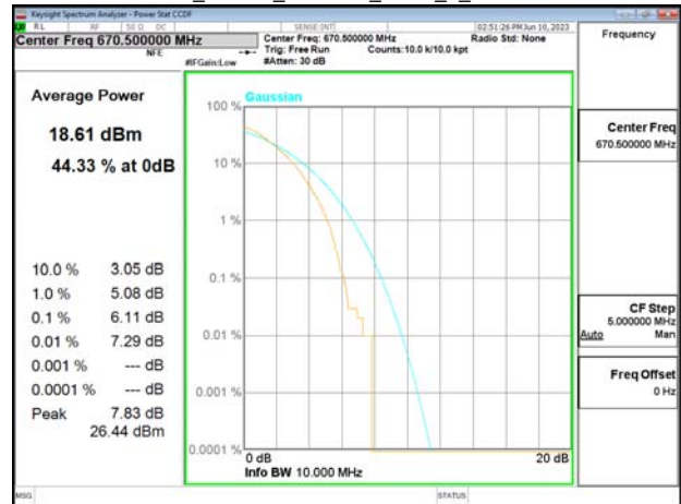
Band71_15MHz_256QAM_RB75_0_CH133197
