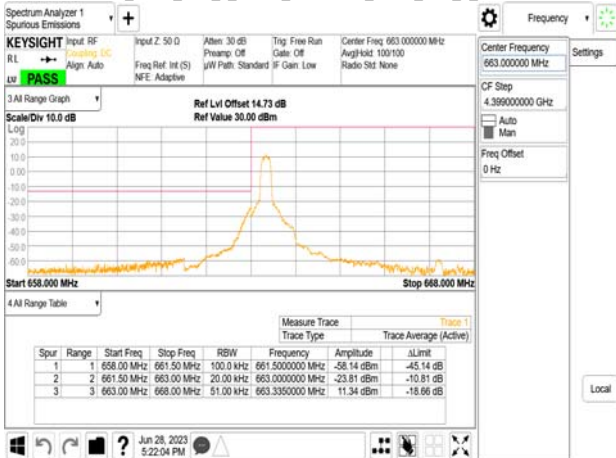
Band71_5MHz_DFT_s_OFDM_SCS15kHz_BPSK_RB1_24_CH1319100
