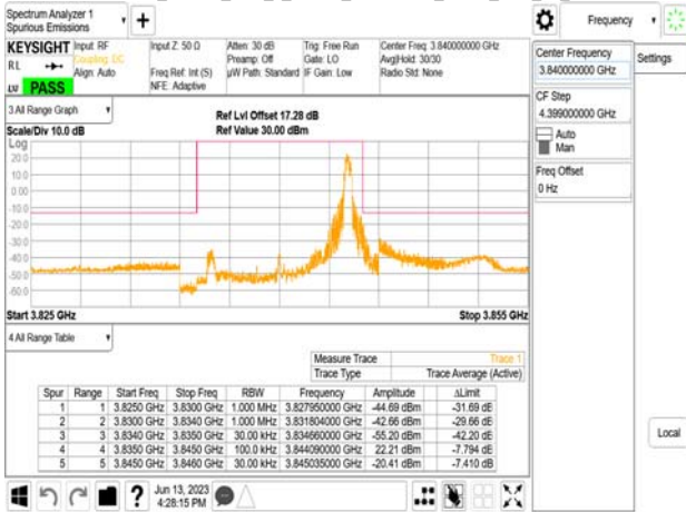
Band77-Part27_10MHz_DFT_s_OFDM_SCS30kHz_BPSK_RB1_23_CH656000
