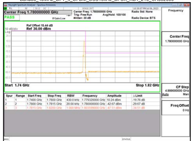
Band66_40MHz_DFT_s_OFDM_SCS15kHz_BPSK_RB1_215_CH352000
