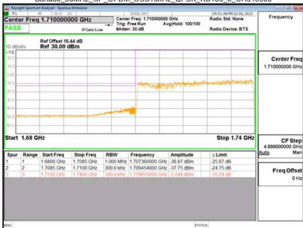
Band66_30MHz_CP_OFDM_SCS15kHz_OPSK_RB160_0_CH345000
