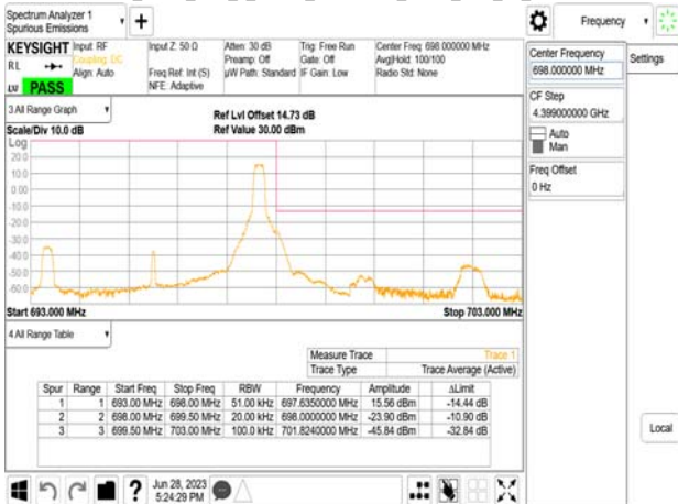
Band71_5MHz_DFT_s_OFDM_SCS15kHz_BPSK_RB25_0_CH1313100
