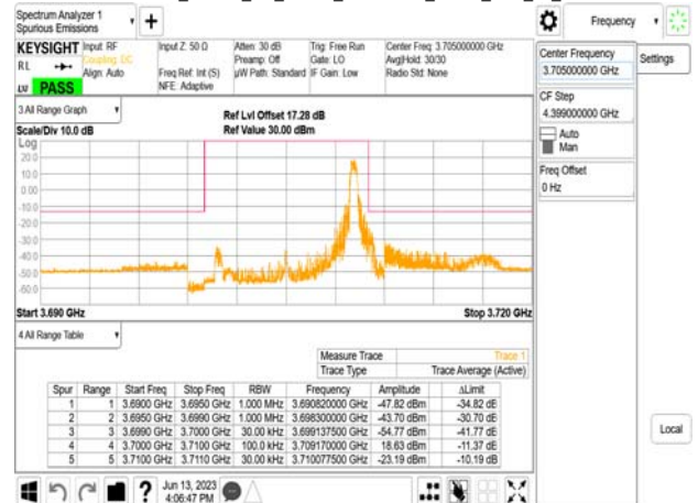
Band77-Part27_10MHz_CP_OFDM_SCS30kHz_QPSK_RB1_23_CH647000
