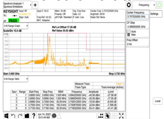
Band77-Part27_15MHz_CP_OFDM_SCS30kHz_QPSK_RB1_0_CH647168
