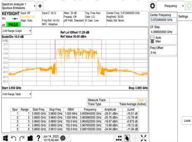
Band77-Part27_15MHz_CP_OFDM_SCS30kHz_QPSK_RB1_0_CH650500
