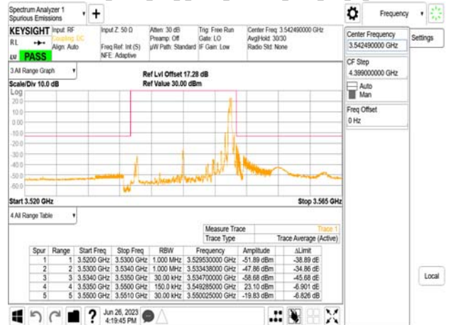
Band77-Part27_15MHz_DFT_s_OFDM_SCS30kHz_BPSK_RB1_37_CH647168
