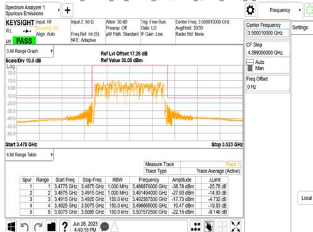
Band77-Part27_15Mhz_CP_OFDM_SCS30kHz_QPSK_RB38_0_CH63166
