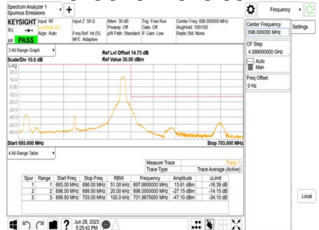
Band71_5MHz_CP_OFDM_SCS15kHz_QPSK_RB1_24_CH1319100
