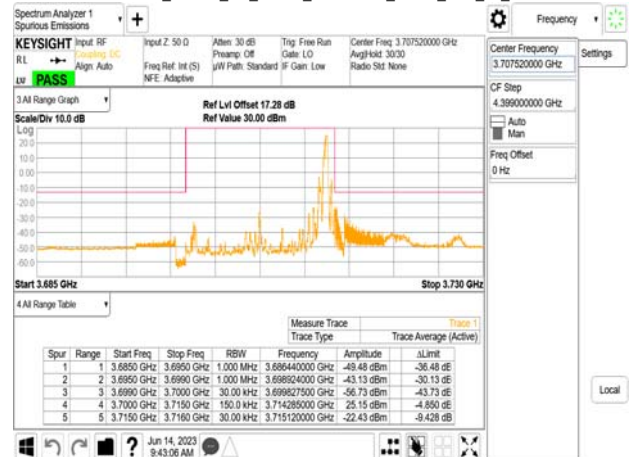
Band77-Part27_15MHz_CP_OFDM_SCS30kHz_QPSK_RB1_37_CH647168
