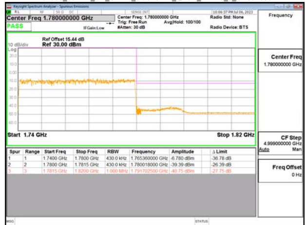
Band66_40MHz_CP_OFDM_SCS15kHz_QPSK_RB216_0_CH352000
