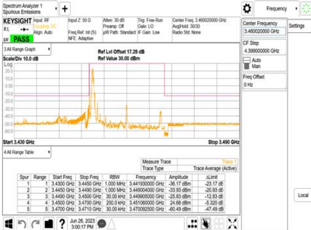
Band77-Part27_20MHz_DFT_s_OFDM_SCS30kHz_BPSK_RB1_0_CH630668
