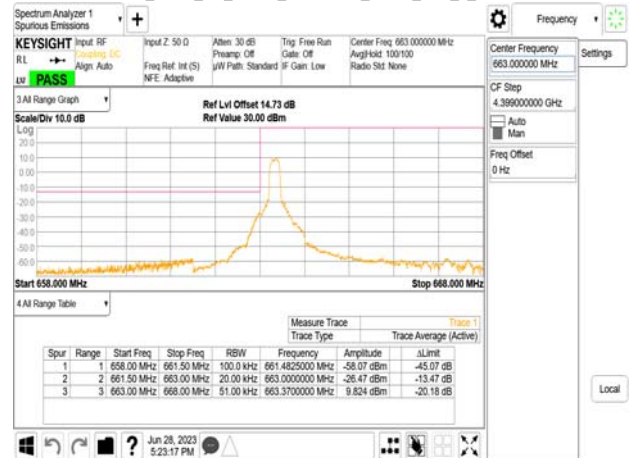
Band71_5MHz_CP_OFDM_SCS15kHz_QPSK_RB1_24_CH1319100
