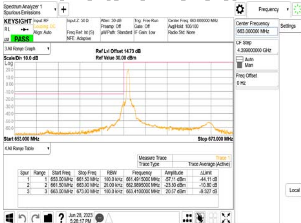
Band71_10MHz_DFT_s_OFDM_SCS15kHz_BPSK_RB1_0_CH133600
