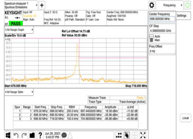
Band71_20MHz_CP_OFDM_SCS15kHz_QPSK_RB1_105_CH137600
