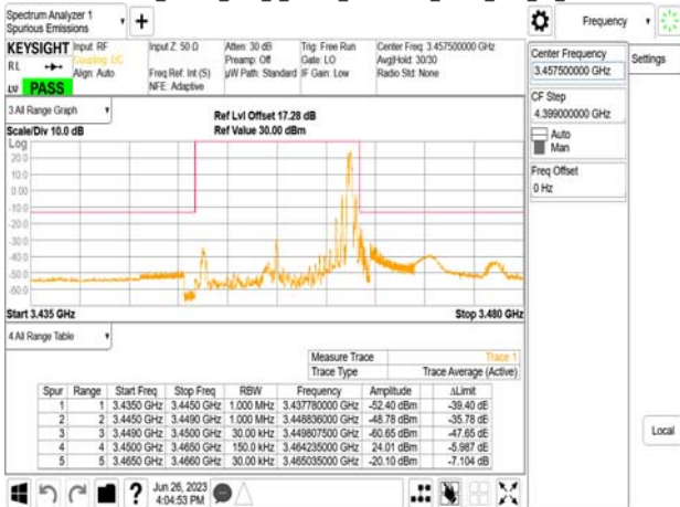
Band77-Part27_15MHz_DFT_s_OFDM_SCS30kHz_BPSK_RB1_37_CH630500
