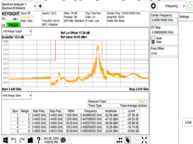
Band77-Part27_10MHz_DFT_s_OFDM_SCS30kHz_BPSK_RB1_23_CH630334
