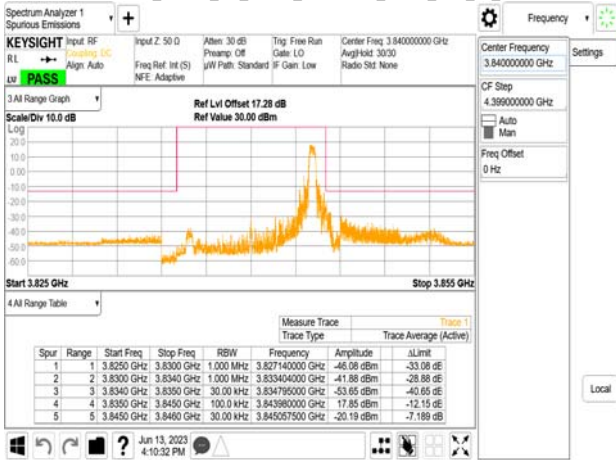
Band77-Part27_10MHz_CP_OFDM_SCS30kHz_QPSK_RB1_23_CH656000
