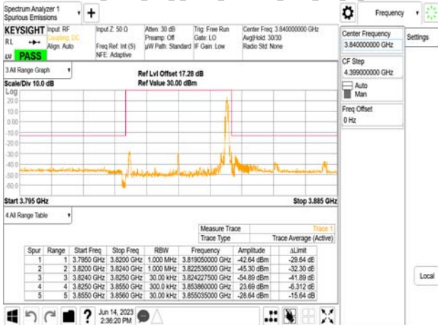
Band77-Part27_30MHz_DFT_s_OFDM_SCS30kHz_BPSK_RB1_77_CH64332
