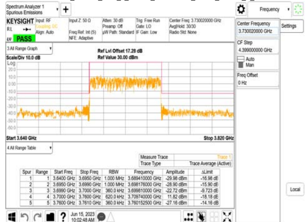
Band77-Part27_60MHz_DFT_s_OFDM_SCS30kHz_BPSK_RB162_0_CH648668
