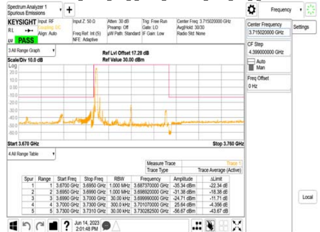
Band77-Part27_30MHz_DFT_s_OFDM_SCS30kHz_BPSK_RB1_0_CH647668
