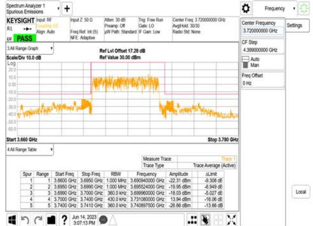
Band77-Part27_40MHz_DFT_s_OFDM_SCS30kHz_BPSK_RB100_0_CH648000
