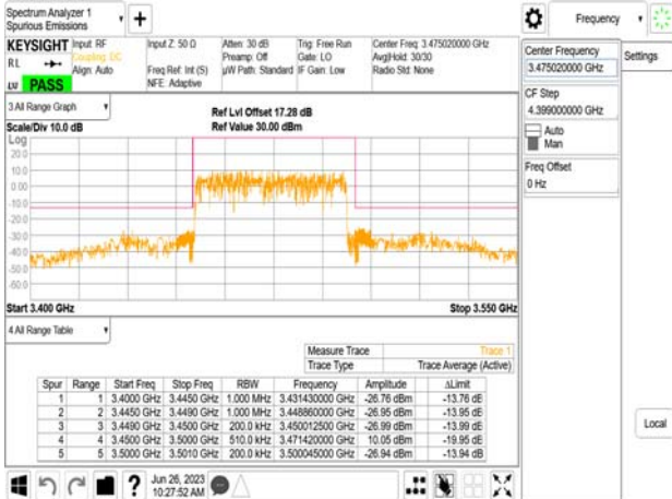
Band77-Part27_50MHz_DFT_s_OFDM_SCS30kHz_BPSK_RB128_0_CH631668
