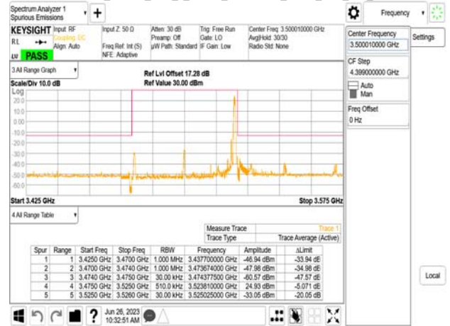
Band77-Part27_50MHz_DFT_s_OFDM_SCS30kHz_BPSK_RB1_132_CH635000
