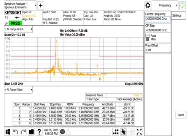
Band77-Part27_30MHz_DFT_s_OFDM_SCS30kHz_BPSK_RB1_0_CH635666
