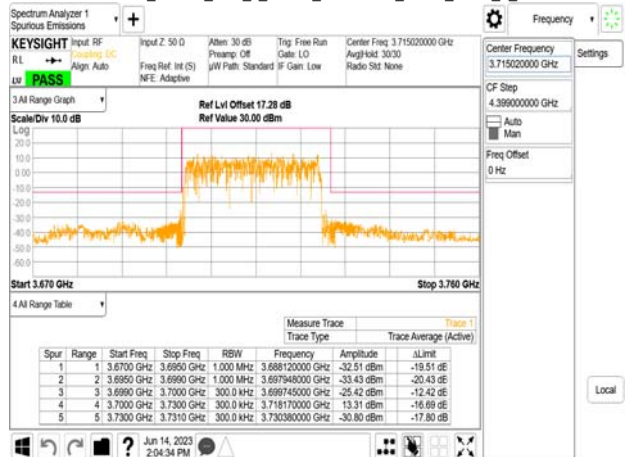
Band77-Part27_30MHz_DFT_s_OFDM_SCS30kHz_BPSK_RB75_0_CH647668
