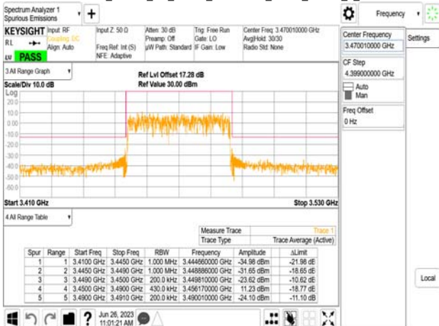
Band77-Part27_40MHz_CP_OFDM_SCS30kHz_QPSK_RB106_0_CH631334
