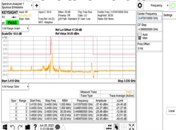
Band77-Part27_40MHz_DFT_s_OFDM_SCS30kHz_BPSK_RB1_0_CH631334
