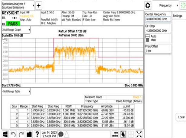
Band77-Part27_30MHz_DFT_s_OFDM_SCS30kHz_BPSK_RB75_0_CH64332
