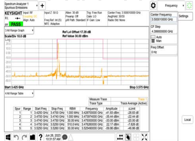
Band77-Part27_50MHz_DFT_s_OFDM_SCS30kHz_BPSK_RB1_0_CH635000
