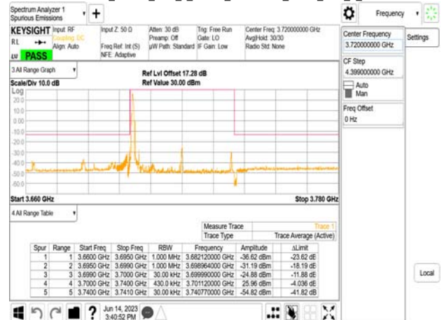
Band77-Part27_40MHz_DFT_s_OFDM_SCS30kHz_BPSK_RB1_0_CH648000
