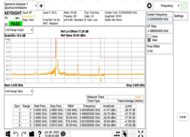
Band77-Part27_50MHz_DFT_s_OFDM_SCS30kHz_BPSK_RB1_0_CH648334
