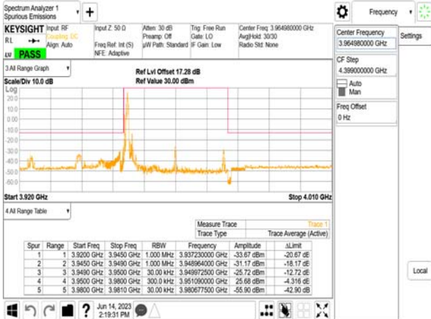
Band77-Part27_30MHz_DFT_s_OFDM_SCS30kHz_BPSK_RB1_77_CH613000
