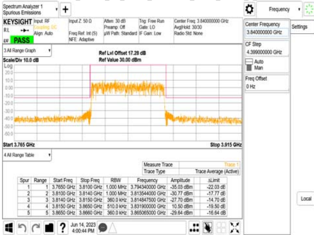
Band77-Part27_50MHz_CP_OFDM_SCS30kHz_OPSK_RB133_0_CH663666
