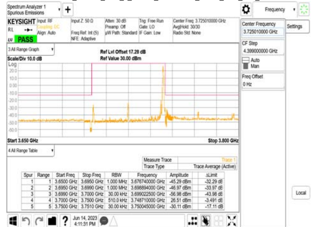
Band77-Part27_50MHz_DFT_s_OFDM_SCS30kHz_BPSK_RB1_132_CH648334
