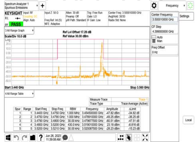
Band77-Part27_40MHz_DFT_s_OFDM_SCS30kHz_BPSK_RB1_105_CH635332
