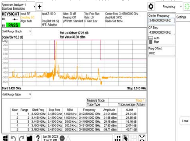
Band77-Part27_30MHz_CP_OFDM_SCS30kHz_QPSK_RB1_0_CH631000
