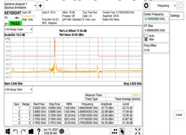
Band77-Part27_60MHz_DFT_s_OFDM_SCS30kHz_BPSK_RB1_0_CH648668
