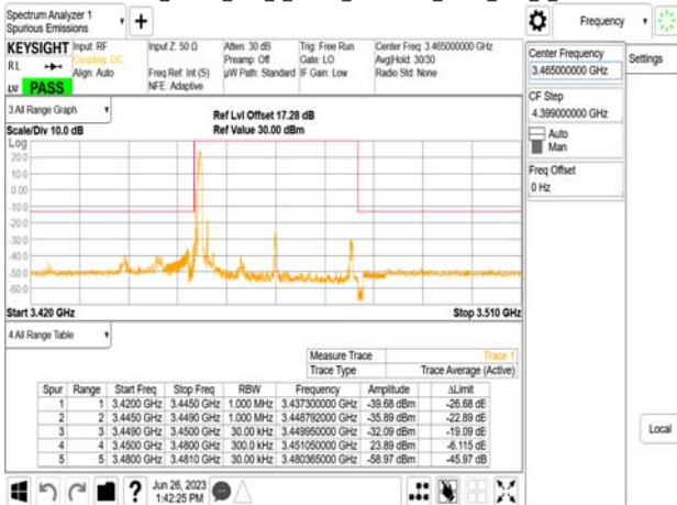
Band77-Part27_30MHz_DFT_s_OFDM_SCS30kHz_BPSK_RB1_0_CH631000
