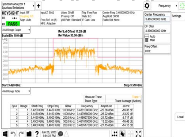
Band77-Part27_30MHz_DFT_s_OFDM_SCS30kHz_BPSK_RB75_0_CH631000
