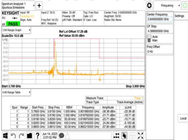
Band77-Part27_40MHz_CP_OFDM_SCS30kHz_QPSK_RB1_0_CH664000
