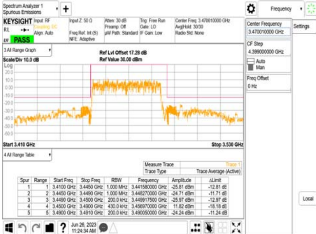
Band77-Part27_40MHz_DFT_s_OFDM_SCS30kHz_BPSK_RB100_0_CH631334
