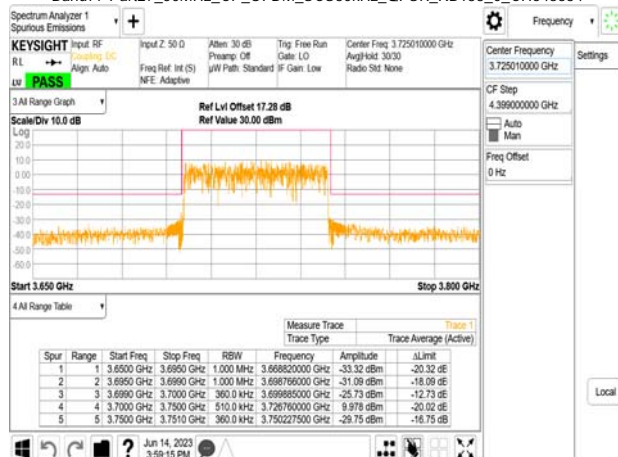
Band77-Part27_50MHz_CP_OFDM_SCS30kHz_QPSK_RB133_0_CH648334
