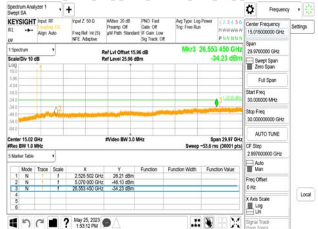
Band7_20MHz_DFT_s_OFDM_SCS15kHz_BPSK_RB1_1_CH512000
