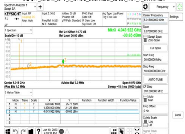
Band71_20MHz_DFT_s_OFDM_SCS15kHz_BPSK_RB1_1_CH137600
