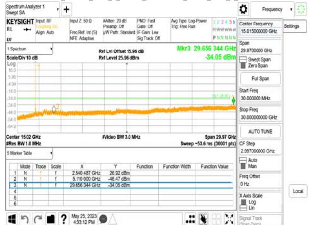
Band7_30MHz_DFT_s_OFDM_SCS15kHz_BPSK_RB1_1_CH511000
