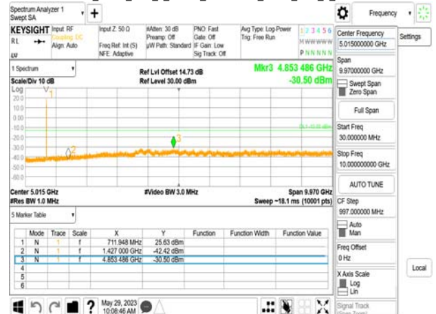
Band12_5MHz_DFT_s_OFDM_SCS15kHz_BPSK_RB1_1_CH142700
