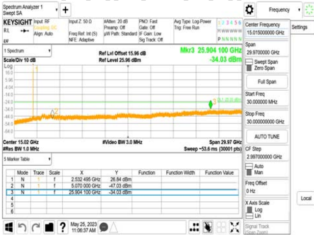
Band7_5MHz_DFT_s_OFDM_SCS15kHz_BPSK_RB1_1_CH513500
