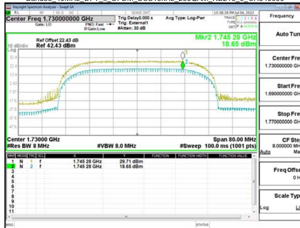
Band66_40MHz_DFT_s_OFDM_SCS15kHz_256QAM_RB216_0_CH349000
