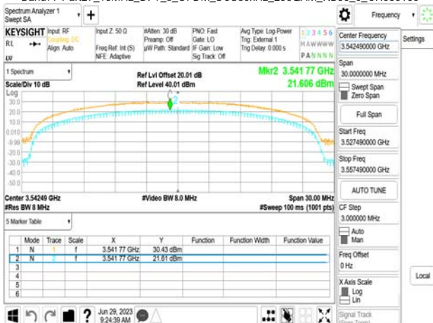
Band77-Part27_15MHz_DFT_s_OFDM_SCS30kHz_256QAM_RB36_0_CH636166
