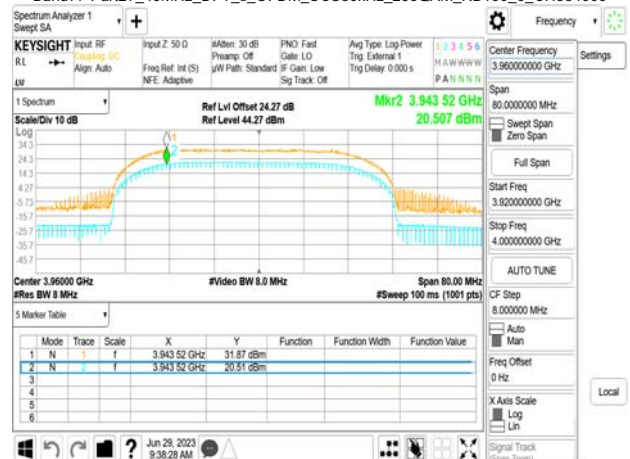
Band77-Part27_40MHz_DFT_s_OFDM_SCS30kHz_256QAM_RB100_0_CH664000
