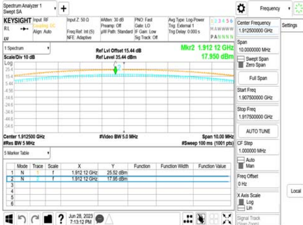
Band25_5MHz_DFT_s_OFDM_SCS15kHz_256QAM_RB25_0_CH382500
