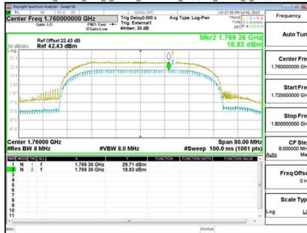
Band66_40MHz_DFT_s_OFDM_SCS15kHz_256QAM_RB216_0_CH352000
