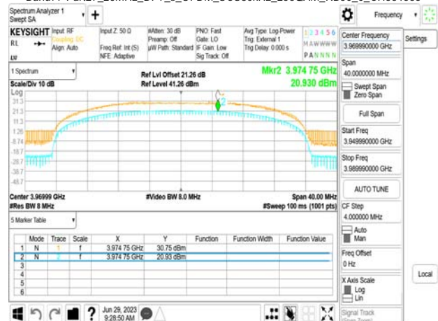
Band77-Part27_20MHz_DFT_s_OFDM_SCS30kHz_256QAM_RB50_0_CH664666
