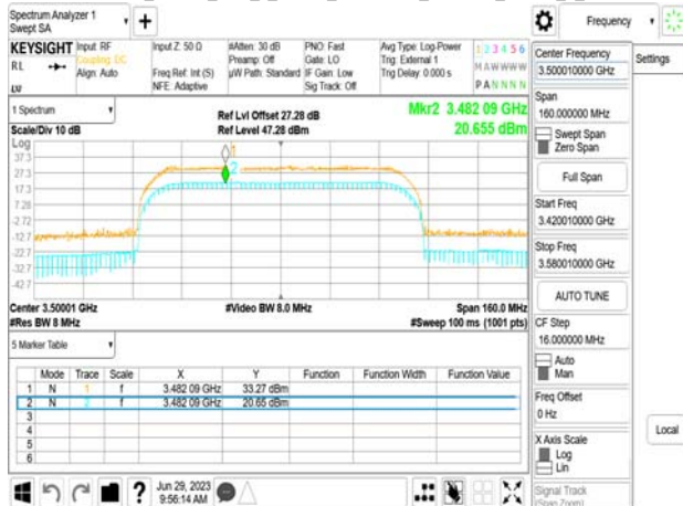
Band77-Part27_80MHz_DFT_s_OFDM_SCS30kHz_256QAM_RB216_0_CH634000
