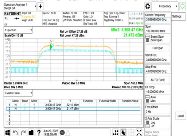
Band77-Part27_80MHz_DFT_s_OFDM_SCS30kHz_256QAM_RB216_0_CH662666
