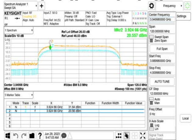
Band77-Part27_60MHz_DFT_s_OFDM_SCS30kHz_256QAM_RB162_0_CH663332
