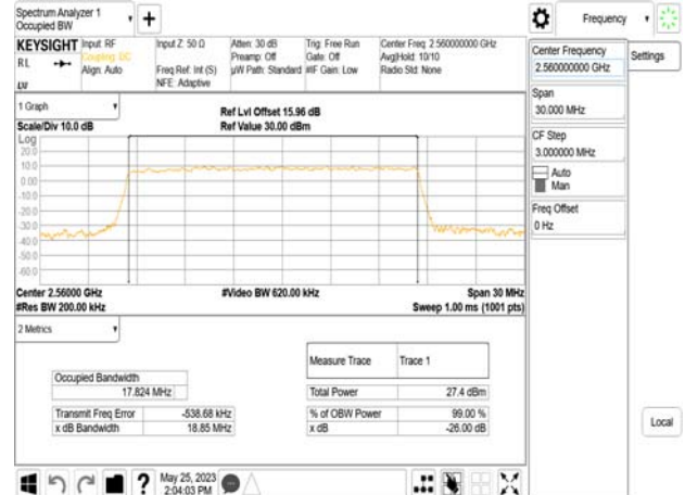
Band7_20MHz_DFT_s_OFDM_SCS15kHz_256QAM_RB100_0_CH512000
