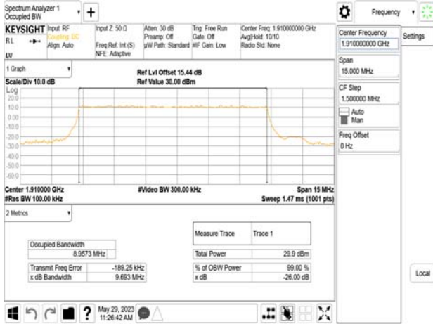
Band25_10MHz_DFT_s_OFDM_SCS15kHz_QPSK_RB50_0_CH382000
