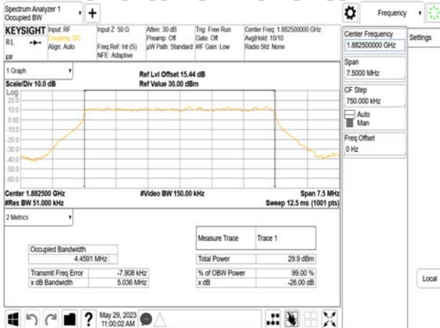
Band25_5MHz_DFT_s_OFDM_SCS15kHz_BPSK_RB25_0_CH382500
