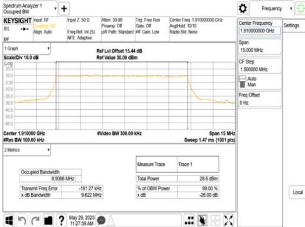
Band25_10MHz_DFT_s_OFDM_SCS15kHz_64QAM_RB50_0_CH382000
