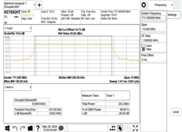
Band12_10MHz_DFT_s_OFDM_SCS15kHz_64QAM_RB50_0_CH142200
