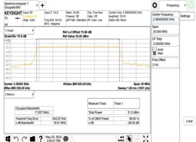
Band7_20MHz_DFT_s_OFDM_SCS15kHz_BPSK_RB100_0_CH512000
