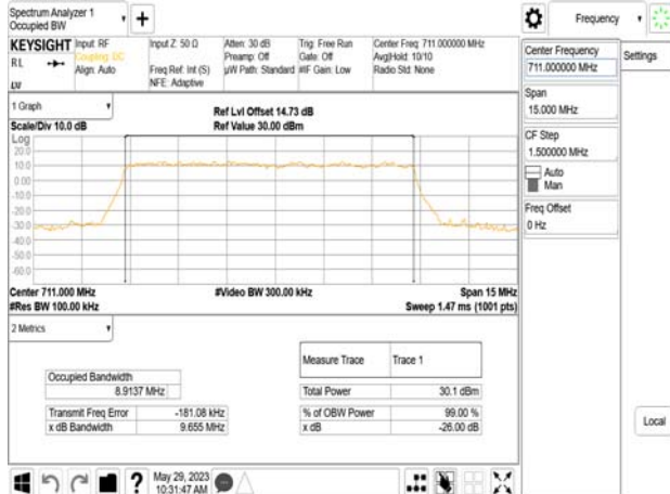
Band12_10MHz_DFT_s_OFDM_SCS15kHz_BPSK_RB50_0_CH142200
