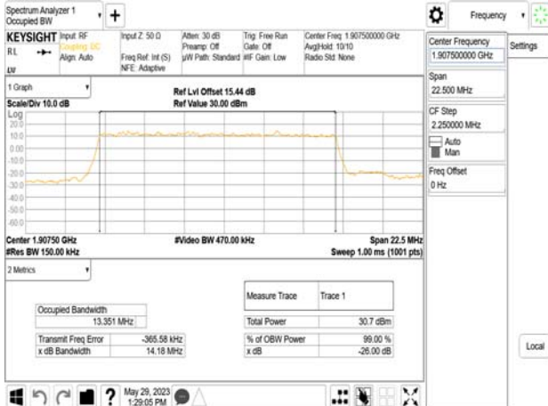
Band25_15MHz_DFT_s_OFDM_SCS15kHz_BPSK_RB75_0_CH381500
