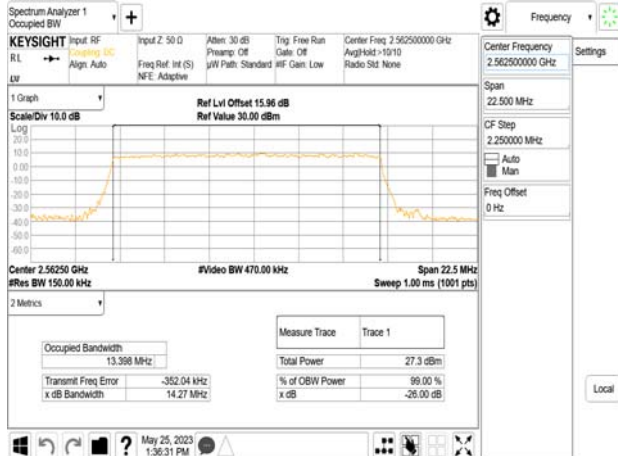
Band7_15MHz_DFT_s_OFDM_SCS15kHz_256QAM_RB75_0_CH512500
