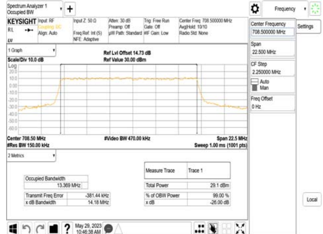
Band12_15MHz_DFT_s_OFDM_SCS15kHz_16QAM_RB75_0_CH141700
