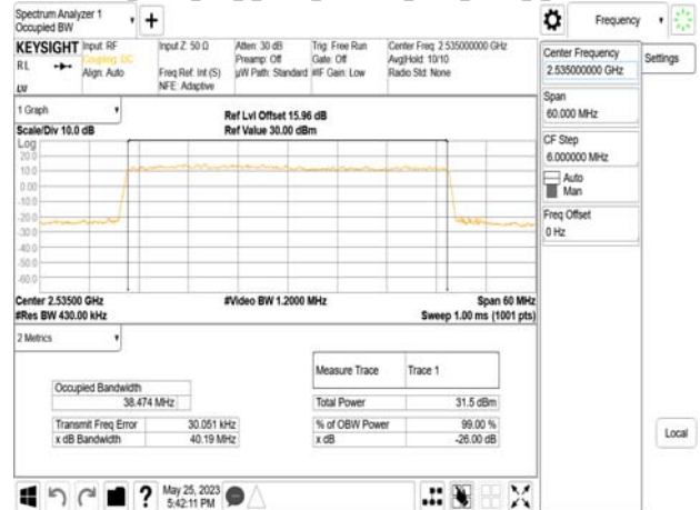
Band7_40MHz_DFT_s_OFDM_SCS15kHz_QPSK_RB216_0_CH510000
