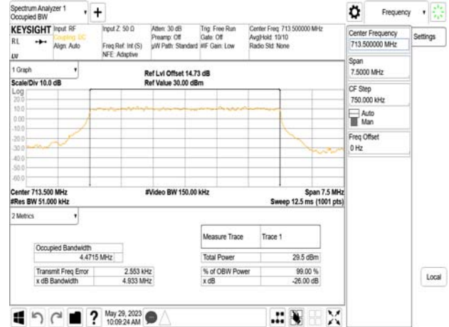
Band12_5MHz_DFT_s_OFDM_SCS15kHz_BPSK_RB25_0_CH142700
