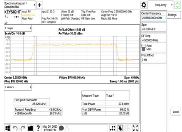
Band7_30MHz_DFT_s_OFDM_SCS15kHz_256QAM_RB160_0_CH511000
