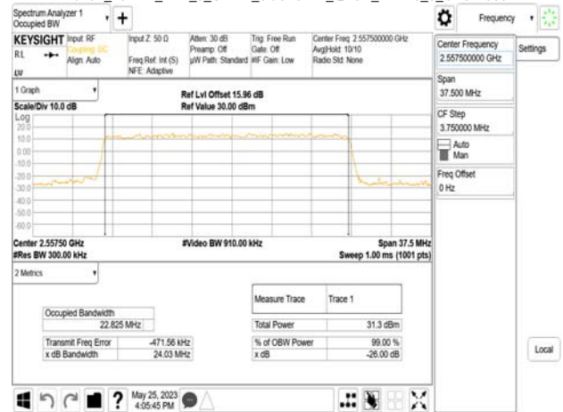
Band7_25MHz_DFT_s_OFDM_SCS15kHz_QPSK_RB128_0_CH511500
