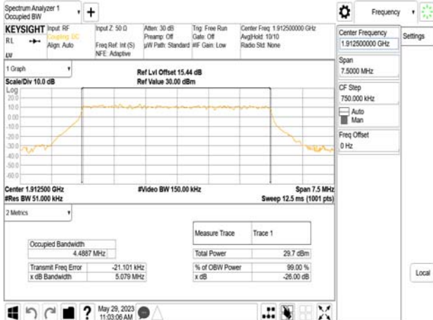
Band25_5MHz_DFT_s_OFDM_SCS15kHz_BPSK_RB25_0_CH382500
