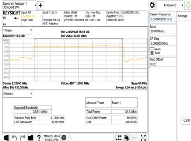
Band7_40MHz_DFT_s_OFDM_SCS15kHz_BPSK_RB216_0_CH510000
