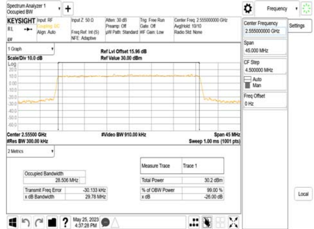
Band7_30MHz_DFT_s_OFDM_SCS15kHz_16QAM_RB160_0_CH511000
