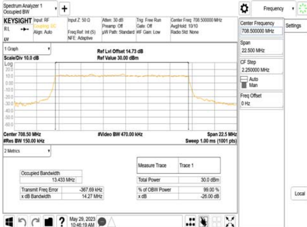
Band12_15MHz_DFT_s_OFDM_SCS15kHz_QPSK_RB75_0_CH141700
