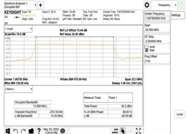
Band25_15MHz_DFT_s_OFDM_SCS15kHz_QPSK_RB75_0_CH381500
