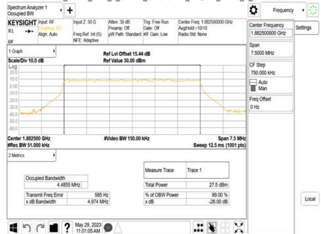
Band25_5MHz_DFT_s_OFDM_SCS15kHz_64QAM_RB25_0_CH382500
