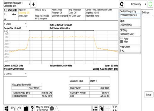
Band7_20MHz_DFT_s_OFDM_SCS15kHz_16QAM_RB100_0_CH512000
