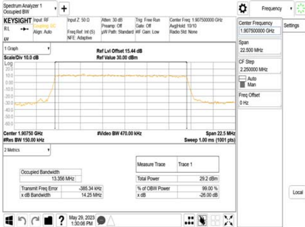
Band25_15MHz_DFT_s_OFDM_SCS15kHz_16QAM_RB75_0_CH381500
