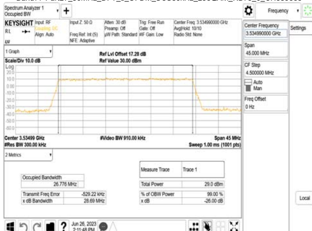
Band77-Part27_30MHz_DFT_s_OFDM_SCS30kHz_256QAM_RB75_0_CH635666
