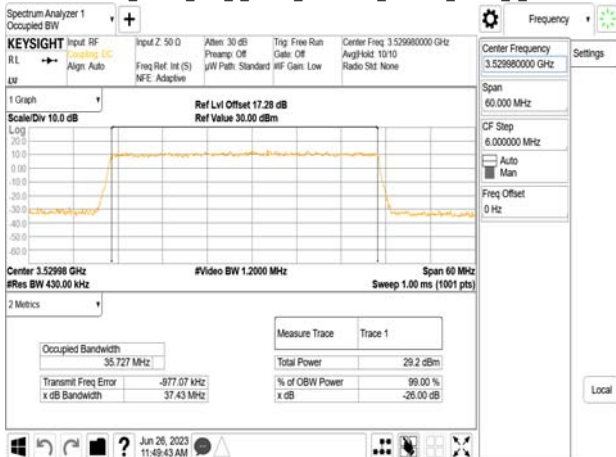
Band77-Part27_40MHz_DFT_s_OFDM_SCS30kHz_256QAM_RB100_0_CH635332
