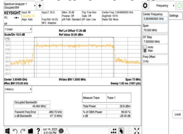
Band77-Part27_50MHz_DFT_s_OFDM_SCS30kHz_16QAM_RB128_0_CH663666
