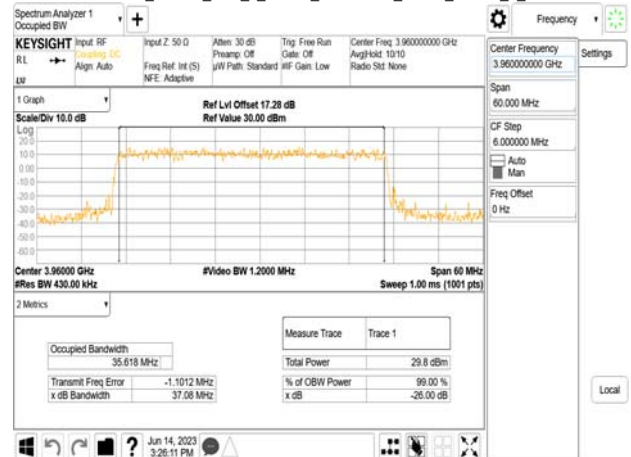
Band77-Part27_40MHz_DFT_s_OFDM_SCS30kHz_QPSK_RB100_0_CH664000
