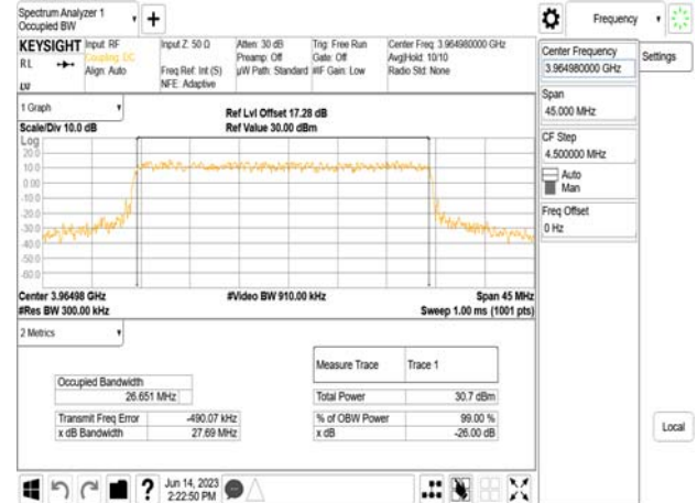
Band77-Part27_30MHz_DFT_s_OFDM_SCS30kHz_QPSK_RB75_0_CH664332
