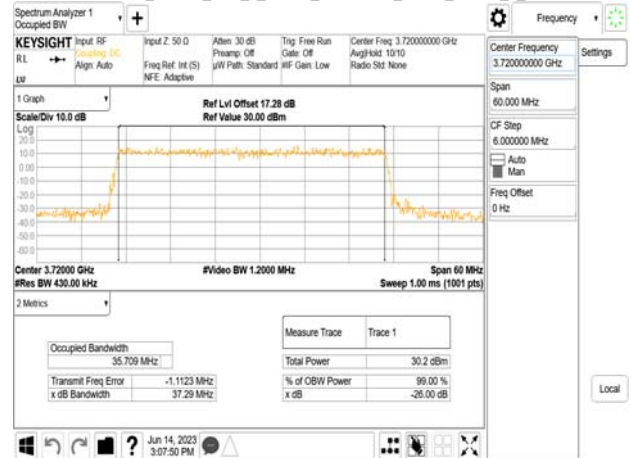
Band77-Part27_40MHz_DFT_s_OFDM_SCS30kHz_QPSK_RB100_0_CH656000
