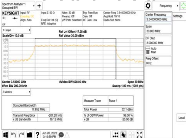
Band77-Part27_20MHz_DFT_s_OFDM_SCS30kHz_QPSK_RB50_0_CH636000
