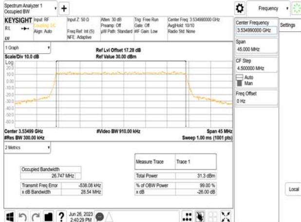
Band77-Part27_30MHz_DFT_s_OFDM_SCS30kHz_16QAM_RB75_0_CH635666
