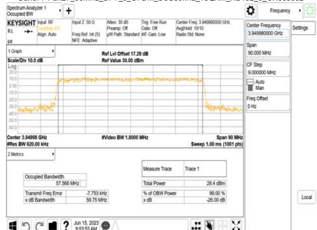
Band77-Part27_60MHz_DFT_s_OFDM_SCS30kHz_16QAM_RB162_0_CH663332
