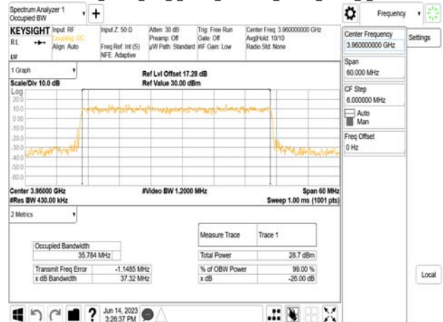
Band77-Part27_40MHz_DFT_s_OFDM_SCS30kHz_16QAM_RB100_0_CH664000
