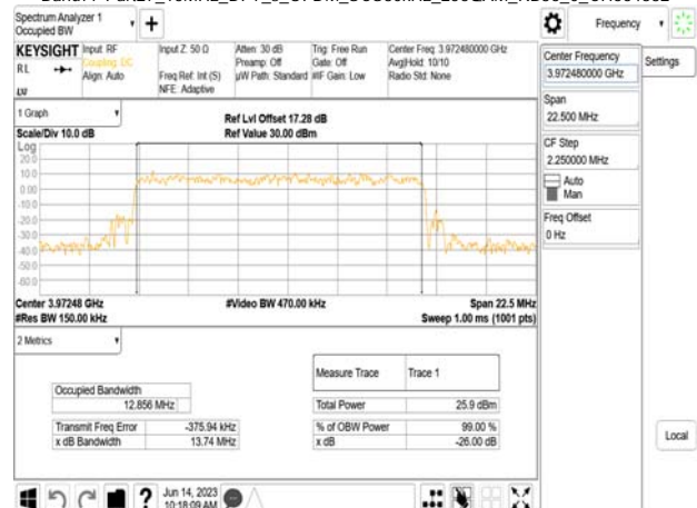
Band77-Part27_15MHz_DFT_s_OFDM_SCS30kHz_256QAM_RB36_0_CH664832
