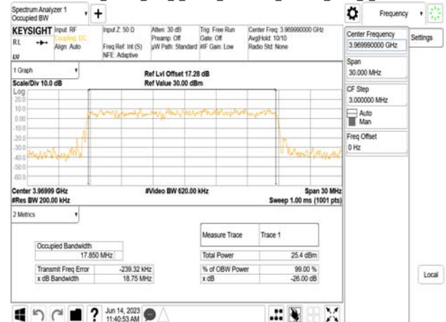
Band77-Part27_20MHz_DFT_s_OFDM_SCS30kHz_256QAM_RB50_0_CH664666
