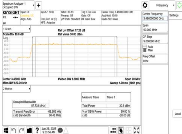
Band77-Part27_60MHz_DFT_s_OFDM_SCS30kHz_BPSK_RB162_0_CH633334
