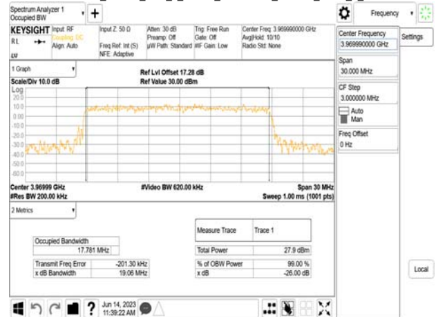
Band77-Part27_20MHz_DFT_s_OFDM_SCS30kHz_16QAM_RB50_0_CH664666
