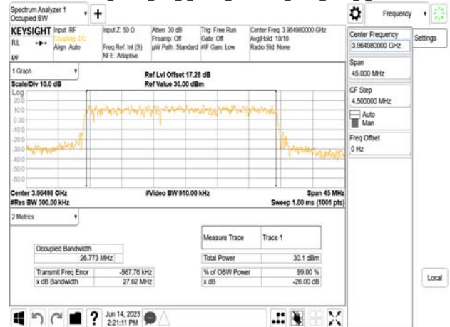
Band77-Part27_30MHz_DFT_s_OFDM_SCS30kHz_BPSK_RB75_0_CH664332
