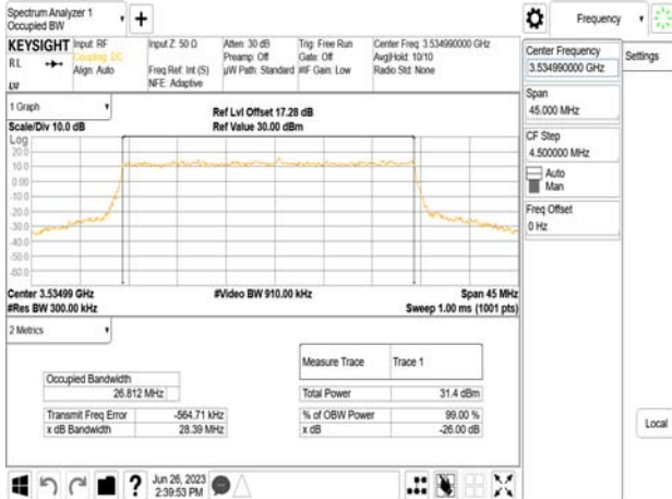
Band77-Part27_30MHz_DFT_s_OFDM_SCS30kHz_QPSK_RB75_0_CH635666
