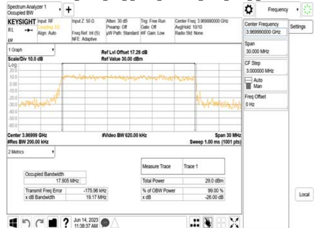
Band77-Part27_20MHz_DFT_s_OFDM_SCS30kHz_QPSK_RB50_0_CH664666
