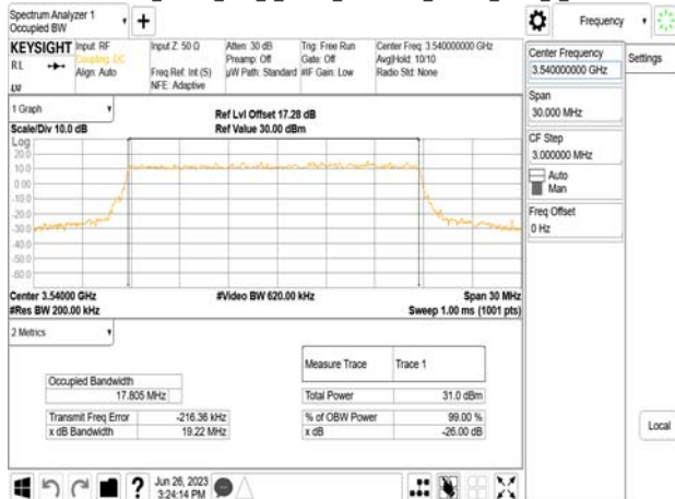
Band77-Part27_20MHz_DFT_s_OFDM_SCS30kHz_64QAM_RB50_0_CH636000
