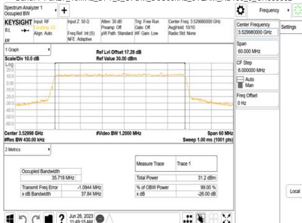
Band77-Part27_40MHz_DFT_s_OFDM_SCS30kHz_64QAM_RB100_0_CH635332
