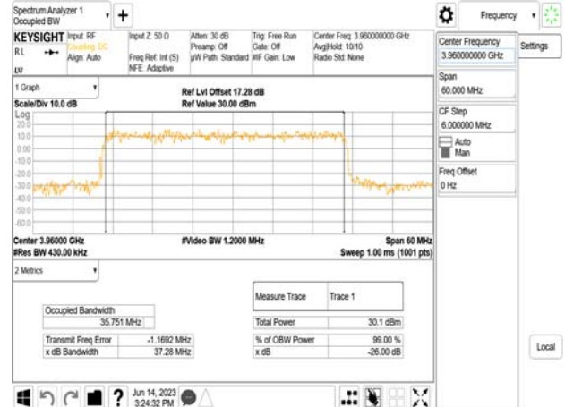
Band77-Part27_40MHz_DFT_s_OFDM_SCS30kHz_BPSK_RB100_0_CH664000
