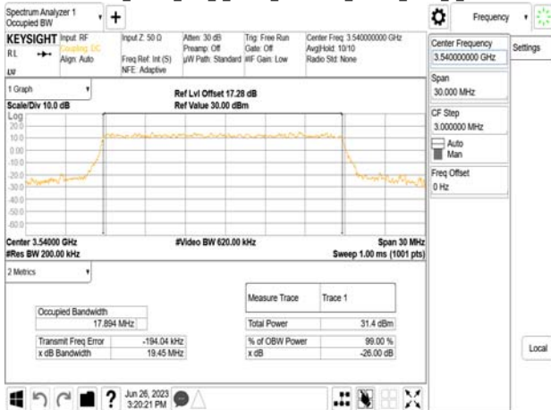
Band77-Part27_20MHz_DFT_s_OFDM_SCS30kHz_16QAM_RB50_0_CH636000
