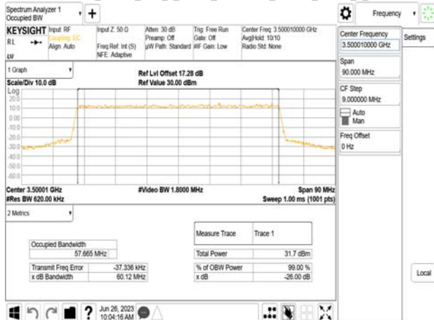
Band77-Part27_60MHz_DFT_s_OFDM_SCS30kHz_16QAM_RB162_0_CH634666
