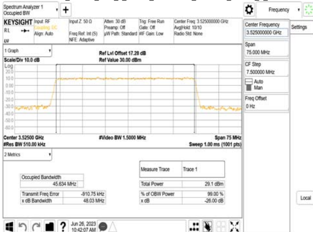
Band77-Part27_50MHz_DFT_s_OFDM_SCS30kHz_256QAM_RB128_0_CH635000
