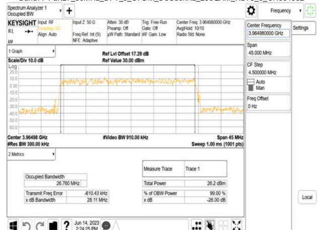
Band77-Part27_30MHz_DFT_s_OFDM_SCS30kHz_256QAM_RB75_0_CH664332
