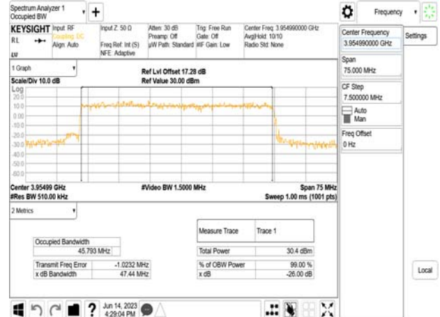
Band77-Part27_50MHz_DFT_s_OFDM_SCS30kHz_BPSK_RB128_0_CH663666
