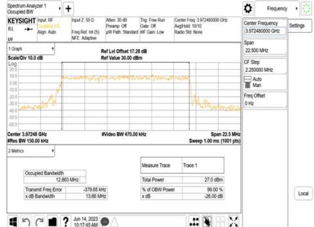
Band77-Part27_15MHz_DFT_s_OFDM_SCS30kHz_64QAM_RB36_0_CH664832
