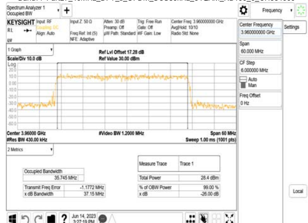
Band77-Part27_40MHz_DFT_s_OFDM_SCS30kHz_64QAM_RB100_0_CH664000
