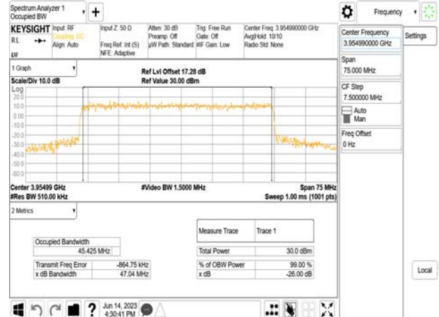
Band77-Part27_50MHz_DFT_s_OFDM_SCS30kHz_QPSK_RB128_0_CH663666
