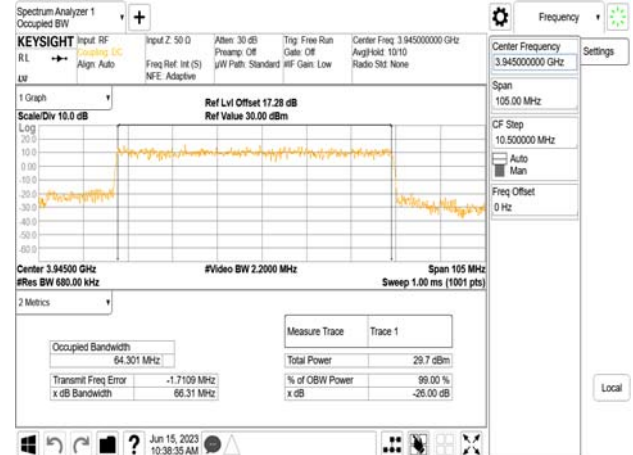
Band77-Part27_70MHz_DFT_s_OFDM_SCS30kHz_BPSK_RB180_0_CH663000
