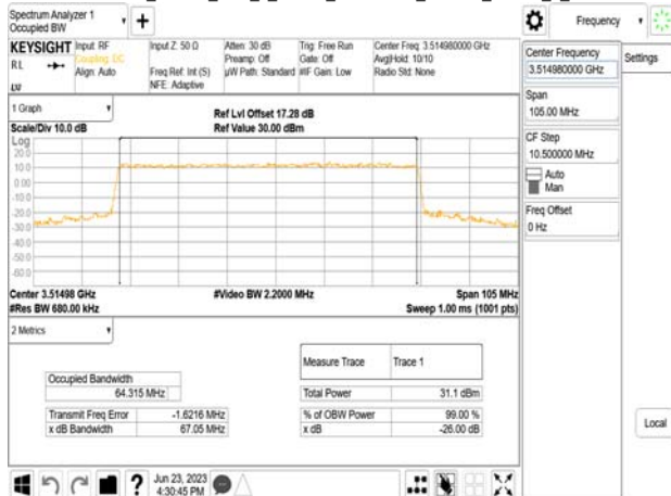
Band77-Part27_70MHz_DFT_s_OFDM_SCS30kHz_16QAM_RB180_0_CH634332
