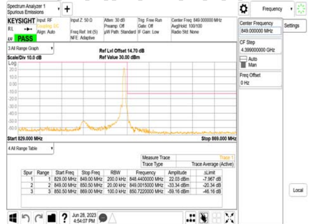
Band5_20MHz_DFT_s_OFDM_SCS15kHz_BPSK_RB100_0_CH166800
