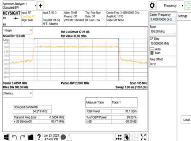
Band77-Part27_70MHz_DFT_s_OFDM_SCS30kHz_16QAM_RB180_0_CH633334
