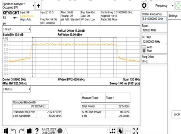
Band77-Part27_80MHz_DFT_s_OFDM_SCS30kHz_QPSK_RB216_0_CH634000
