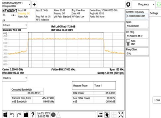
Band77-Part27_90MHz_DFT_s_OFDM_SCS30kHz_QPSK_RB243_0_CH633666
