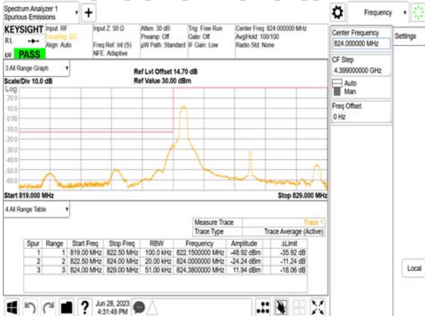
Band5_5MHz_CP_OFDM_SCS15kHz_OPSK_RB1_24_CH169300
