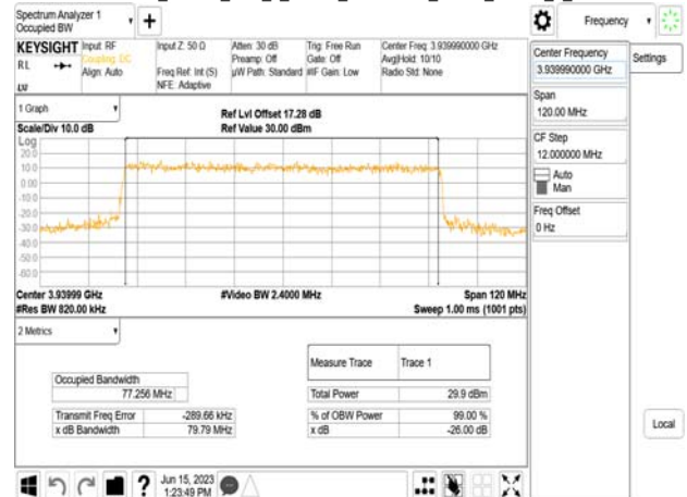
Band77-Part27_80MHz_DFT_s_OFDM_SCS30kHz_QPSK_RB216_0_CH662666
