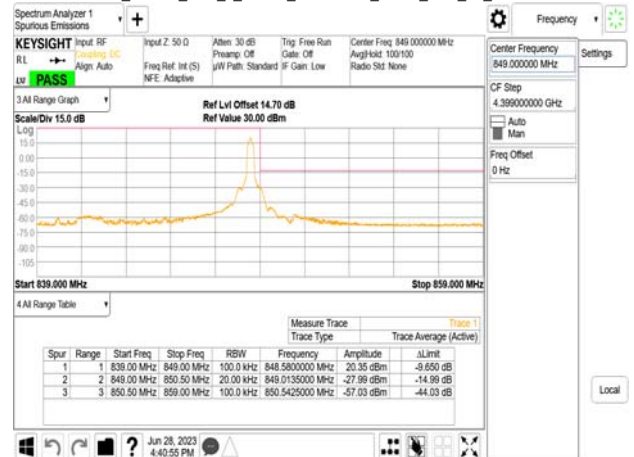
Band5_10MHz_DFT_s_OFDM_SCS15kHz_BPSK_RB1_51_CH168800
