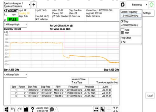
Band2_15MHz_CP_OFDM_SCS15kHz_QPSK_RB79_0_CH380500
