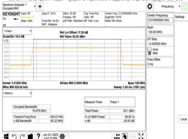
Band77-Part27_80MHz_DFT_s_OFDM_SCS30kHz_256QAM_RB216_0_CH634000
