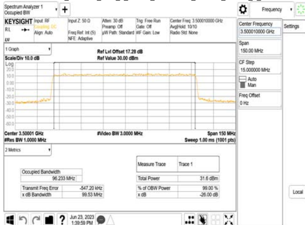
Band77-Part27_100MHz_DFT_s_OFDM_SCS30kHz_16QAM_RB270_0_CH633334
