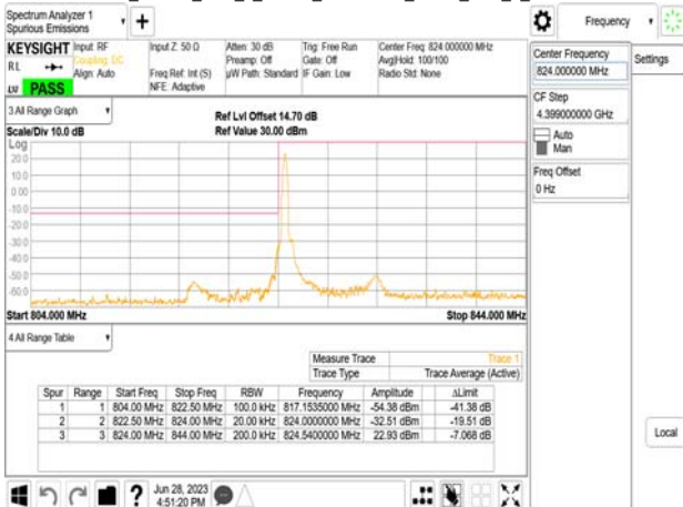
Band5_20MHz_DFT_s_OFDM_SCS15kHz_BPSK_RB1_0_CH166800
