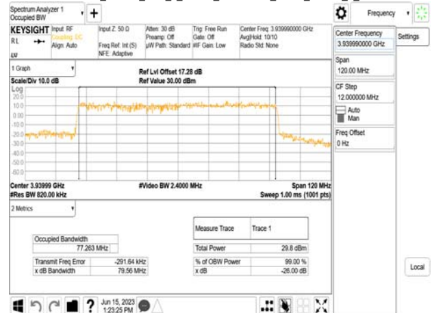
Band77-Part27_80MHz_DFT_s_OFDM_SCS30kHz_BPSK_RB216_0_CH662666
