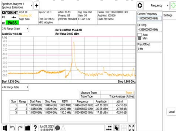
Band2_15MHz_CP_OFDM_SCS15kHz_QPSK_RB1_0_CH371500
