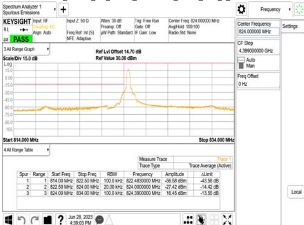
Band5_10MHz_CP_OFDM_SCS15kHz_QPSK_RB1_0_CH165800
