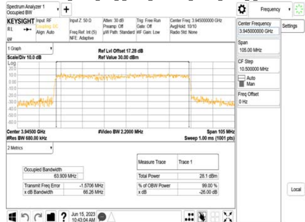
Band77-Part27_70MHz_DFT_s_OFDM_SCS30kHz_16QAM_RB180_0_CH663000
