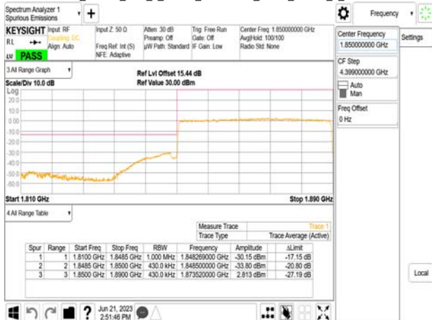
Band25_40MHz_DFT_s_OFDM_SCS15kHz_BPSK_RB216_0_CH374000
