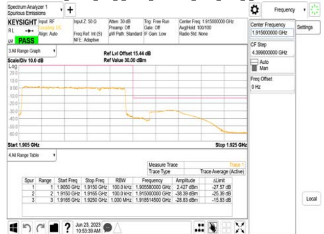
Band25_10MHz_DFT_s_OFDM_SCS15kHz_BPSK_RB50_0_CH382000
