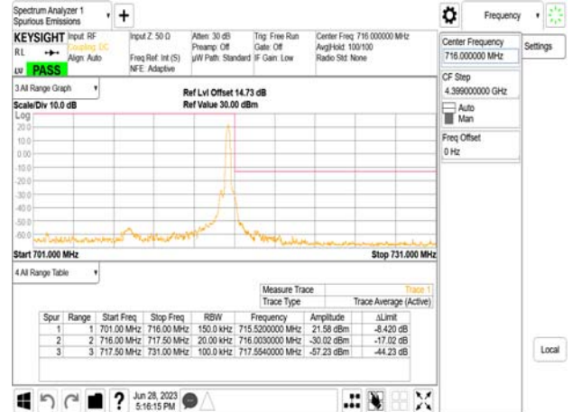
Band12_15MHz_DFT_s_OFDM_SCS15kHz_BPSK_RB1_78_CH141700
