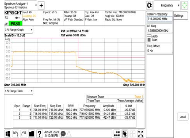
Band12_15MHz_DFT_s_OFDM_SCS15kHz_BPSK_RB1_0_CH141300
