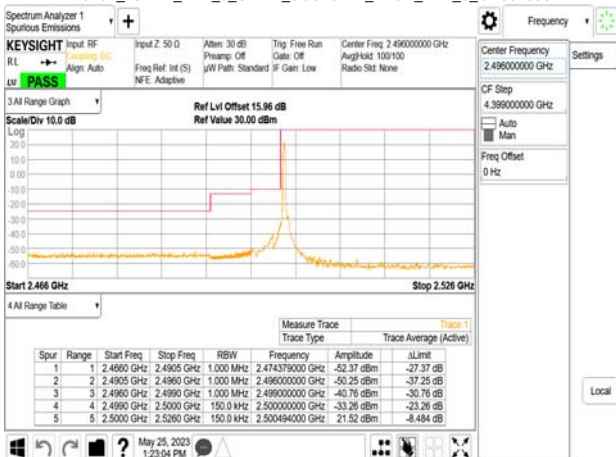
Band7_15MHz_DFT_s_OFDM_SCS15kHz_BPSK_RB1_0_CH501500
