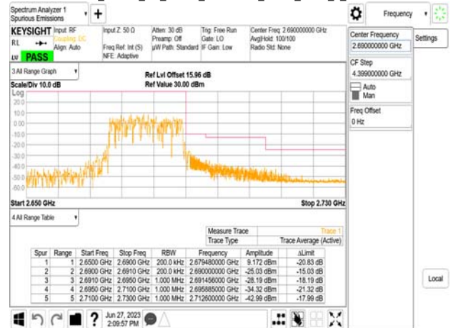
Band41_20MHz_CP_OFDM_SCS30kHz_QPSK_RB51_0_CH535998
