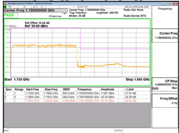
Band66_25MHz_CP_OFDM_SCS15kHz_QPSK_RB1_0_CH344500
