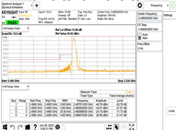
Band41_100MHz_DFT_s_OFDM_SCS30kHz_BPSK_RB1_0_CH509202
