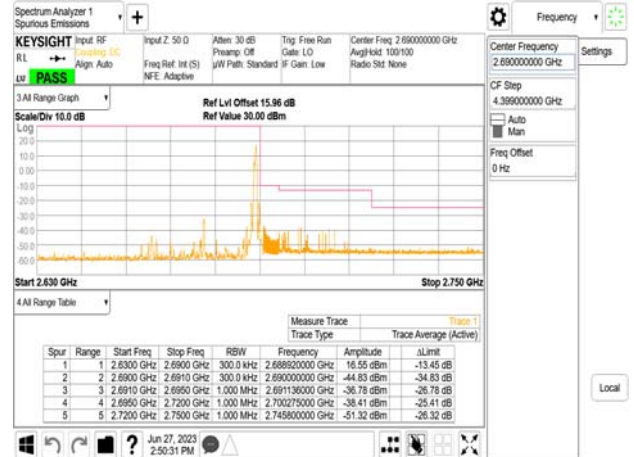
Band41_30MHz_CP_OFDM_SCS30kHz_QPSK_RB1_77_CH534996
