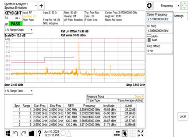
Band38_40MHz_DFT_s_OFDM_SCS30kHz_BPSK_RB1_105_CH520000
