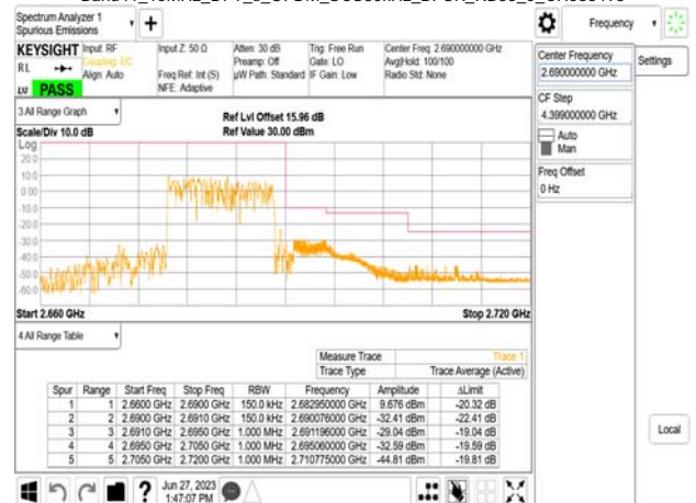
Band41_15MHz_DFT_s_OFDM_SCS30kHz_BPSK_RB36_0_CH536496
