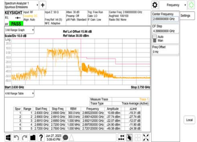
Band41_30MHz_CP_OFDM_SCS30kHz_QPSK_RB1_0_CH502200
