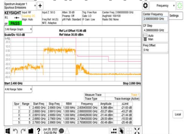
Band41_100MHz_DFT_s_OFDM_SCS30kHz_BPSK_RB270_0_CH528000
