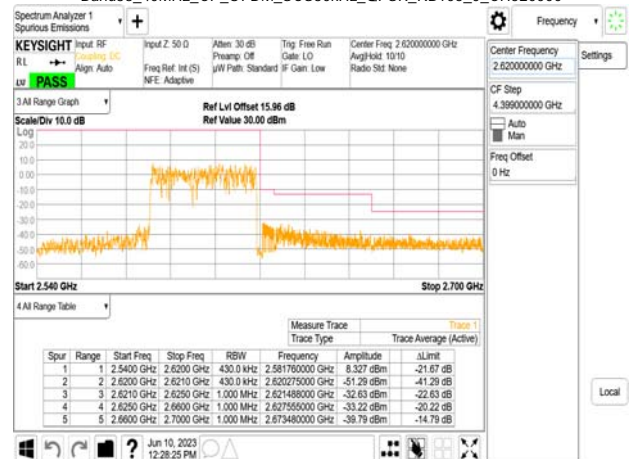
Band38_40MHz_CP_OFDM_SCS30kHz_QPSK_RB106_0_CH520000
