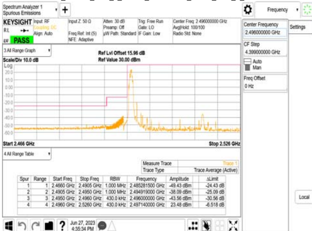
Band41_40MHz_DFT_s_OFDM_SCS30kHz_BPSK_RB1_0_CH503202
