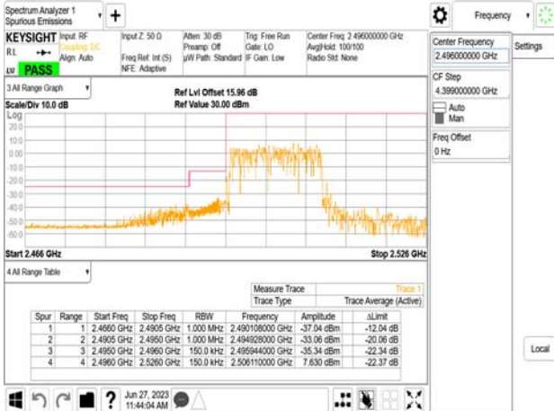
Band41_15MHz_CP_OFDM_SCS30kHz_QPSK_RB38_0_CH500700
