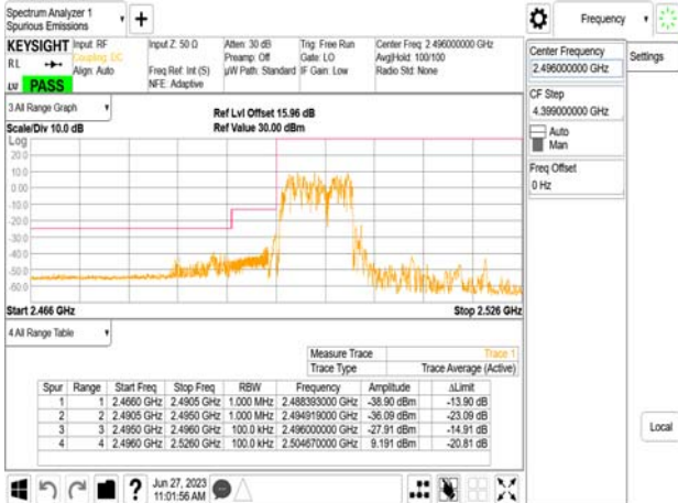
Band41_10MHz_DFT_s_OFDM_SCS30kHz_BPSK_RB24_0_CH500202
