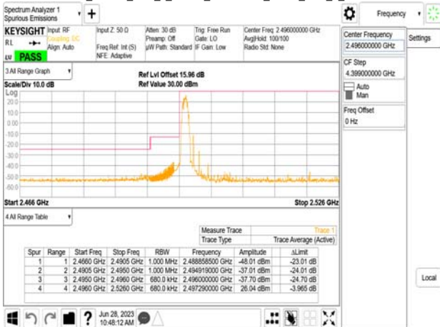
Band41_70MHz_DFT_s_OFDM_SCS30kHz_BPSK_RB1_0_CH506202
