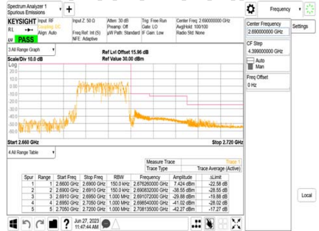
Band41_20MHz_DFT_s_OFDM_SCS30kHz_BPSK_RB1_0_CH510204
