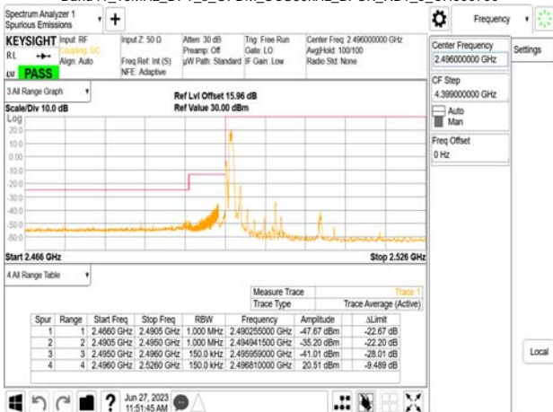
Band41_15MHz_DFT_s_OFDM_SCS30kHz_BPSK_RB1_0_CH500700
