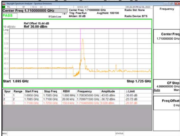
Band66_15MHz_CP_OFDM_SCS15kHz_OPSK_RB1_78_CH34500
