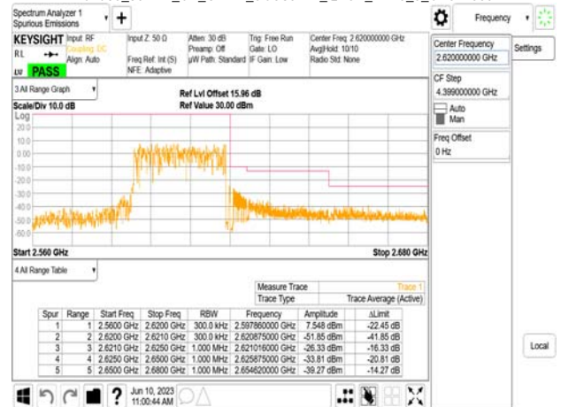
Band38_40MHz_DFT_s_OFDM_SCS30kHz_BPSK_RB1_0_CH518000
