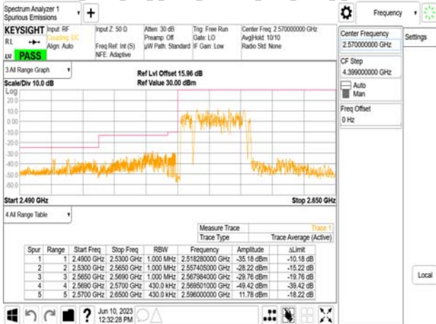
Band38_40MHz_DFT_s_OFDM_SCS30kHz_BPSK_RB100_0_CH520000
