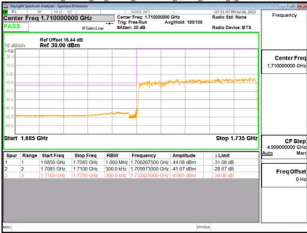
Band66_25MHz_CP_OFDM_SCS15kHz_OPKS_RB133_0_CH353500
