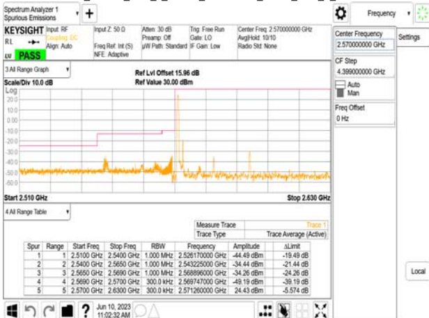
Band38_30MHz_DFT_s_OFDM_SCS30kHz_BPSK_RB1_0_CH517000
