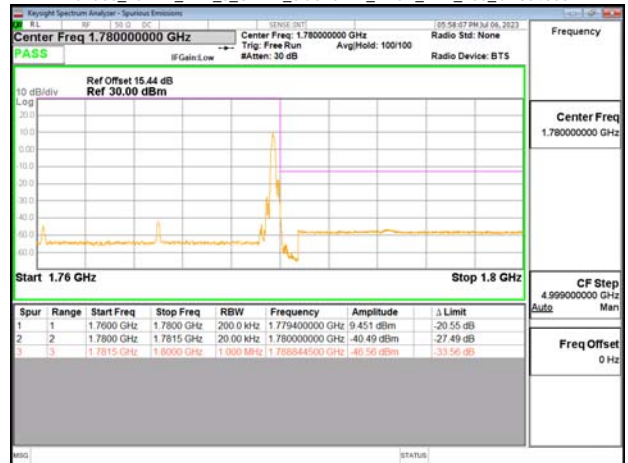
Band66_20MHz_DFT_s_OFDM_SCS15kHz_BPSK_RB1_105_CH34000
