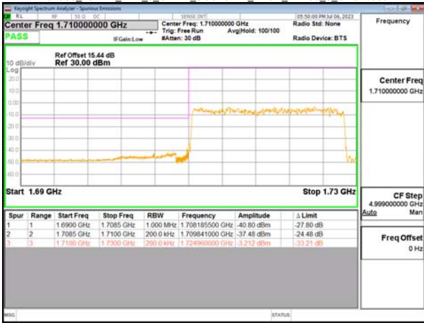
Band66_20MHz_DFT_s_OFDM_SCS15kHz_BPSK_RB100_0_CH344000
