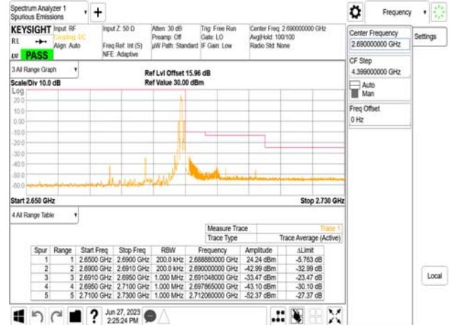
Band41_20MHz_DFT_s_OFDM_SCS30kHz_BPSK_RB1_50_CH535998
