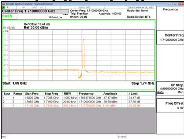
Band66_30MHz_DFT_s_OFDM_SCS15kHz_BPSK_RB1_0_CH345000
