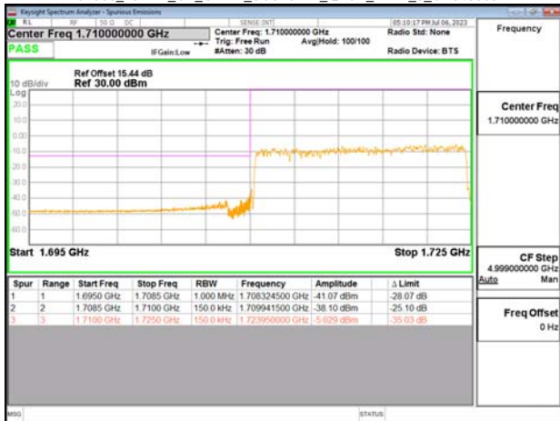
Band66_15MHz_CP_OFDM_SCS15kHz_OPSK_RB79_0_CH343500
