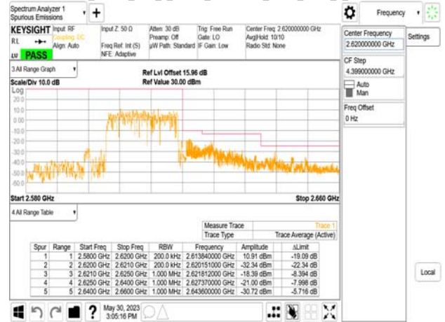
Band38_20MHz_CP_OFDM_SCS30kHz_QPSK_RB1_0_CH516000
