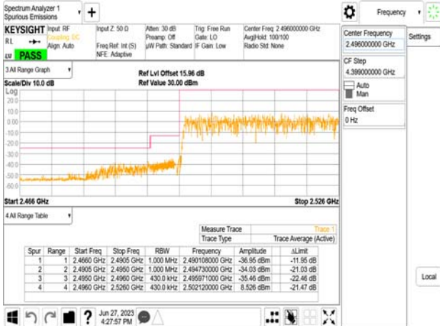
Band41_40MHz_CP_OFDM_SCS30kHz_QPSK_RB106_0_CH503202
