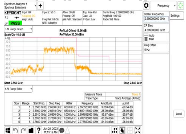
Band41_70MHz_DFT_s_OFDM_SCS30kHz_BPSK_RB180_0_CH531000
