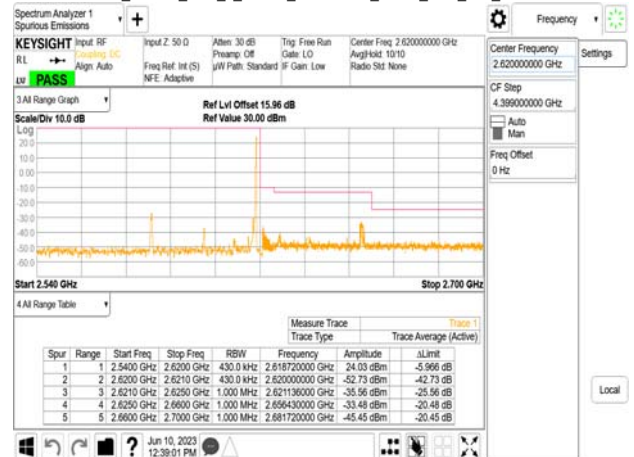
Band38_40MHz_DFT_s_OFDM_SCS30kHz_BPSK_RB1_105_CH520000
