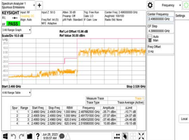
Band41_60MHz_DFT_s_OFDM_SCS30kHz_BPSK_RB162_0_CH505200
