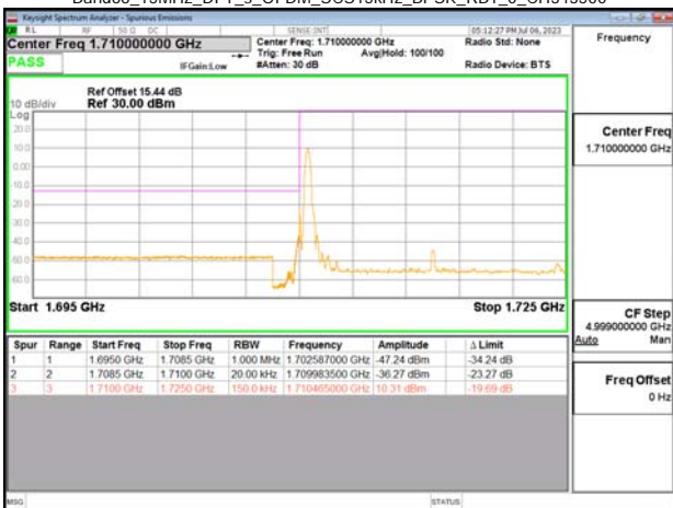
Band66_15MHz_DFT_s_OFDM_SCS15kHz_BPSK_RB1_0_CH343500
