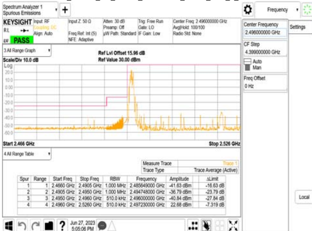
Band41_50MHz_CP_OFDM_SCS30kHz_QPSK_RB1_0_CH504204
