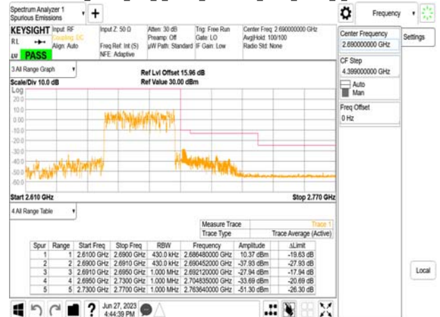
Band41_40MHz_DFT_s_OFDM_SCS30kHz_BPSK_RB100_0_CH534000
