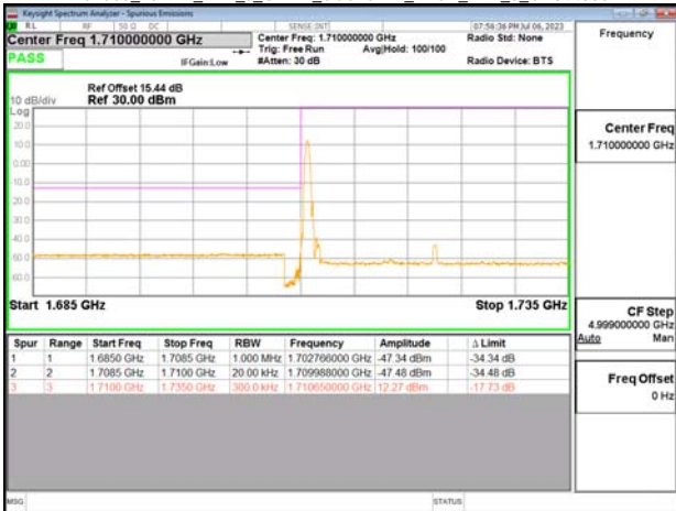
Band66_25MHz_DFT_s_OFDM_SCS15kHz_BPSK_RB1_132_CH353500
