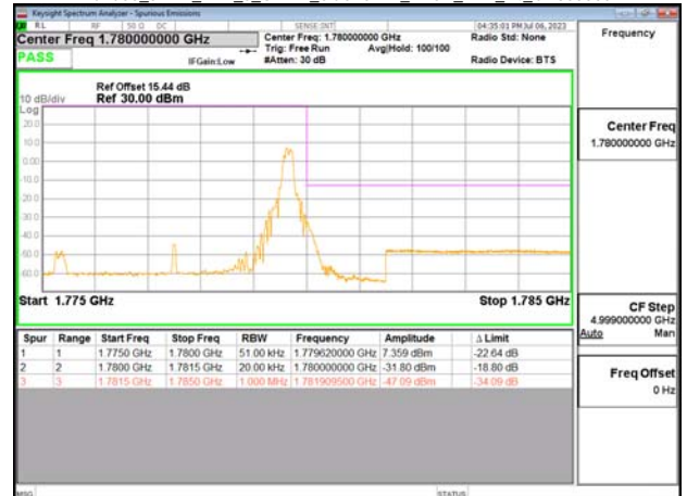
Band66_5MHz_DFT_s_OFDM_SCS15kHz_BPSK_RB1_24_CH355500
