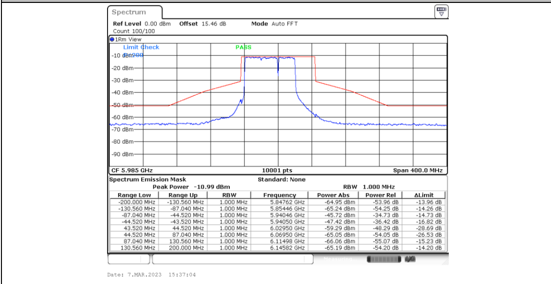
11BE80MIMO_Ant4_5985_Large RU 484+242_2
