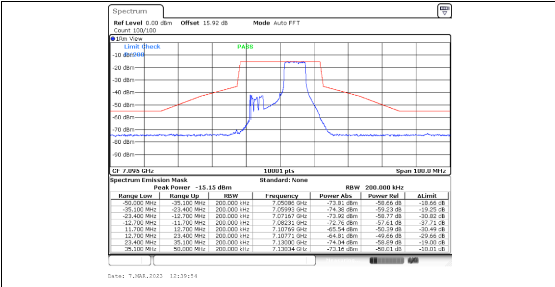
11BE20MIMO_Ant4_7095_106+26_OFDMA_2
