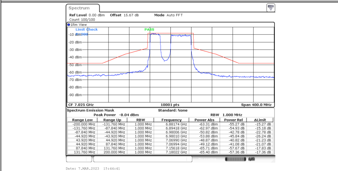
11BE80MIMO_Ant5_7025_Puncturing 20M_3
