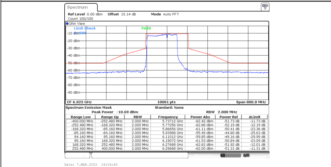
11BE160MIMO_Ant5_6025_Puncturing 20M_1
