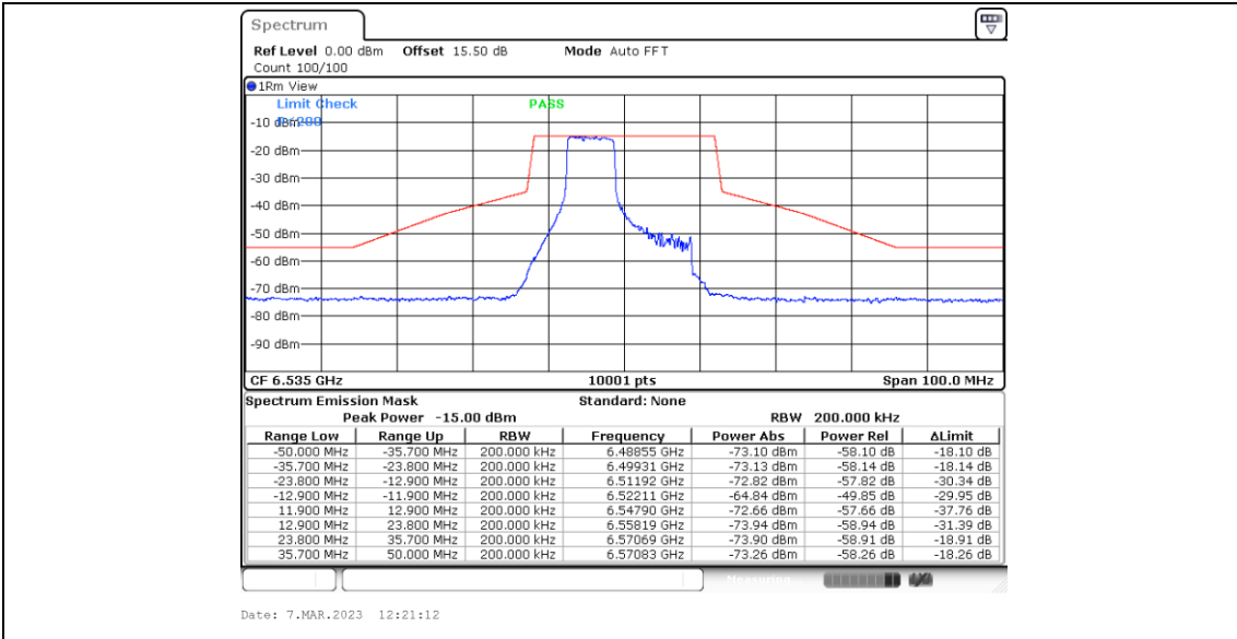
11BE20MIMO_Ant4_6535_106+26_OFDMA_1
