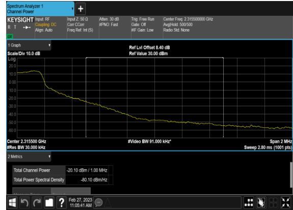
N30(10M)_DFT-s-OFDM_BPSK_Edge_1RB_Right_ Low_CH_CHP_PASS
