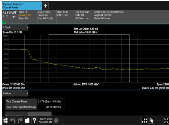
N30(5M)_DFT-s-OFDM_QPSK_Outer_Full_Low_
