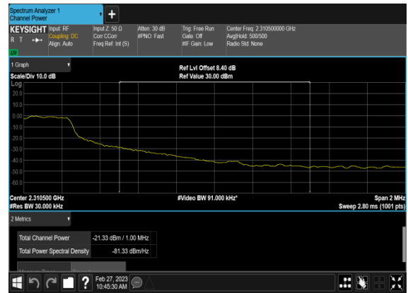
N30(5M)_DFT-s-OFDM_BPSK_Edge_1RB_Right_High
