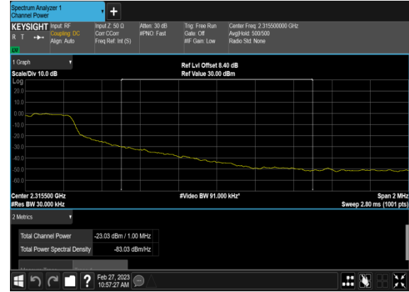
N30(5M)_DFT-s-OFDM_QPSK_Outer_Full_High_CH_ CHP_PASS
