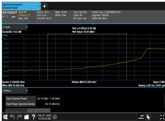
N30(5M)_DFT-s-OFDM_BPSK_Edge_1RB_Right
