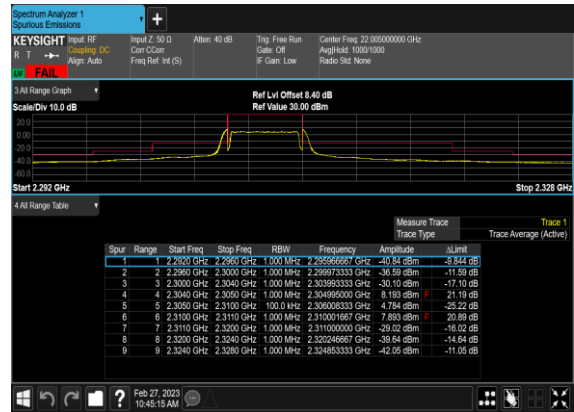
N30(5M)_DFT-s-OFDM_QPSK_Outer_Full_Low_CH
