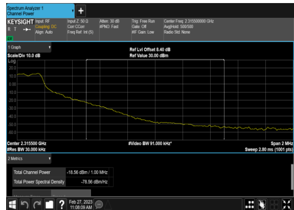
N30(10M)_DFT-s-OFDM_QPSK_Edge_1RB_Right_ Low_CH_CHP_PASS
