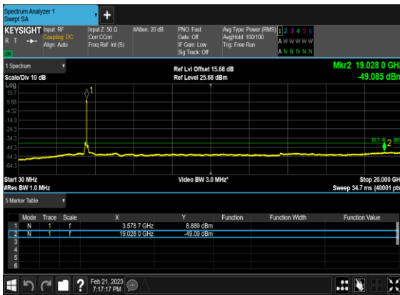
N48(40M)_DFT-s-OFDM_QPSK_Outer_Full_Low_CH
