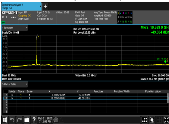
N48(40M)_DFT-s-OFDM_BPSK_Edge_1RB_Right_Low_CH
