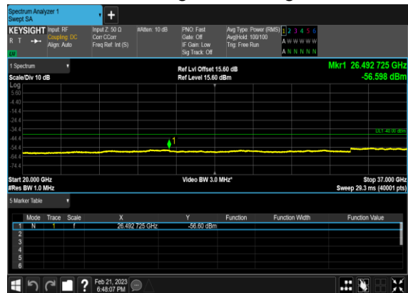
N48(20M)_DFT-s-OFDM_BPSK_Edge_1RB_Right_Low_CH
