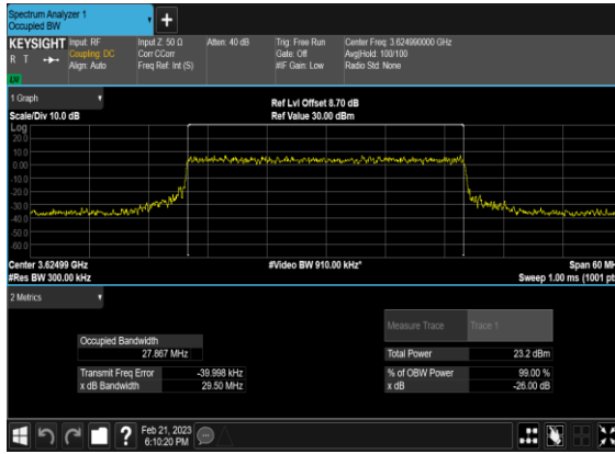
N48(30M)_CP-OFDM_QPSK_Outer_Full_Mid_CH
