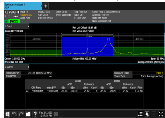
N48(10M)_DFT-s-OFDM_QPSK_Edge_1RB_Right_Low_CH
