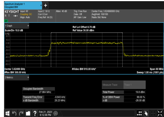
N48(30M)_CP-OFDM_256QAM_Outer_Full_Mid_CH
