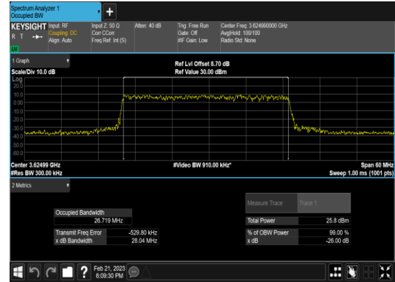
N48(30M)_DFT-s-OFDM_QPSK_Outer_Full_Mid_CH
