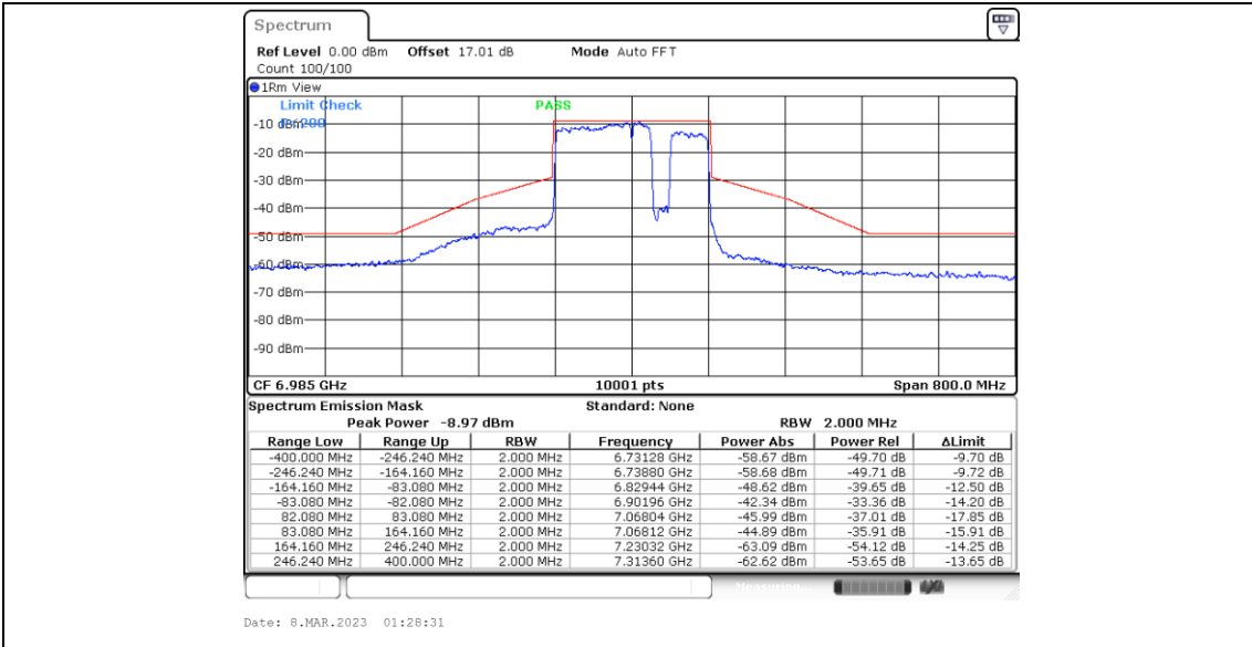
11BE160MIMO_Ant6_6985_Puncturing 20M_8
