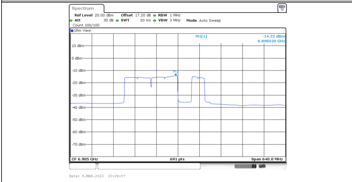
11BE320MIMO_Ant5_6905_Puncturing 80M+40M_8
