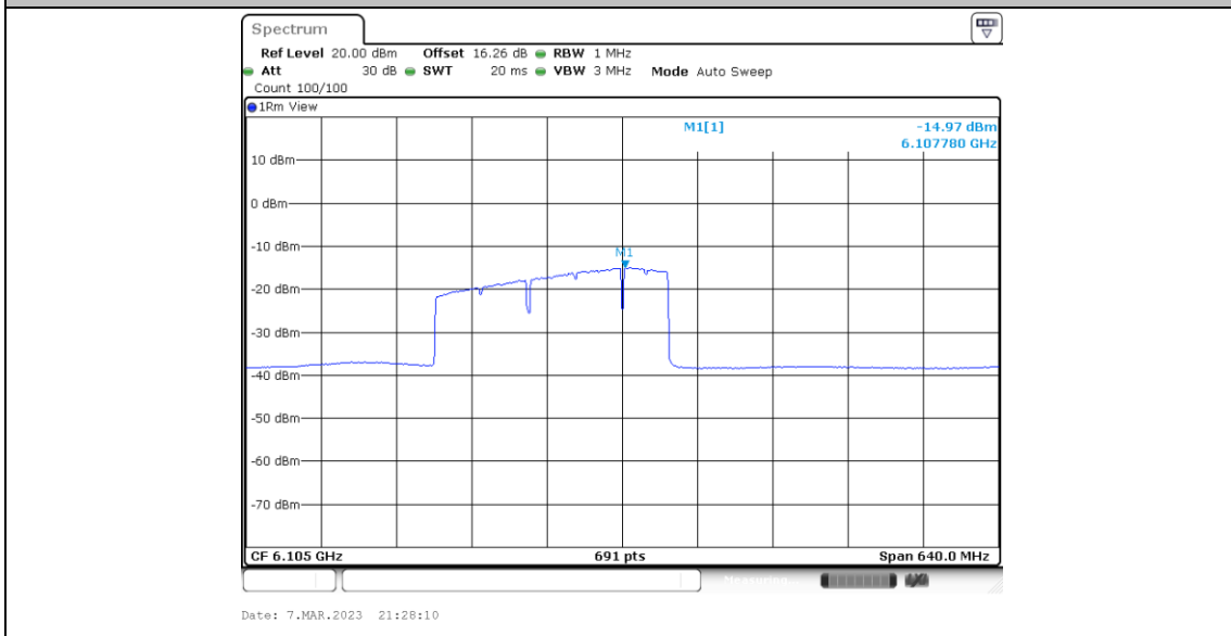
11BE320MIMO_Ant5_6105_Large RU 996*3_4
