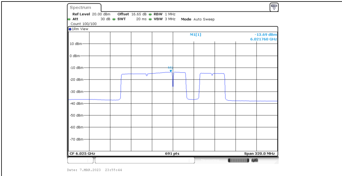
11BE160MIMO_Ant6_6025_Puncturing 20M_8
