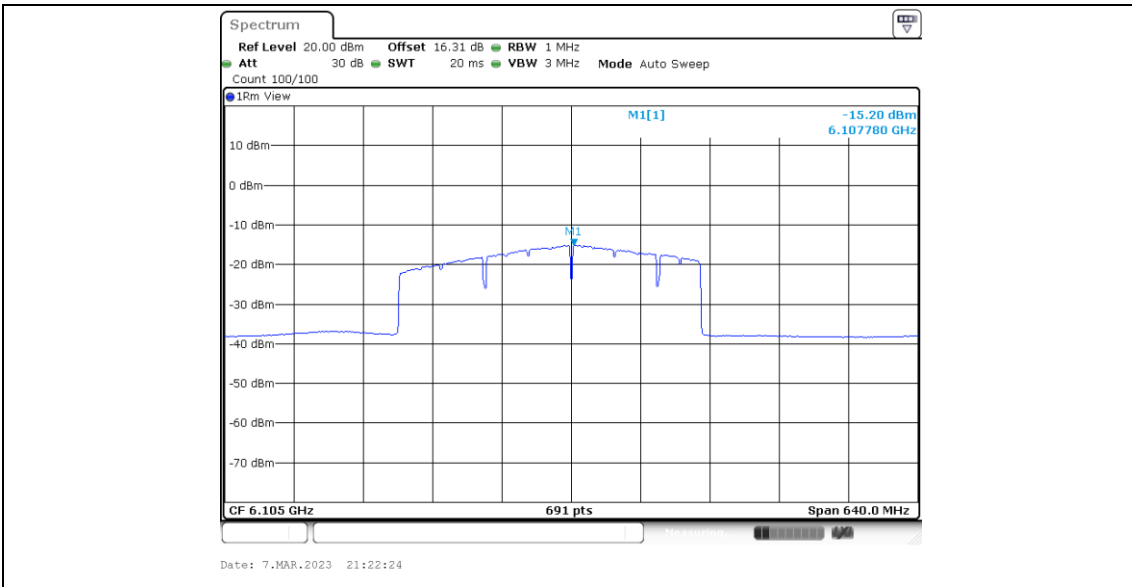
11BE320MIMO_Ant5_6105_Puncturing 80M+40M_1
