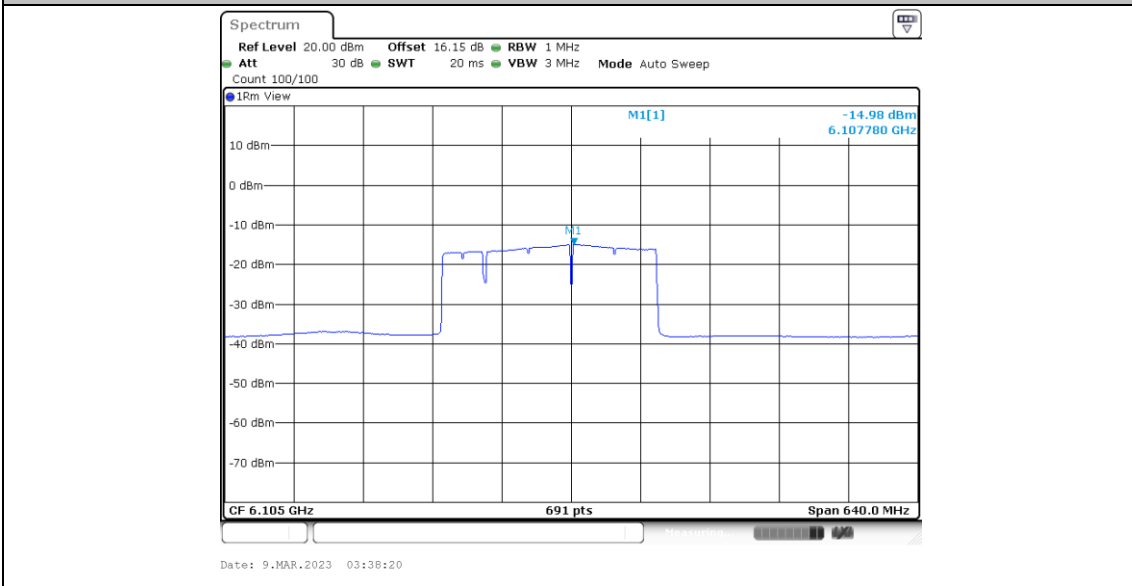
11BE320MIMO_Ant5_6105_Puncturing 80M+40M_3
