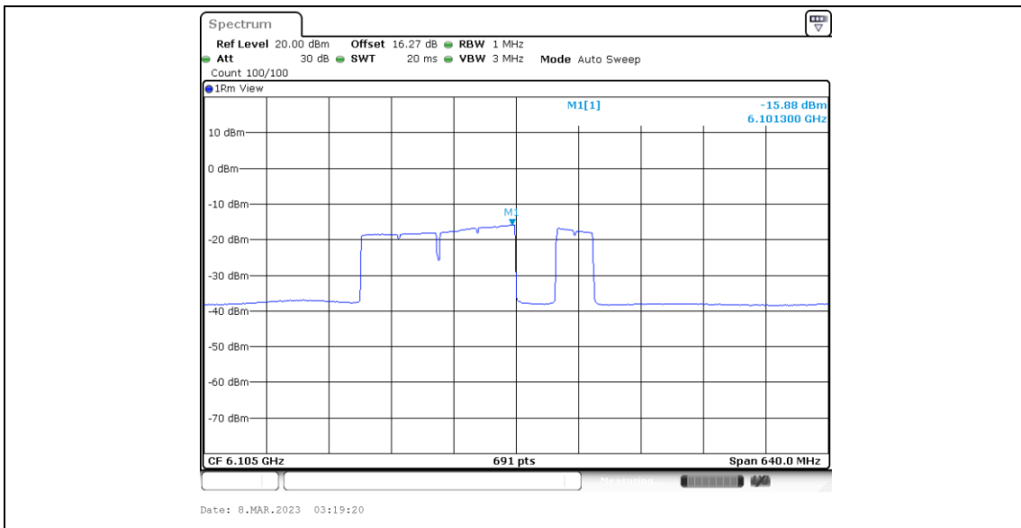
11BE320MIMO_Ant6_6105_Puncturing 80M+40M_8
