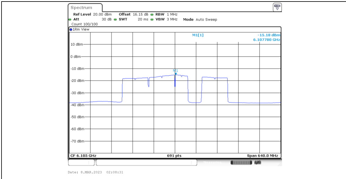
11BE320MIMO_Ant5_6105_Puncturing 40M_7
