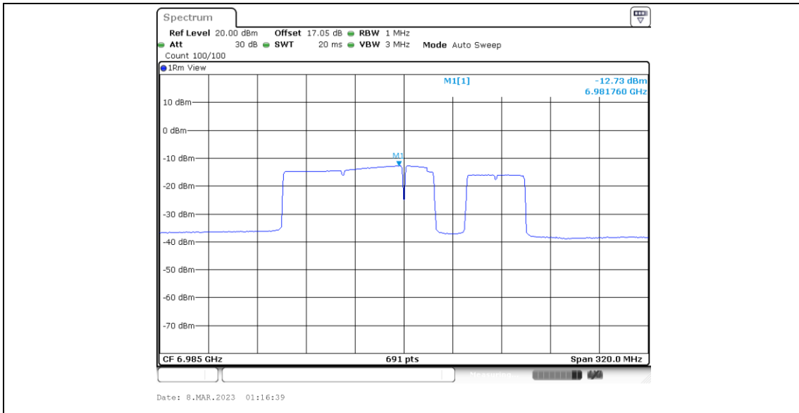
11BE160MIMO_Ant6_6985_Puncturing 20M_8
