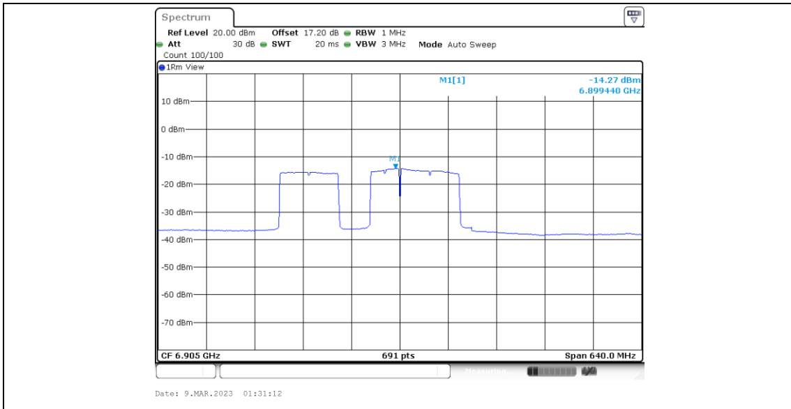
11BE320MIMO_Ant5_6905_Puncturing 80M+40M_5
