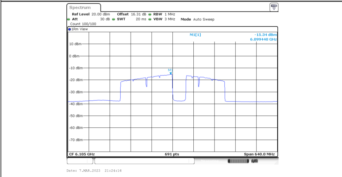
11BE320MIMO_Ant5_6105_Large RU 996*3+484_8
