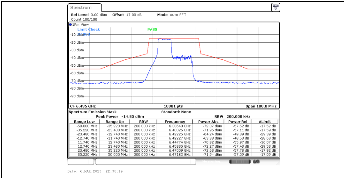
11BE20MIMO_Ant6_6435_106+26_OFDMA_1
