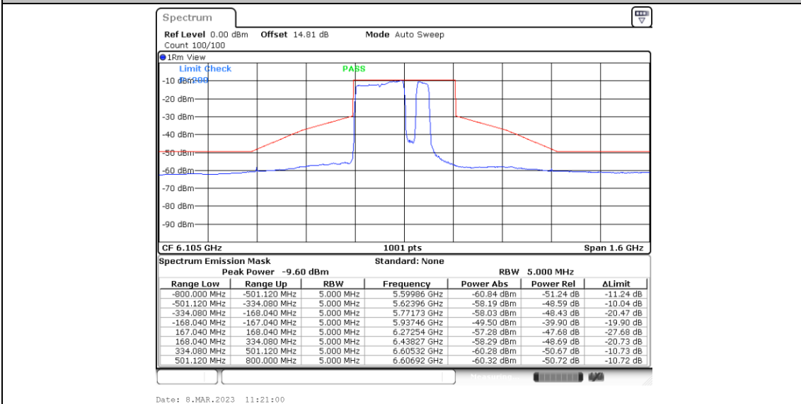
11BE320MIMO_Ant5_6105_Puncturing 80M+40M_8
