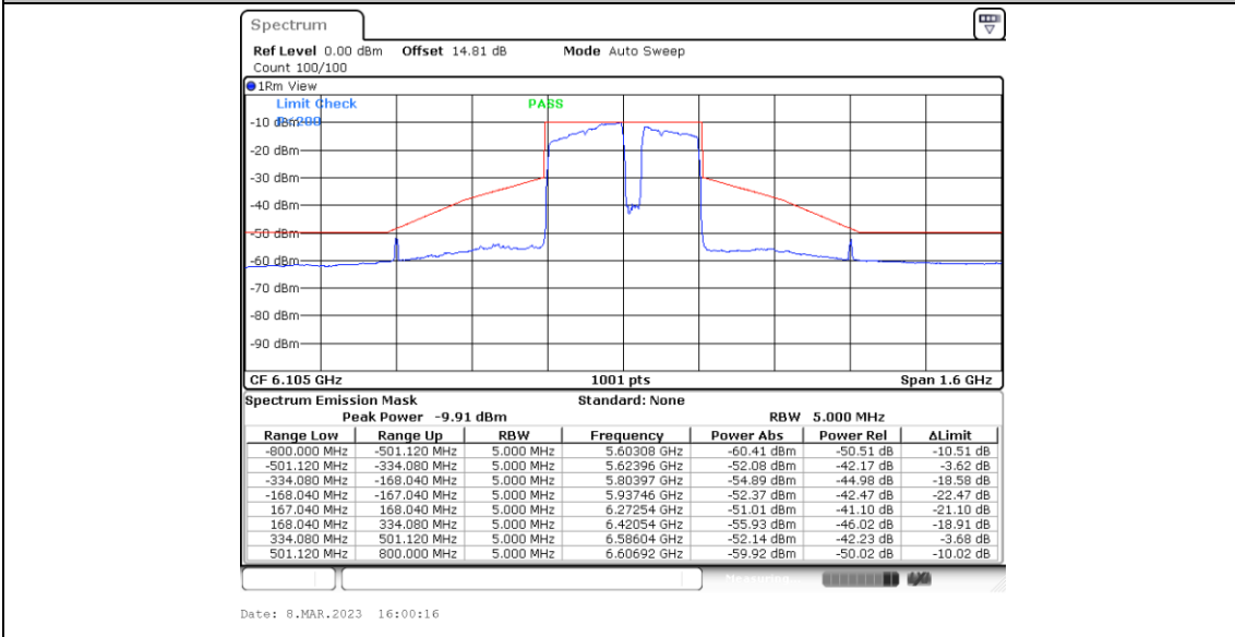
11BE320MIMO_Ant5_6105_Large RU 996*3+484_8
