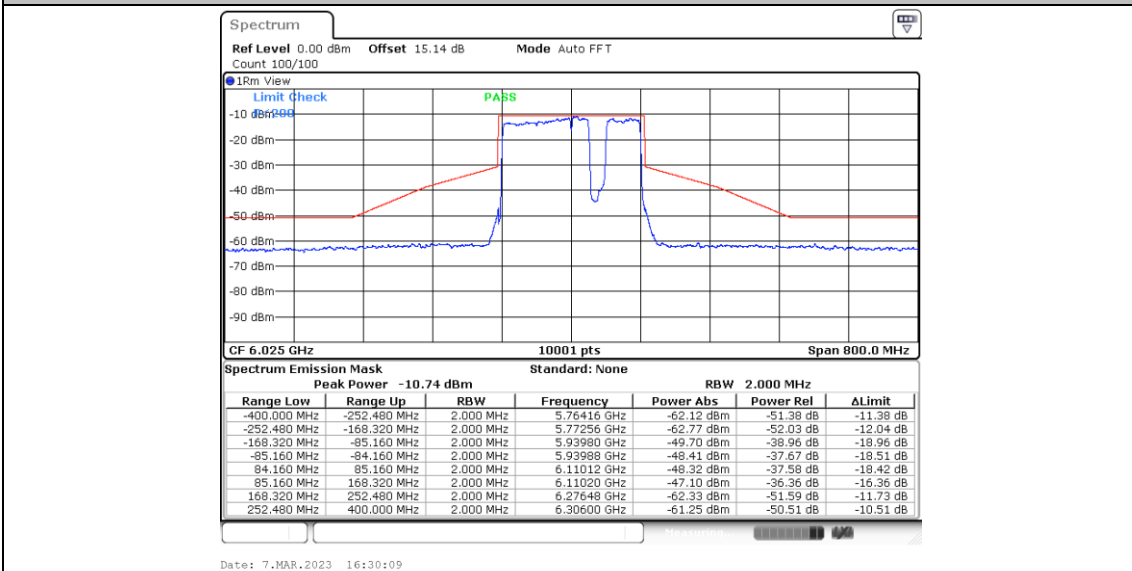
11BE160MIMO_Ant5_6025_Puncturing 20M_8
