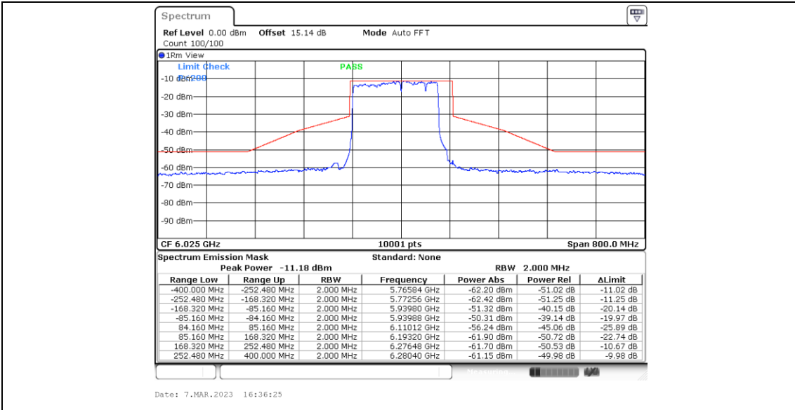
11BE160MIMO_Ant4_6025_Large RU 996+484_3
