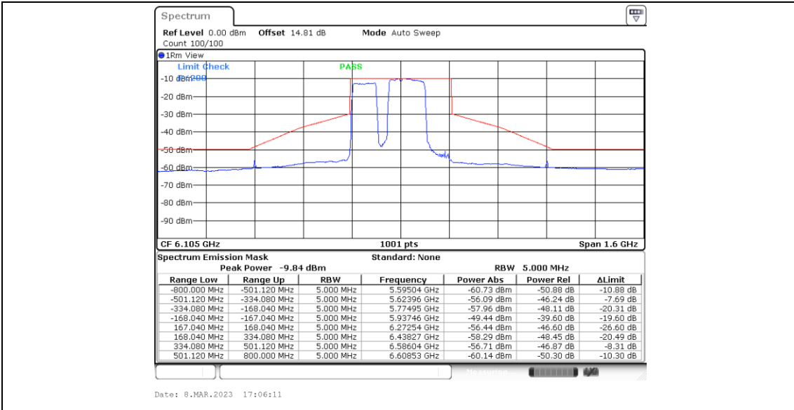
11BE320MIMO_Ant5_6105_Large RU 996*2+484_6
