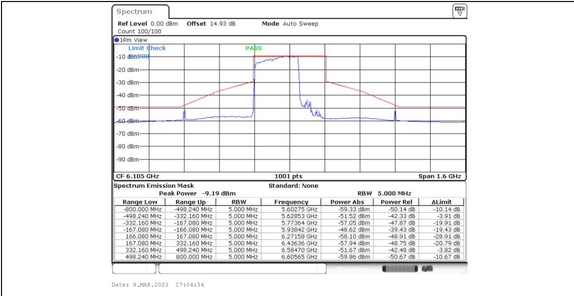
11BE320MIMO_Ant4_6105_Large RU 996*3_4
