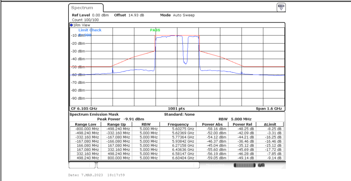
11BE320MIMO_Ant4_6105_Puncturing 40M_7
