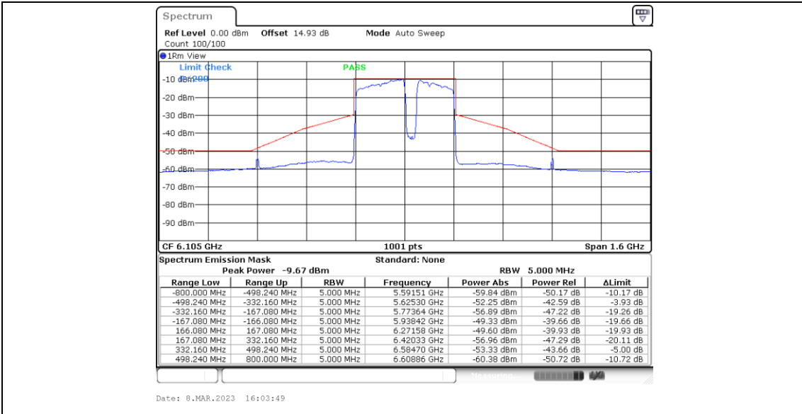
11BE320MIMO_Ant4_6105_Large RU 996*3+484_8
