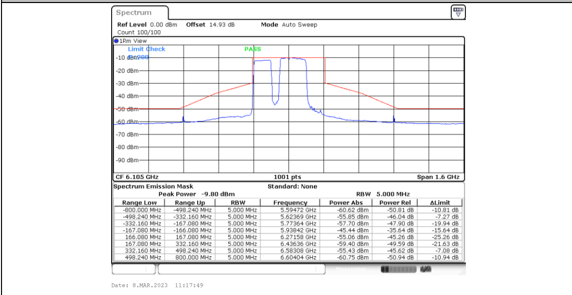
11BE320MIMO_Ant4_6105_Puncturing 80M+40M_5
