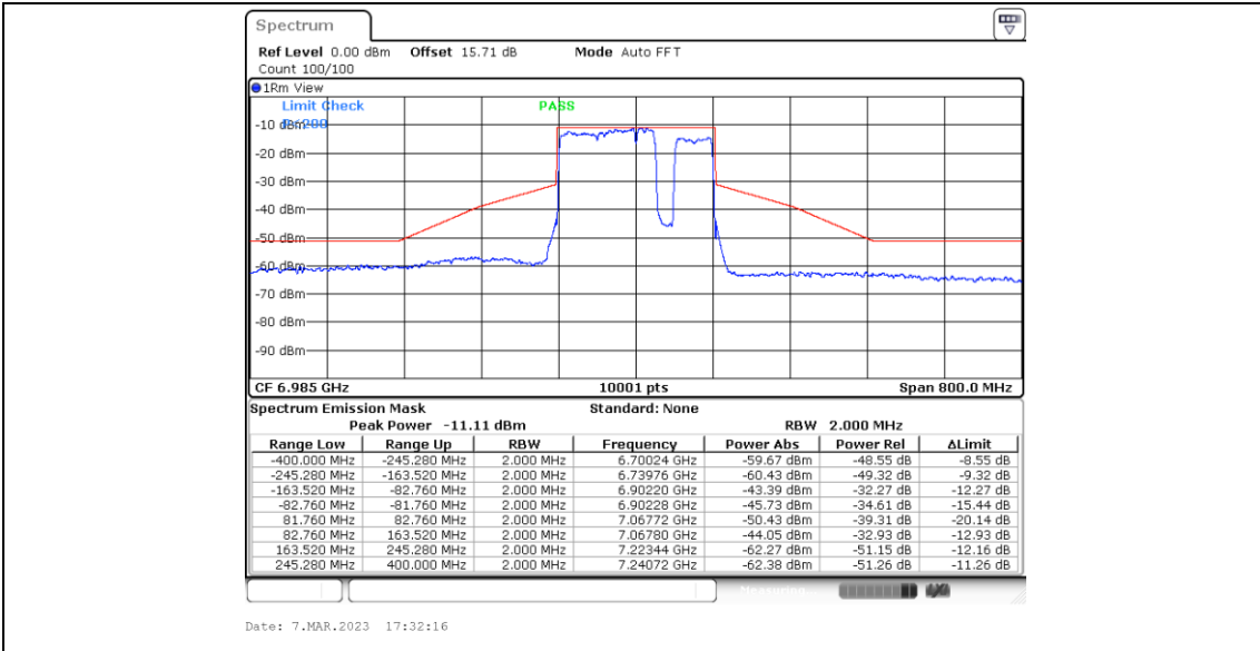
11BE160MIMO_Ant4_6985_Puncturing 20M_8
