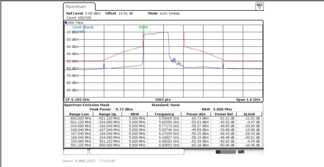
11BE320MIMO_Ant5_6105_Large RU 996*3_4
