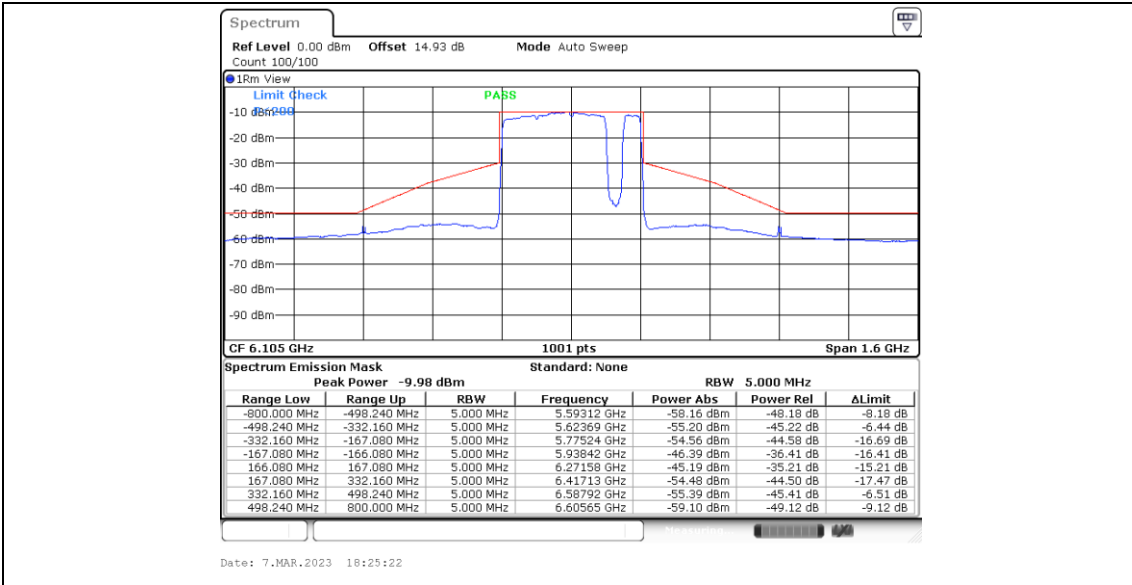
11BE320MIMO_Ant4_6105_Puncturing 40M_8
