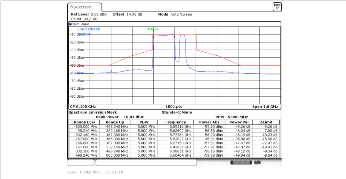
11BE320MIMO_Ant4_6105_Puncturing 80M+40M_8
