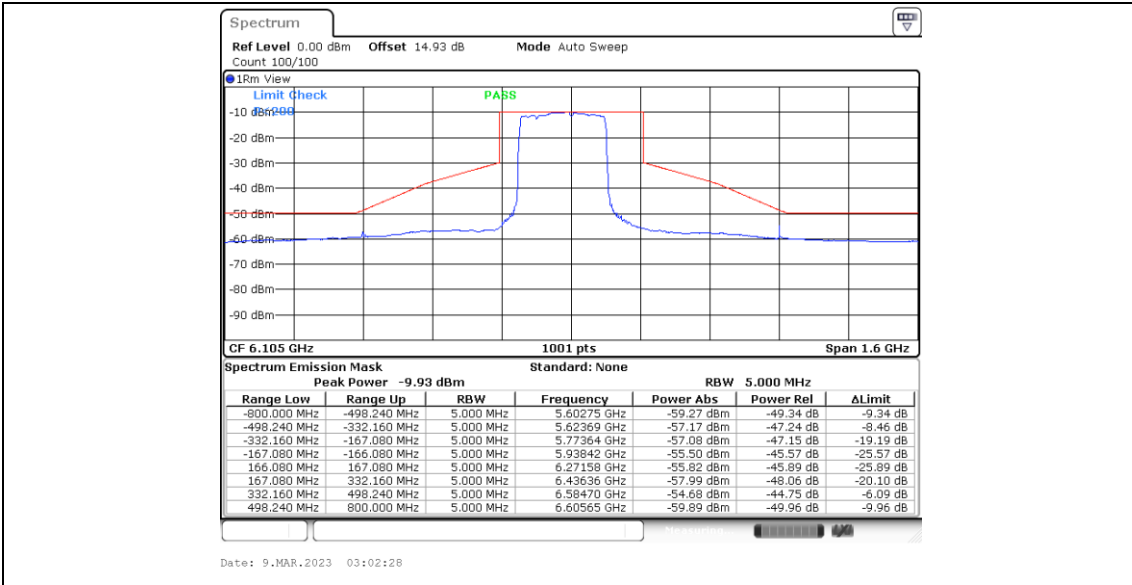
11BE320MIMO_Ant4_6105_Puncturing 80M+40M_3
