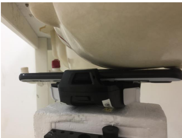
Left Cheek with AeroActive cooler, Test Separation 0 mm
