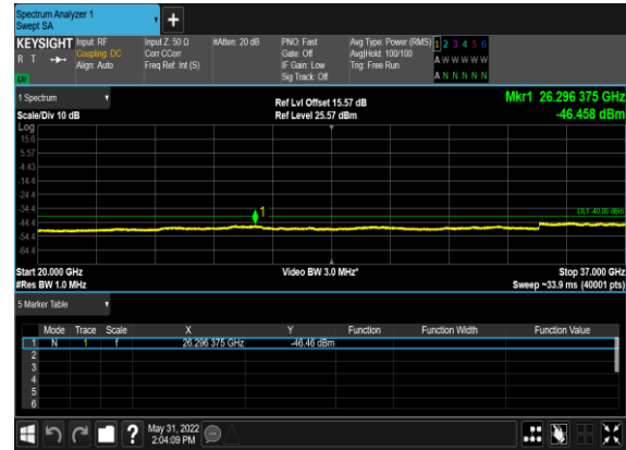
N48(10M)_DFT-s- OFDM_BPSK_Outer_Full_High_CH
