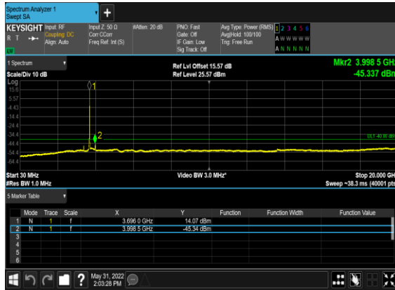
N48(10M)_DFT-s- OFDM_BPSK_Outer_Full_High_CH
