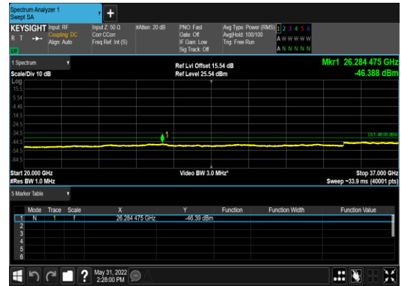
N48(20M)_DFT-s- OFDM_QPSK_Edge_1RB_Right_High_CH
