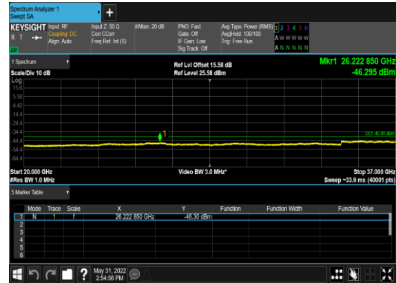
N48(40M)_DFT-s- OFDM_BPSK_Outer_Full_High_CH
