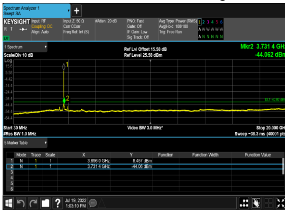
N48(20M)_DFT-s- OFDM_QPSK_Outer_Full_High_CH
