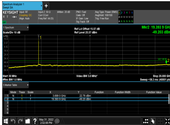
N48(10M)_DFT-s- OFDM_QPSK_Edge_1RB_Right_High_CH
