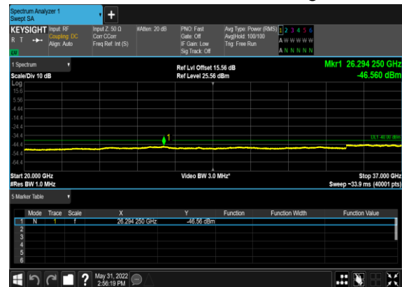
N48(40M)_DFT-s- OFDM_QPSK_Outer_Full_High_CH
