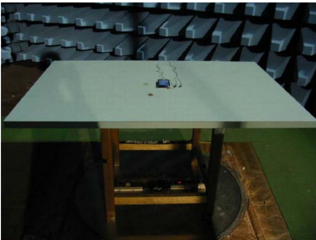
Front View of the Test Configuration of X-axis
