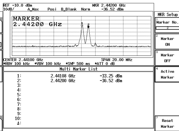
Channel 39 2441MHz
