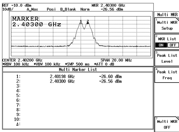
Channel 00 2402MHz
