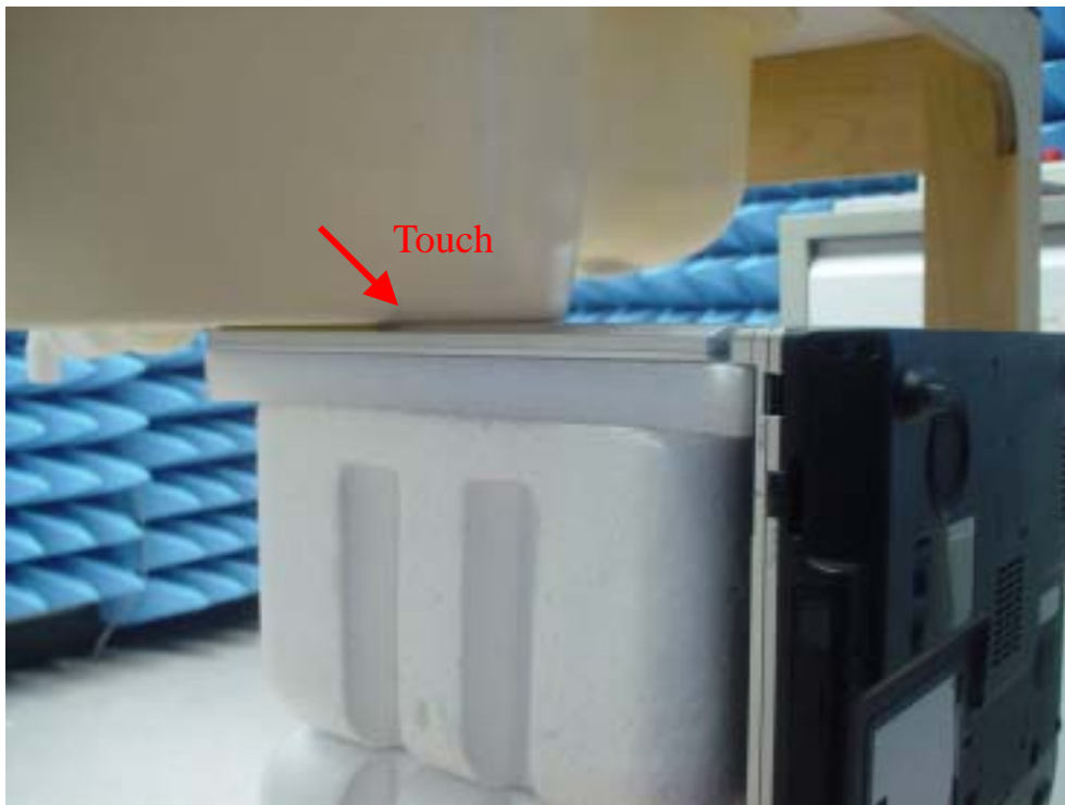
Fig.3 Photograph of the back of the LCD Panel of Right Antenna contact to the flat phantom; and at a distance of 0.0 cm from the base of the phantom
