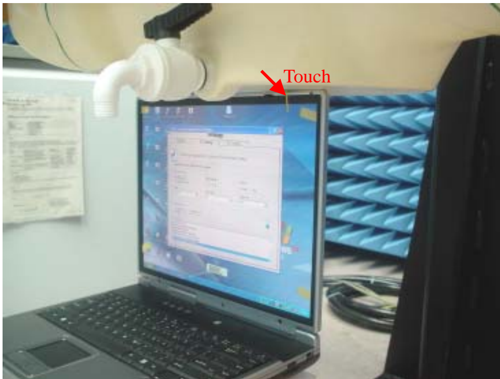
Fig.2 Photograph of the top of the LCD panel of Main Antenna contact to the flat Phantom; and at a distance of 0.0 cm from the base of the phantom.
