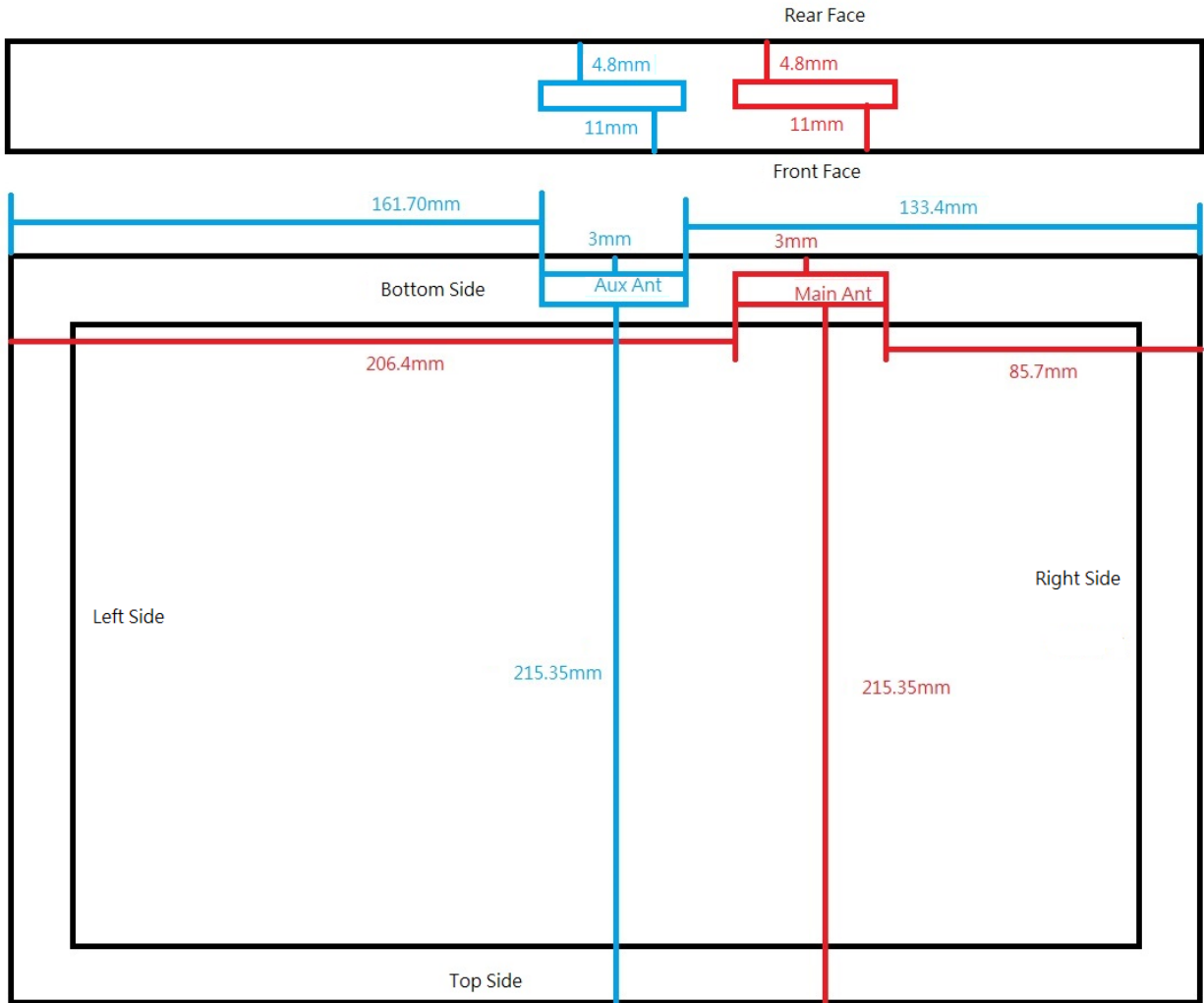
Fig 7.2.3: Antenna to the edge for PAD Mode (Rear View)
