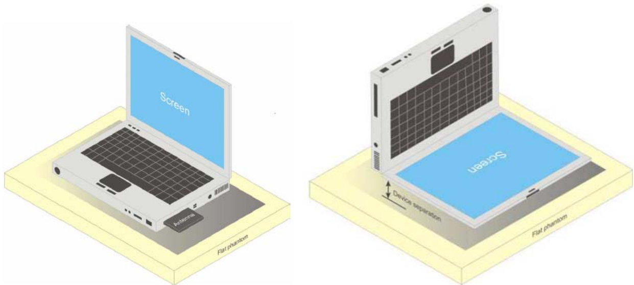
Fig 7.2.1: Test setup for NB mode
