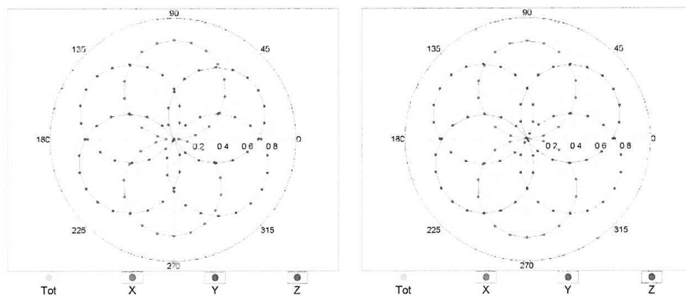
f=600 MHz,TEM
