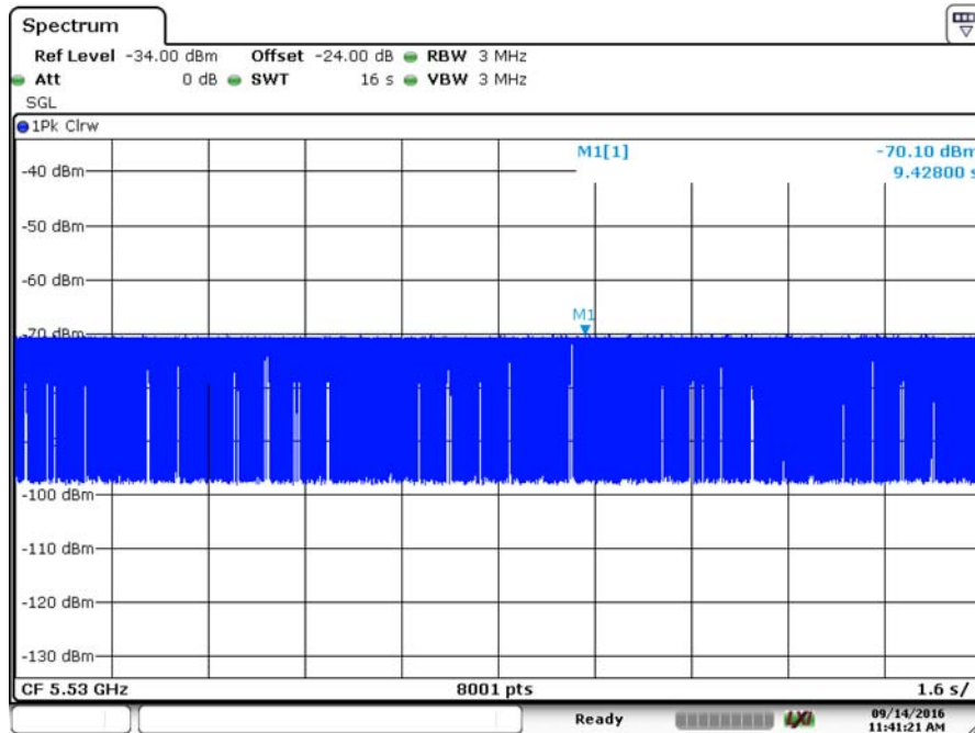
Plot of Slave Traffic at 5530MHz
