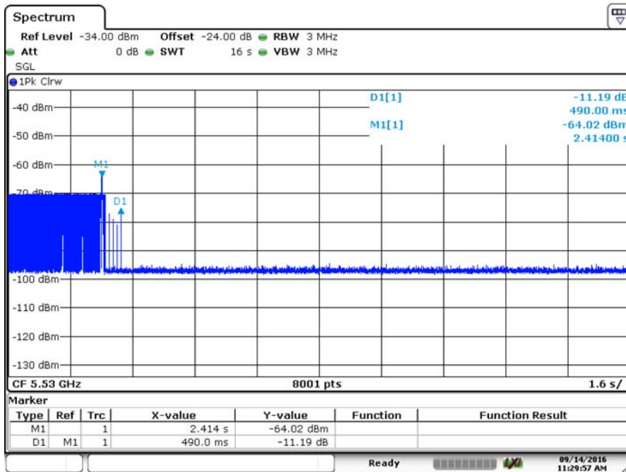
Channel Move Time for Radar Test Type 0 at 5530MHz
