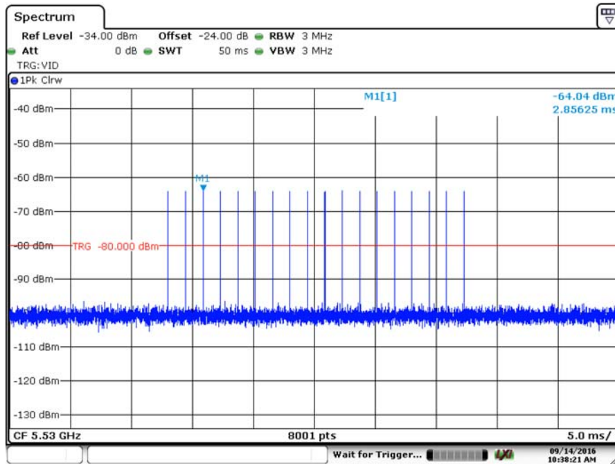
Radar Type 0 Calibration Plot (5530MHz)
