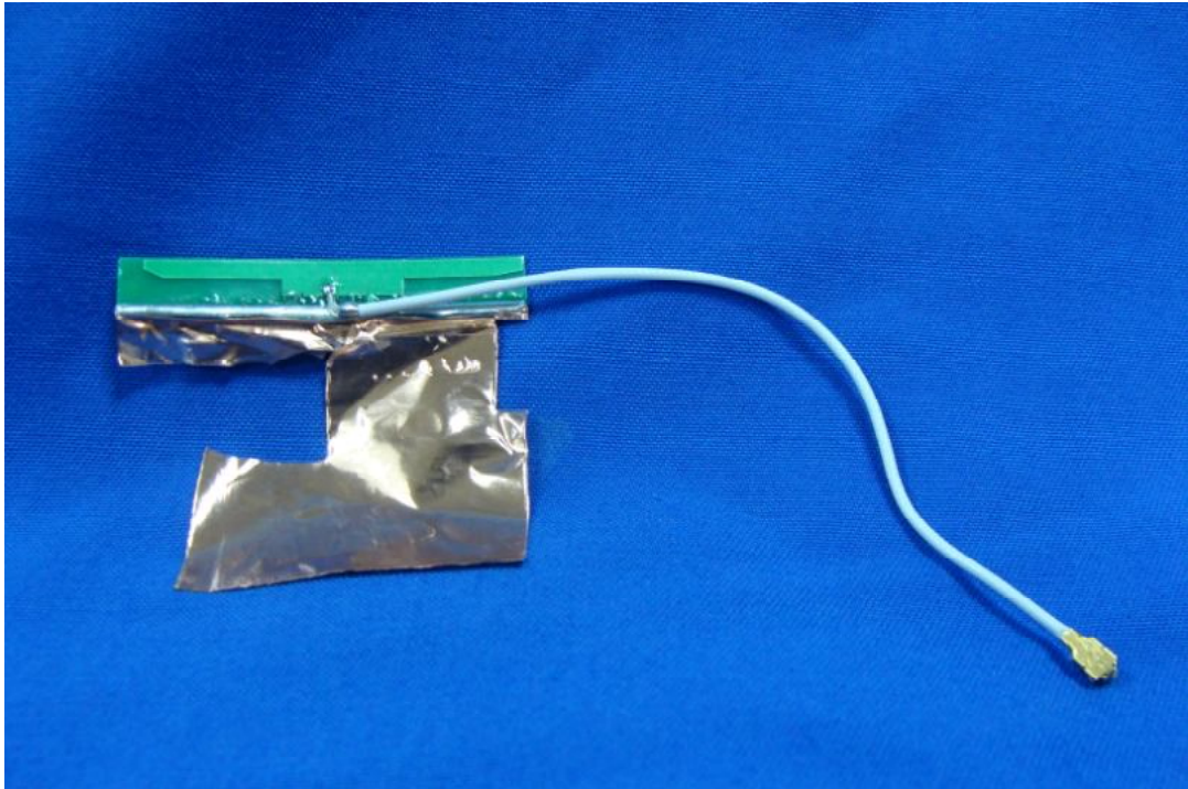
(19) EUT Photo (INPAQ Antenna-Aux)
