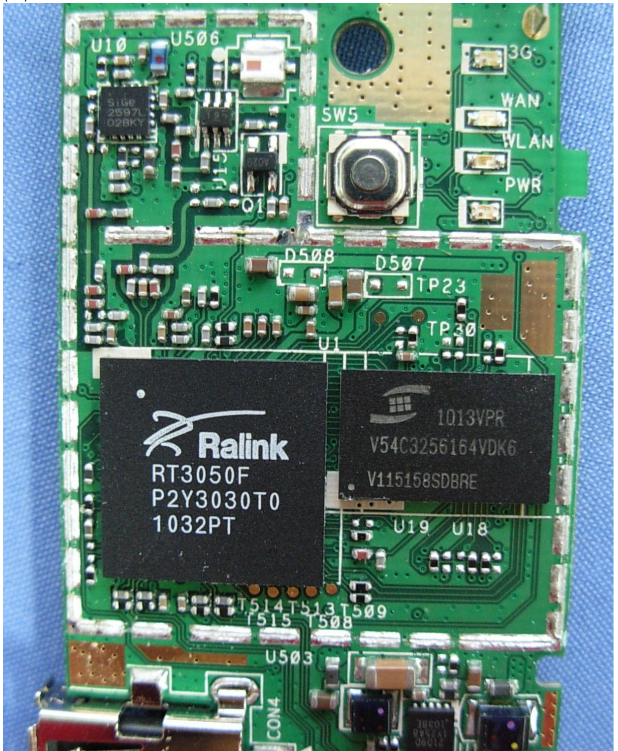
(26) EUT Photo
