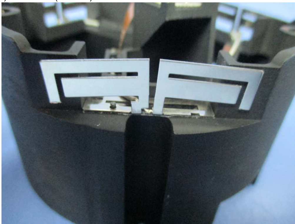
(45) EUT Photo (Antenna)
