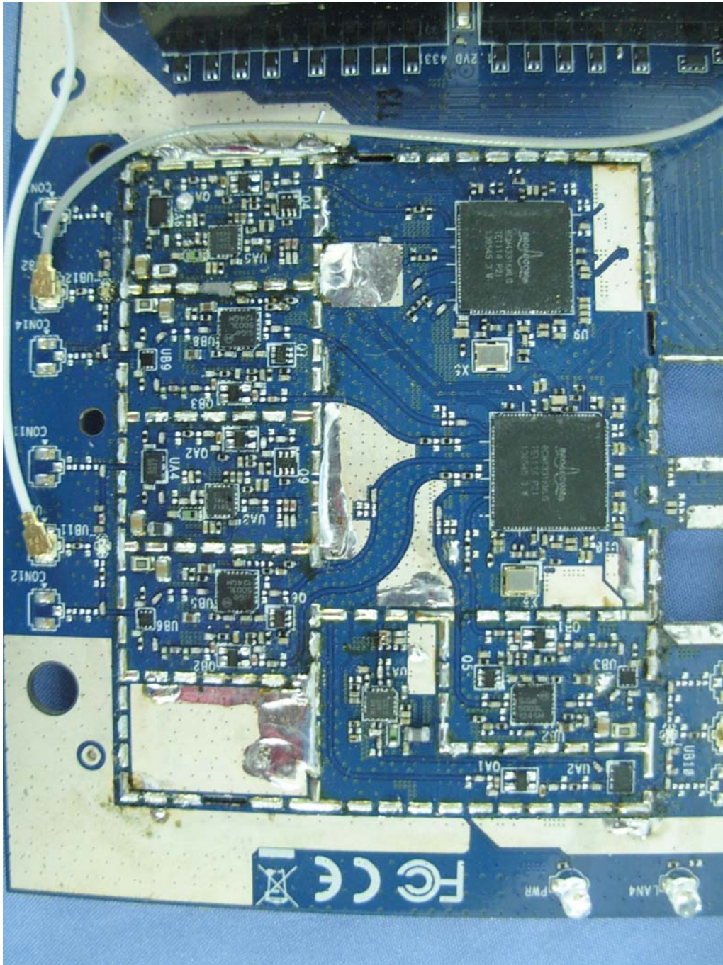
(11) EUT Photo
