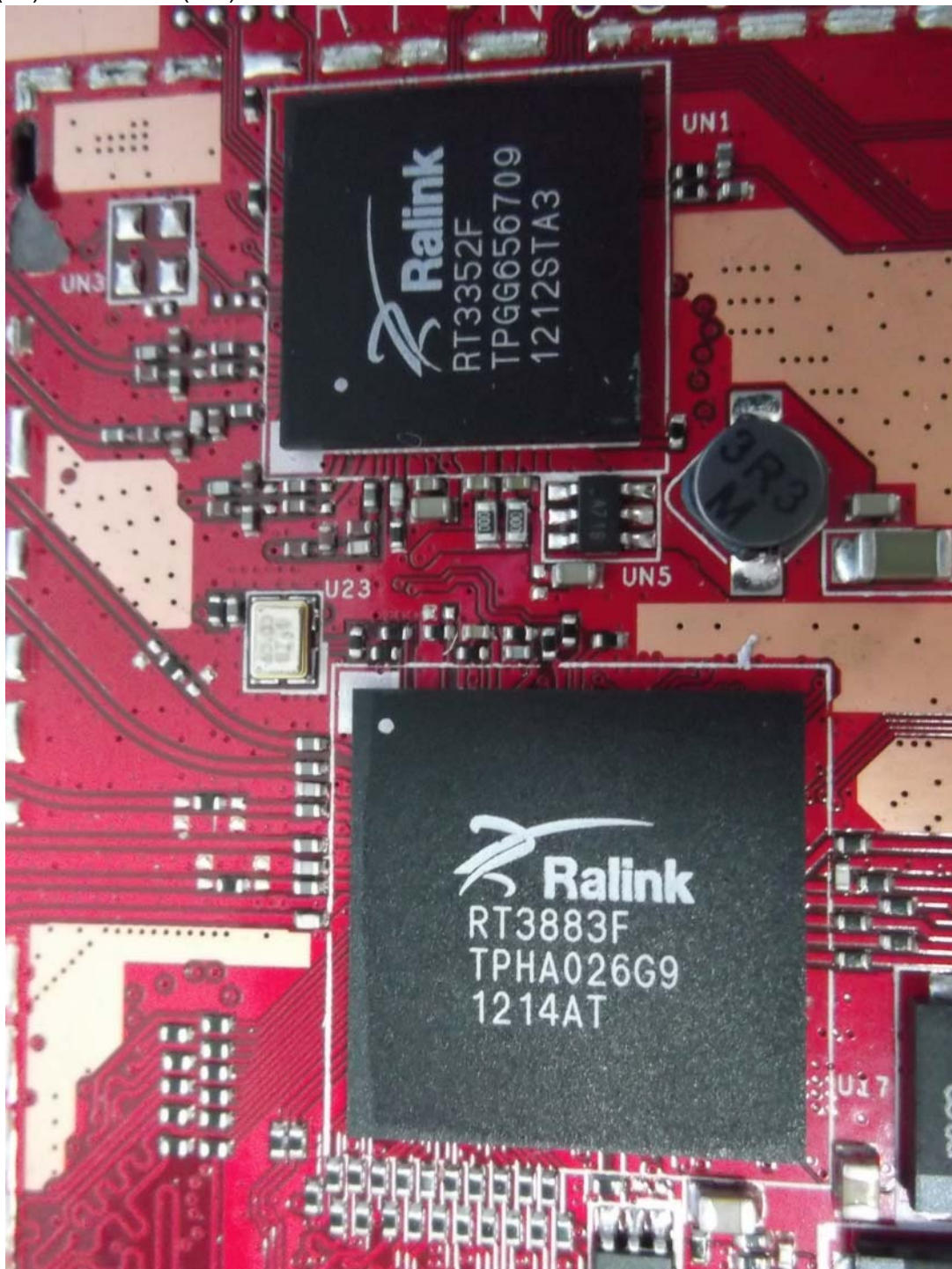
(23) EUT Photo (MB)
