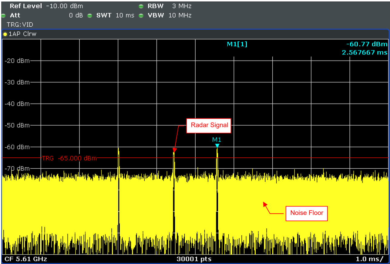
Single Burst of Radar Signal 5
