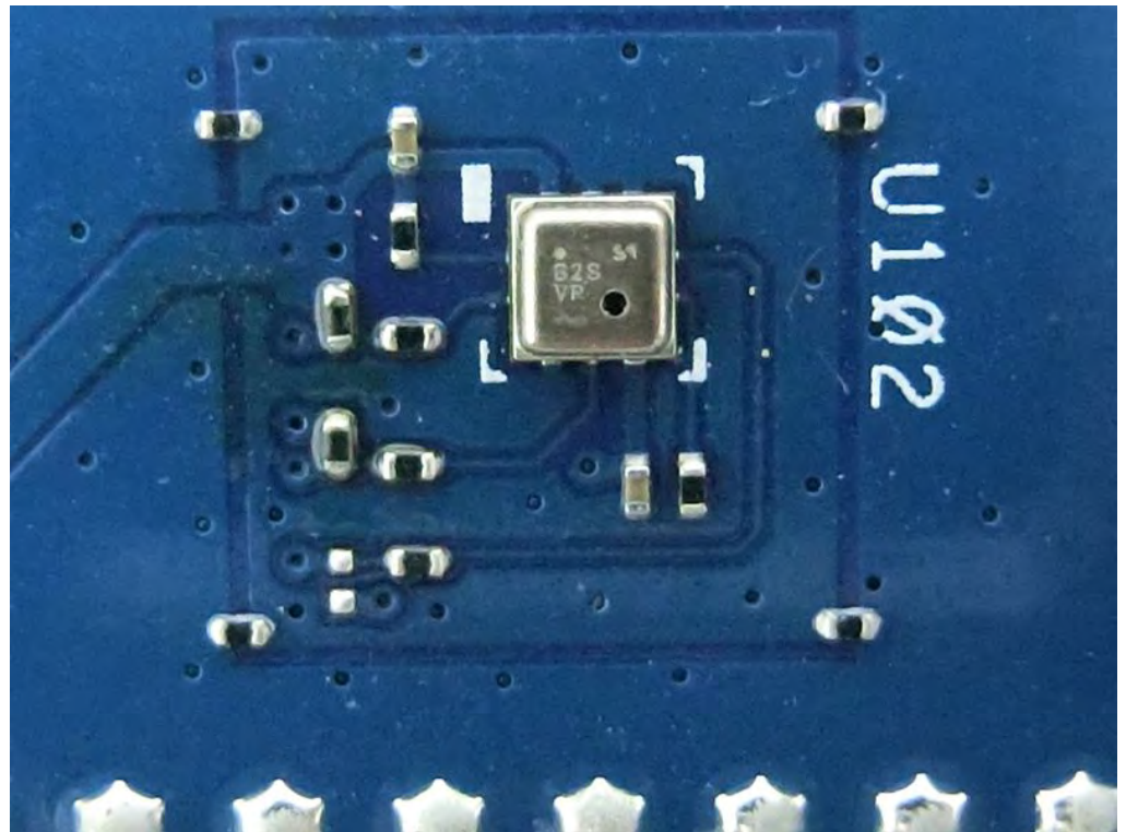
Barometric pressure sensor (Location: U102)
