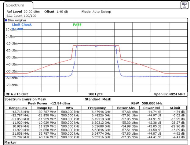
802.11ax (20MHz) 6515MHz Chain B NSS-2
